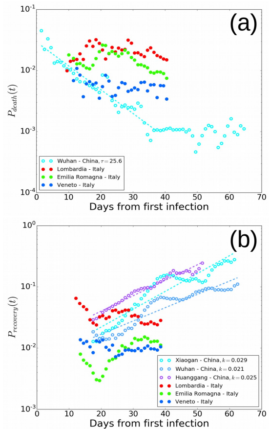
FIG. 4: Death and recovery rates. (a) The death rate in Wuhan shows an exponential decay similar to the infection rate (other cities show poor statistics). The characteristic decay time \tau is about twice time longer for the death rate than the infection rate. Provinces in Italy with most cases do not show a decay suggesting an overload of the health system. (b) The recovery rate in China shows an approximate exponential growth as the disease is getting controlled, Eq. (13). The growth parameter k characterizes the health system efficiency. Provinces in Italy with most recovery cases do not show growth and remain approximately constant suggesting an overload of the health system as suggested by the death rate.
