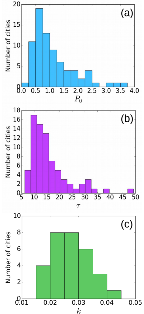
FIG. 5: Statistical properties of the temporal behaviour of city in China (a) The constant infection rate, P_0 is mostly range 0.5-2 while in a few cities it can be much larger. The average value is 1.16 with standard deviation 0.84. (b) The distribution of the exponent \tau characterizing the extinction of the disease which found to be in the range 5-50 days. The average value is 15.9 with standard deviation 7.7. Here we used latency period of 4 days. (c) The distribution of k characterizing the recovery rate and reflects the health system efficiency which found to be in the range 0.015-0.045. The average value is 0.027 with standard deviation 0.006.
