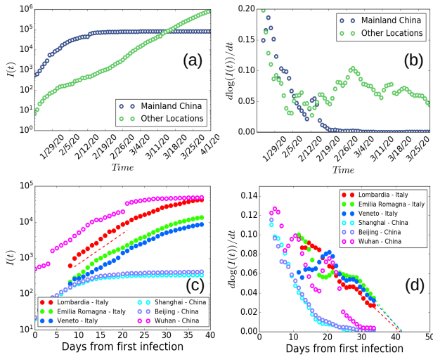
FIG. 1: General view of the COVID-19 propagation.
