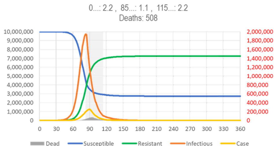
Fig 11: SIR Model of SARS, Window of Opportunity for Fast Eradication of the Epidemic. (see Fig 1 for legend). The gray area indicates the period where containment can give a “coup de grace” to a respiratory disease epidemic. The more narrow bell curve with a post-peak intervention indicates the reduction in number of infections and, thus, deaths. (spreadsheet for model calculations available from https://app.box.com/s/pa446z1csxcvfksgj13oohjm3bjg86q1 )
