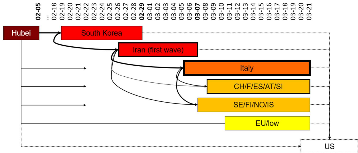
Fig 14: Hypothetical virus transmission pathways. Connection width: number of contacts, box colors: infectiousness, box borders: lethality, dotted connections/borders: unknown. The end date of a box indicates the date of peak incidence, if known (bold date).
