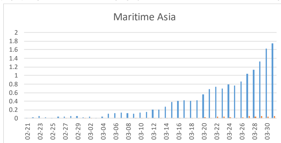
Fig 3: COVID-19 cases in Maritime Asia. See Fig 1 for legend.
