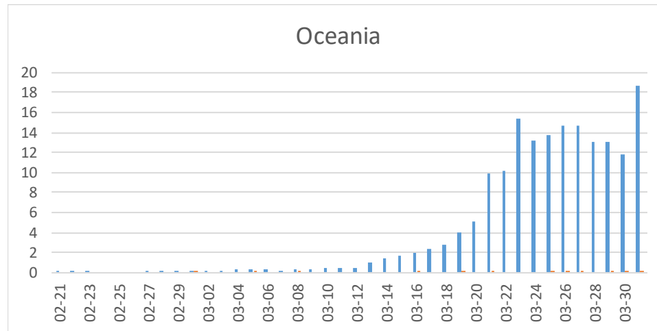
Fig 10: COVID-19 cases in the Oceania (Australia and New Zealand). See Fig 1 for legend..
