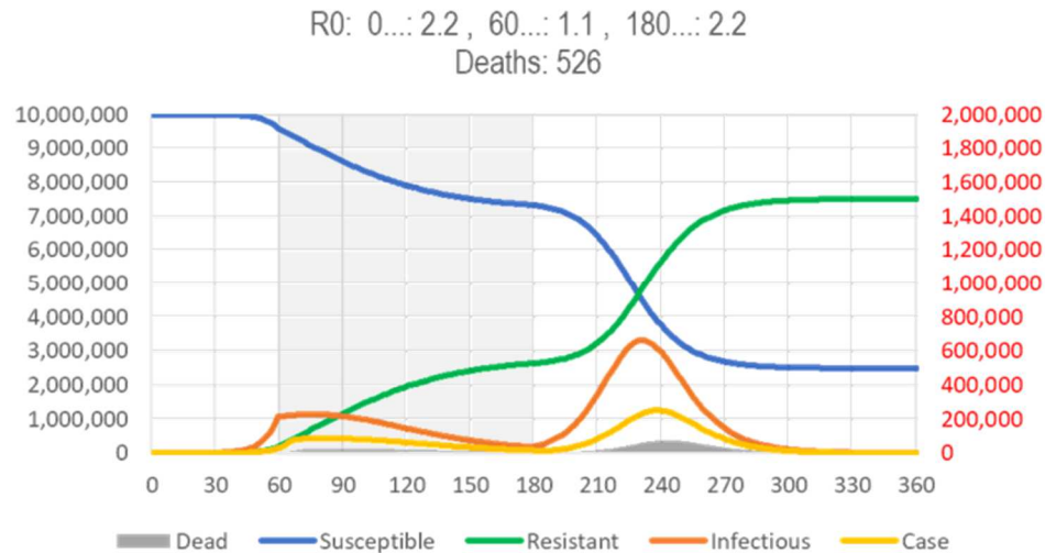
Fig 13: SIR Model of SARS, Effect of Early Social Distancing / Lockdown. (see Fig 1 for legend). It is assumed that a highly effective intervention reduces R_0 by 50% for 4 months, beginning after the appearance of a novel type of cases is noticed. The proportion of symptomatic cases (0.05%/d, i.e., .35% of infected people will become cases and the proportion of cases to die (2%) may change, but the issues discussed here are broadly independent of these assumptions. (spreadsheet for model calculations available from https://app.box.com/s/pa446z1csxcvfksgj13oohjm3bjg86ql )
