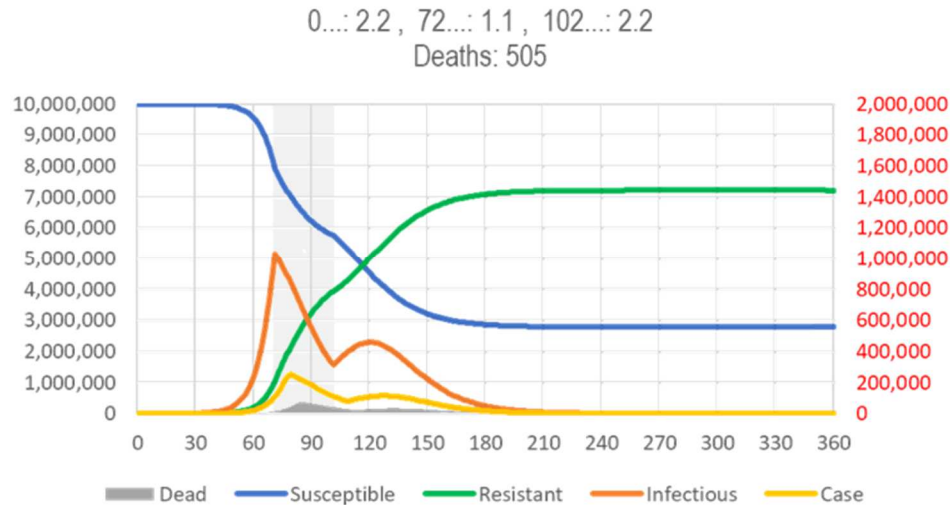
Fig 12: SIR Model of SARS, Window of Opportunity for Maximal Reduction of Total Deaths. (see Fig 1 for legend). The gray area indicates the period where containment can have the most impact on total number of deaths. However, the epidemic is not eradicated. (spreadsheet for model calculations available from https://app.box.com/s/pa446z1csxcvfksgj13oohjm3bjg86ql )
