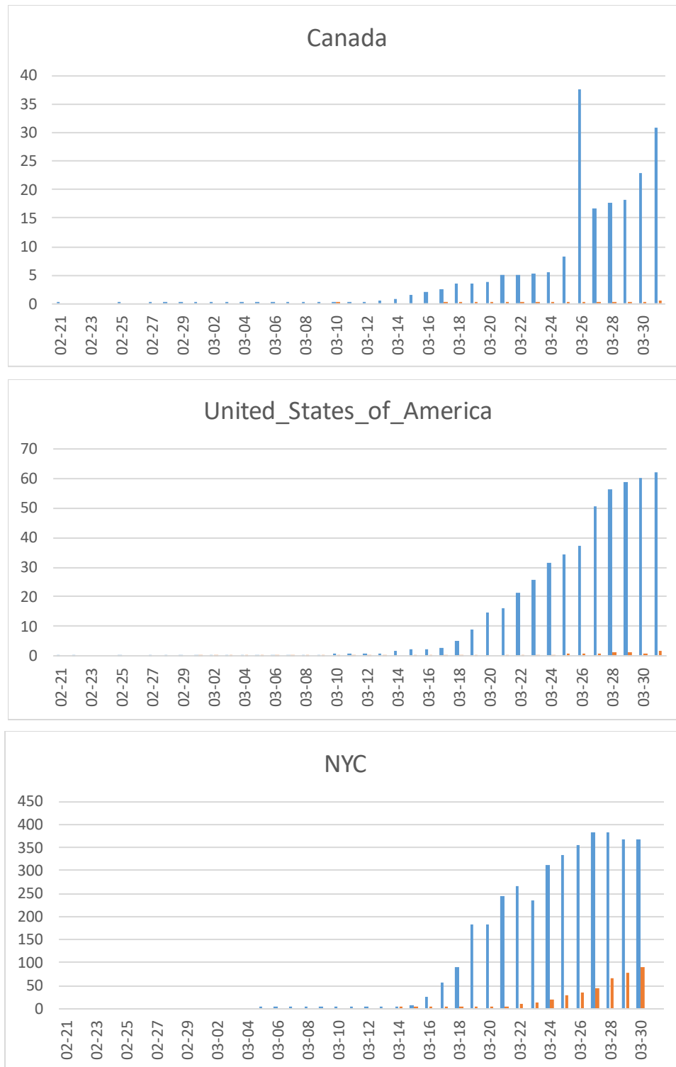
Fig 9: COVID-19 cases in the North America. See Fig 1 for legend. The high peak in the Canadian data on 03-26 cannot be reconciled with the dynamics of a respiratory disease spreading.
