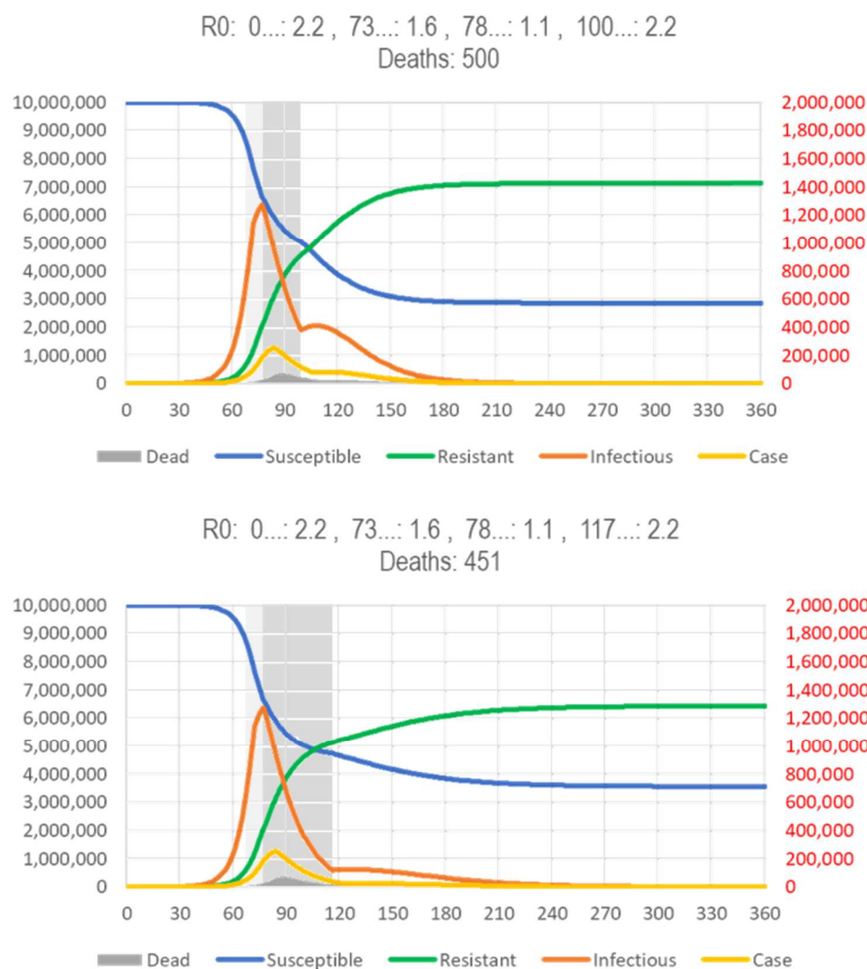
Fig 15: SIR Model of SARS, Phased in Restrictions. (see Fig 1 for legend). The gray areas indicate the periods of low (5 d) and high intensity (22/40 d) restrictions)
