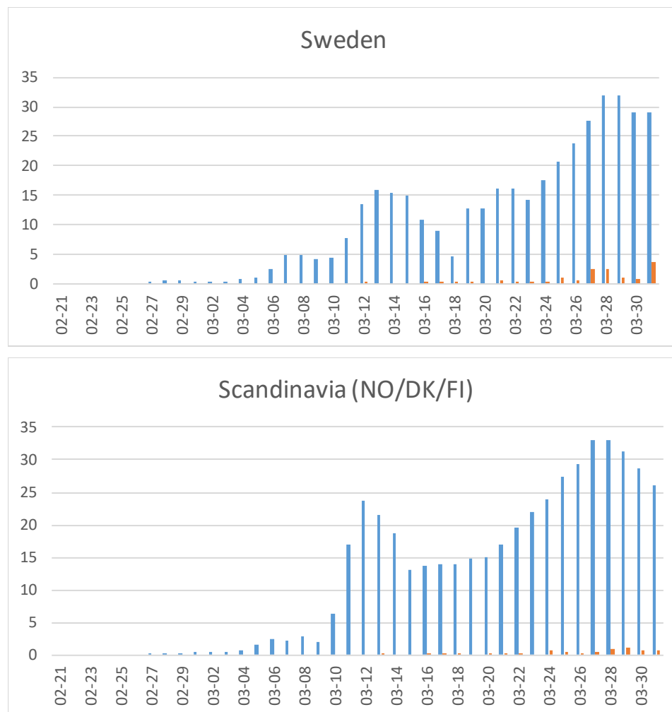
Fig 8: COVID-19 cases in the Scandinavia. See Fig 1 for legend.
