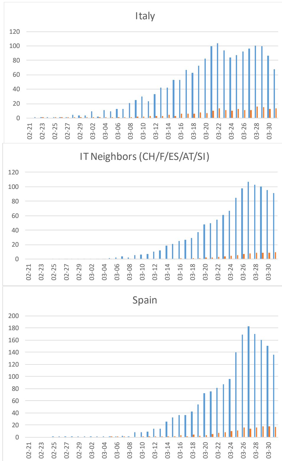
Fig 5: COVID-19 cases in Italy and its neighboring countries. Italy (top), European countries neighboring Italy (IT+, middle). Spain also shown separately. See Fig 1 for legend.
