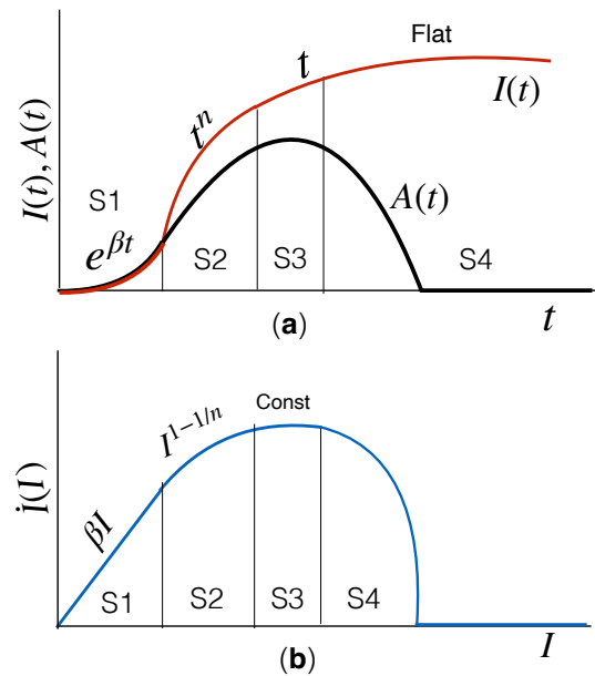
FIG. 3. (color online) For COVID-19 epidemic: (a) Schematic plots for the count of infected individuals, I(t) , and the count of active cases, A(t) , vs. time. (b) Schematic plot of the derivative \dot{I} vs. I . S1, S2, S3, S4 represent four stages of the epidemic: exponential growth in count ( \exp(\beta t) ), power law growth ( t^n ), linear growth ( t ), and flat. In stages S2, S3, S4, A(t) < I(t) due to recovery or death.
