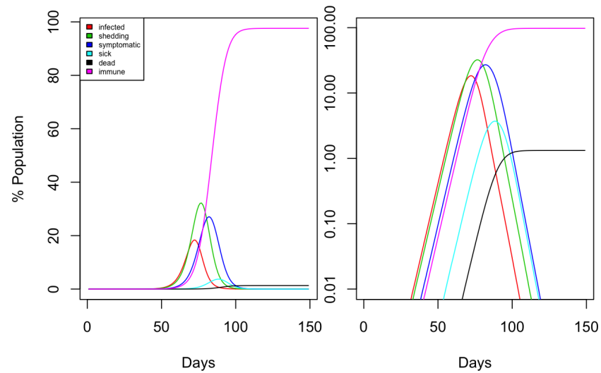
Figure 4: Model simulations with constant R_0 = 2.75 and a population size of 60 million.
