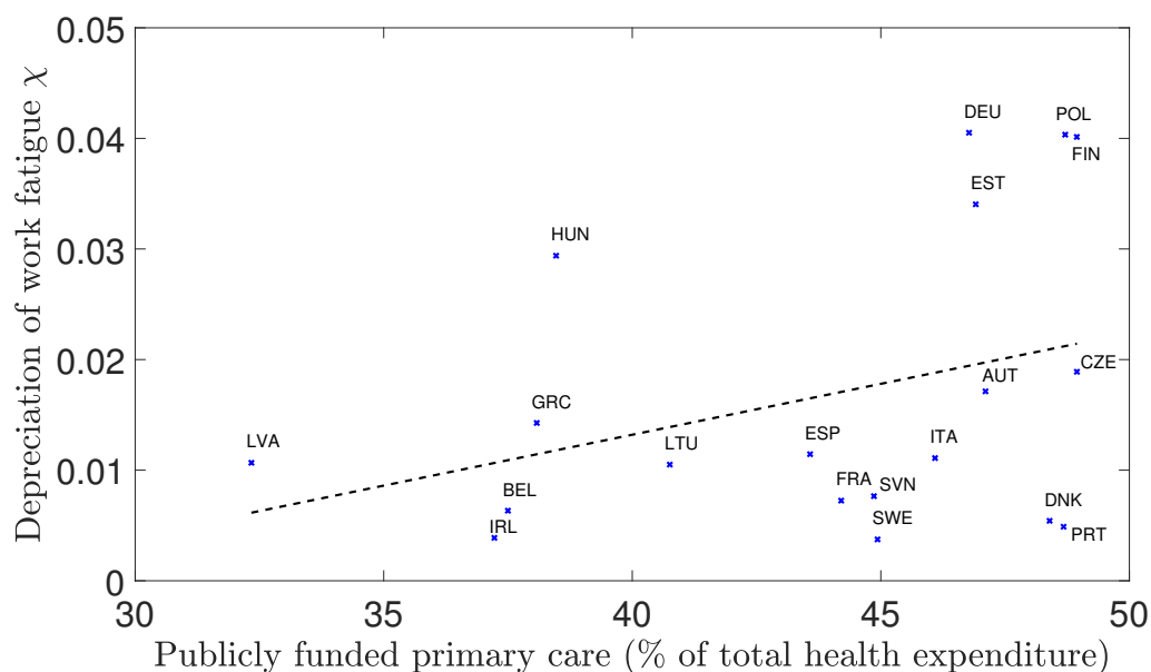
Figure 9: Calibrated values of \chi can partly be explained by primary care public expenditure. The trend line shows the fitted values of a (simple) linear regression, the p -values are reported in parentheses. With slope/coefficient = 0.09 ( p = 0.148 ), and intercept/constant = -0.02 ( p = 0.390 ). The coefficient of determination is given by R^2 = 0.12 , and the sample size is N = 19 .
