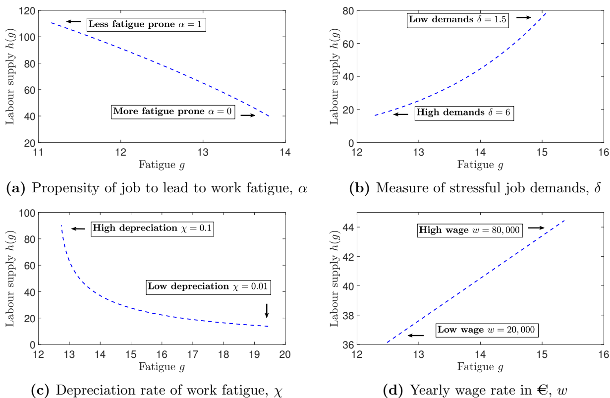
Figure 4: Differentiated effects of institutional background on steady-state values h^* and g^*
