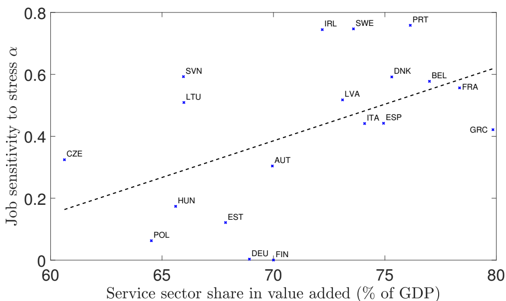
Figure 8: Calibrated values of \alpha can be rationalised by the share of the service sector in GDP in value-added. The trend line shows the fitted values of a (simple) linear regression, the p -values are reported in parentheses. With slope/coefficient = 2.37^{**} ( p = 0.028 ), and intercept/constant = -1.27^* ( p = 0.089 ). The coefficient of determination is given by R^2 = 0.25 , and the sample size is N = 19 .
