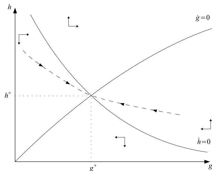
Figure 1: Dynamics of labour supply and fatigue along the stable saddle-path
