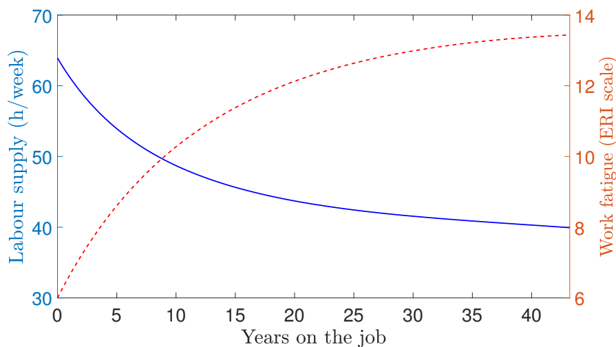
Figure 3: Hours and fatigue profiles over time converge to their steady-state values
