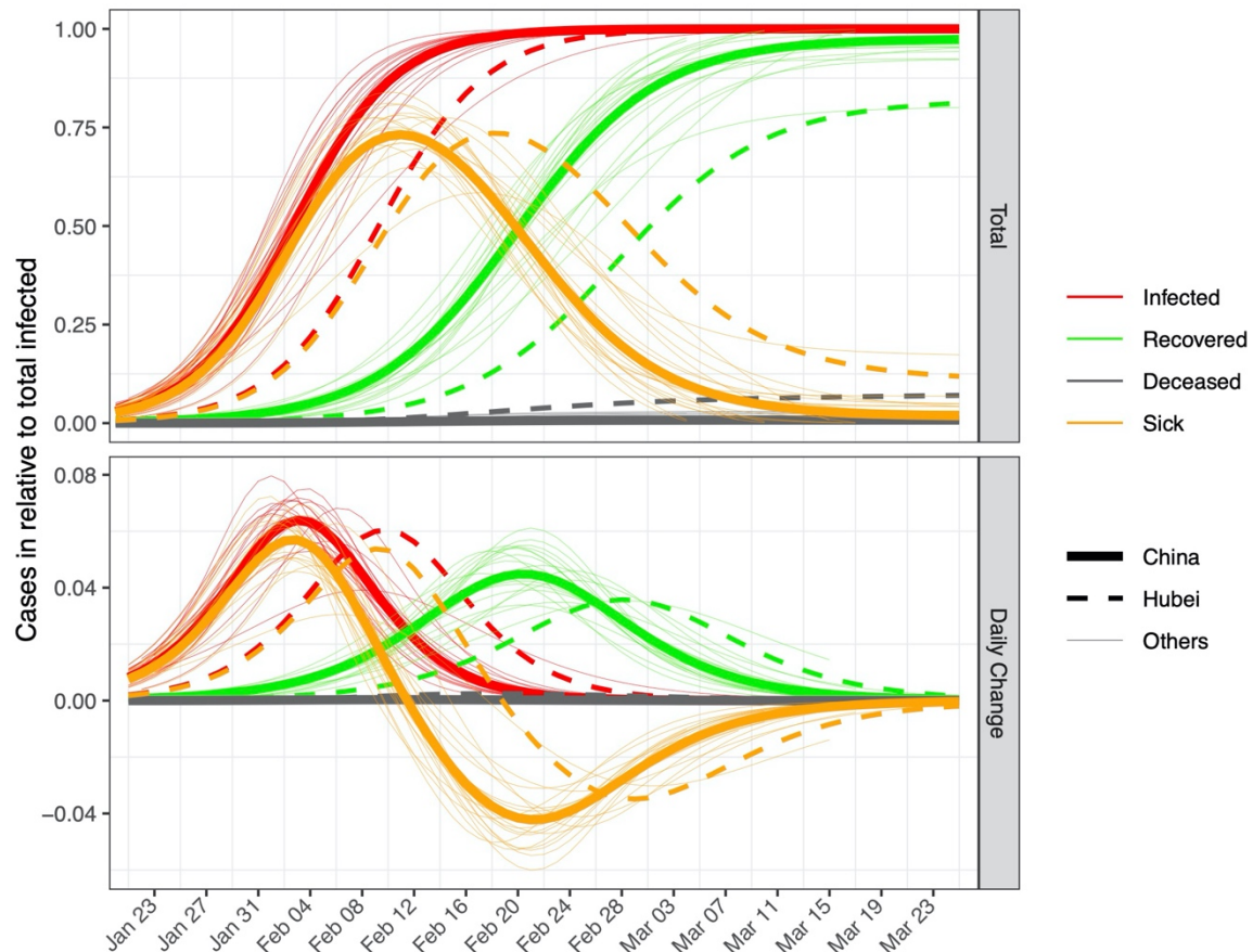
128 129 Fig. 1. Fitted epidemic curves based on the observed data of SARS-CoV2 in China excluding 130 Hubei (thick solid lines), Hubei (dashed lines), and 19 other provinces (thin solid lines). The 131 y-axis of the top panel shows the number of cases relative to the maximum cumulative 132 infected for each region (the value a , see method). The bottom panel shows the daily change 133 on the same relative scale. Red, green and grey colors indicate confirmed, recovered and 134 deceased cases. Orange color indicates the number of “active” sick cases (relative to total 135 infected, top panel), i.e. infected and not yet recovered or deceased, and the daily changes 136 (bottom panel), with negative values in the lower panel indicating that the number of active 137 cases is decreasing. Fitted and observed values for the true number can be found in Fig. A1 138 and Fig. A2 for normal scale and in Fig. A3 and Fig. A4 for log scale.
