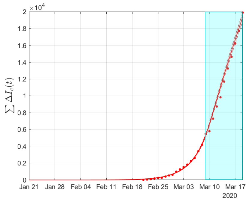
Figure 2: Cumulative number of (confirmed) infected cases resulting from simulations from DAY-ZERO (January 21) until the 19th of March. The DAY-ZERO, \beta = 0.779 , \gamma = 0.0174 were computed by solving the mixed-integer optimization problem for the period DAY-ZERO to March 8. The validation of the model was performed using the reported data of confirmed cases from March 9 to March 19 (shaded area) by taking a 80% reduction in the “effective” transmission rate (see Methodology) to the lockdown of March 8. Dots correspond to the reported data of confirmed cases. Dotted lines depict the upper and lower limits of the estimation.
