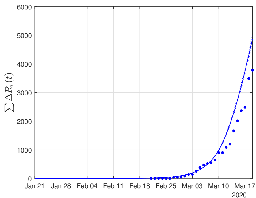
Figure 3: Cumulative number of (confirmed) recovered cases resulting from simulations from DAY-ZERO (January 21) until the 19th of March. The DAY-ZERO, \beta = 0.779 , \gamma = 0.0174 were computed by solving the mixed-integer optimization problem for the period DAY-ZERO to March 8. The validation of the model was performed using the reported data of confirmed cases from March 9 to March 19 (shaded area) by taking a 80% reduction in the “effective” transmission rate (see Methodology) to the lockdown of March 8. Dots correspond to the reported data of confirmed cases. Dotted lines depict the upper and lower limits of the estimation.
