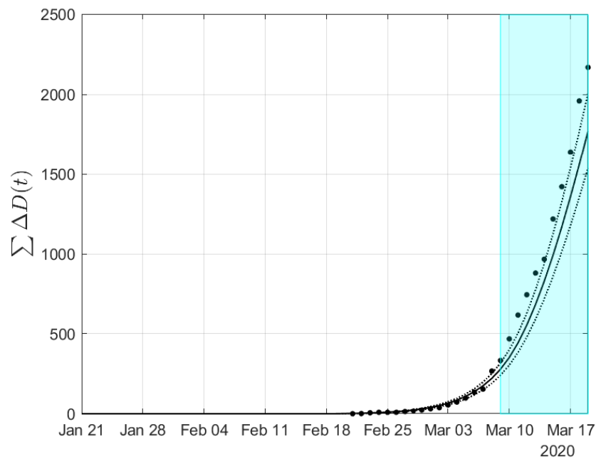
Figure 4: Cumulative number of (confirmed) deaths resulting from simulations from DAY-ZERO (January 21) until the 19th of March. The DAY-ZERO, \beta = 0.779 , \gamma = 0.0174 were computed by solving the mixed-integer optimization problem for the period DAY-ZERO to March 8. The validation of the model was performed using the reported data of confirmed cases from March 9 to March 19 (shaded area) by taking a 80% reduction in the “effective” transmission rate (see Methodology) to the lockdown of March 8. Dots correspond to the reported data of confirmed cases. Dotted lines depict the upper and lower limits of the estimation.
