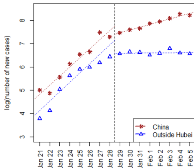
Figure 3: Visualization of daily numbers of newly confirmed case along with date, an obvious change of rate occurred on January 29, 2020.
