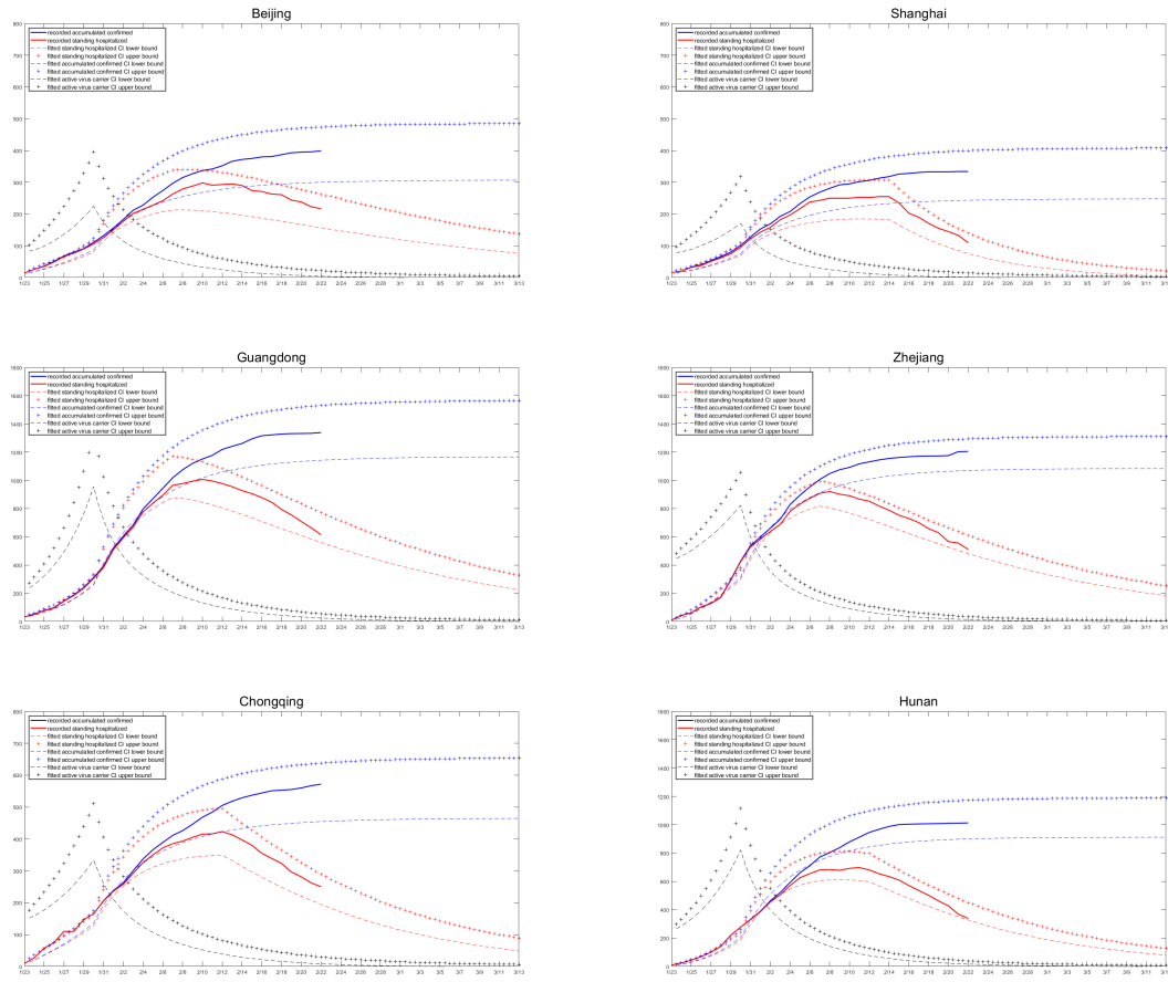
Figure 4: Predicted confidence interval for key populations
