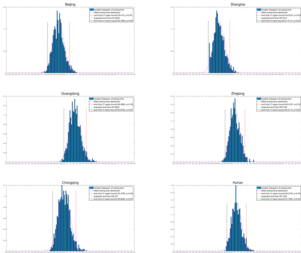
Figure 5: Prediction of the containment time of the outbreak. The containment time of 1000 simulations is plotted as a histogram and is fitted with normal distribution for each region. The y axis represents the density of containment time.
