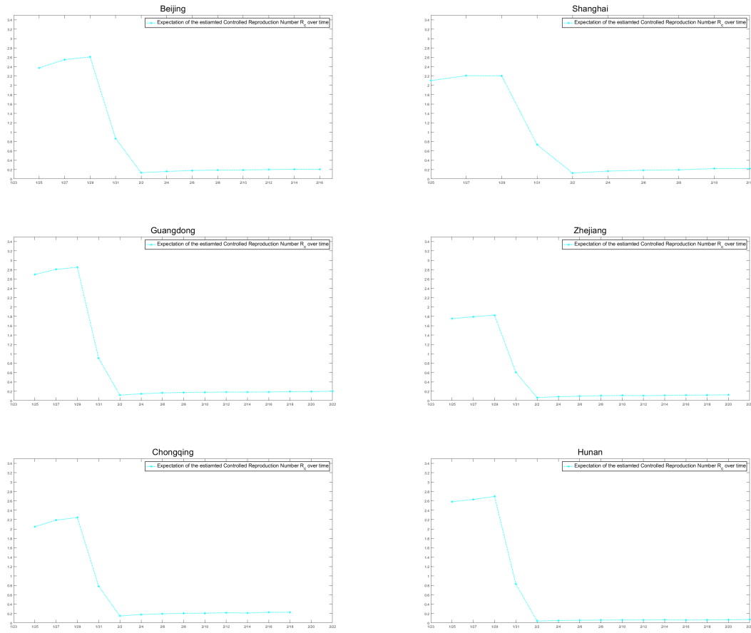
Figure 6: Predicted time-varying R_c curve.
