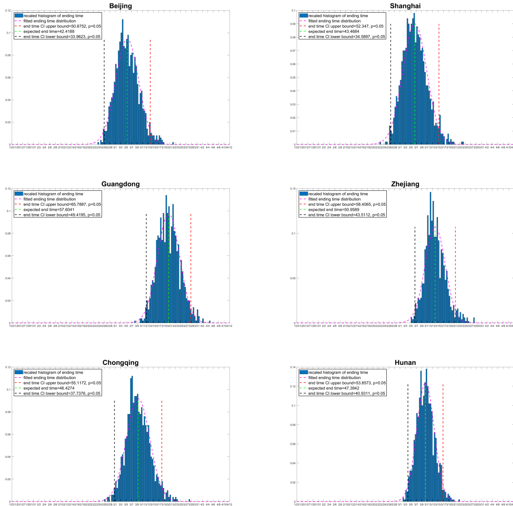
Figure 7: Prediction of the containment time of the outbreak with q = 0 . The containment time of 1000 simulations is plotted as a histogram and is fitted with normal distribution for each region. The y axis represents the density of containment time.
