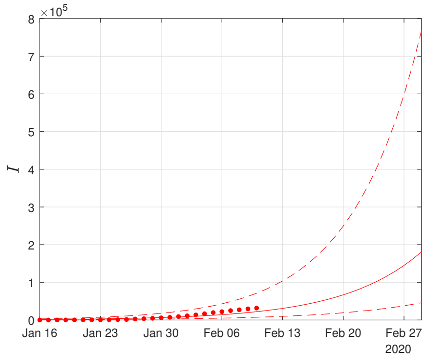
Fig 6. Scenario I. Simulations until the 29th of February of the cumulative number of infected as obtained using the SIRD model. Dots correspond to the number of confirmed cases from the 16th of January to the 10th of February. The initial date of the simulations was the 16th of November with one infected, zero recovered and zero deaths. Solid lines correspond to the dynamics obtained using the estimated expected values of the epidemiological parameters \alpha = 0.191 , \beta = 0.064d^{-1} , \gamma = 0.01 ; dashed lines correspond to the lower and upper bounds derived by performing simulations on the limits of the confidence intervals of the parameters.
