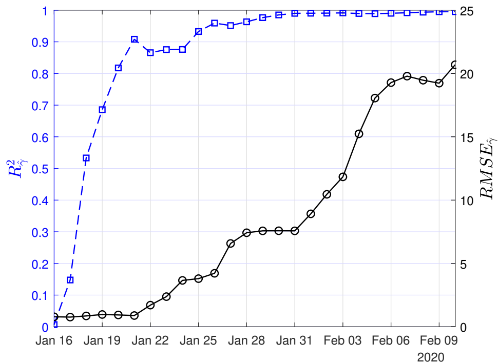
Fig 13. Scenario II. Coefficient of determination ( R^2 ) and root mean square error ( RMSE ) resulting from the solution of the linear regression problem with least-squares for the mortality rate ( \gamma ).
