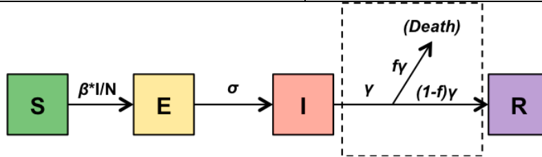
FIGURE 1. In this schematic diagram of the SEIR model, each box represents a compartment of the population, and arrows show the progression of individuals through those compartments. Expressions above arrows are rate coefficients showing progression through compartments. Note that the dashed boxed portion, indicating individuals leaving the population because of death, will not be included in future diagrams for simplicity.
