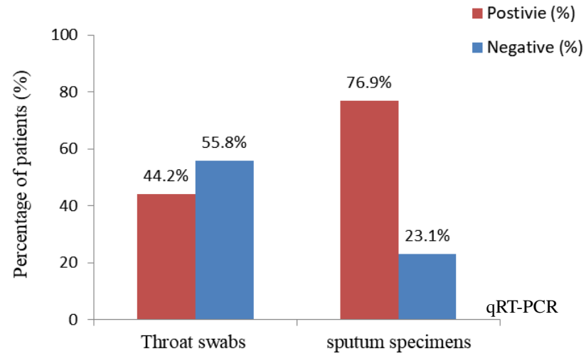
Figure 1. Distribution of qRT-PCR results on throat swabs and sputum specimens in patients with suspected COVID-19.
