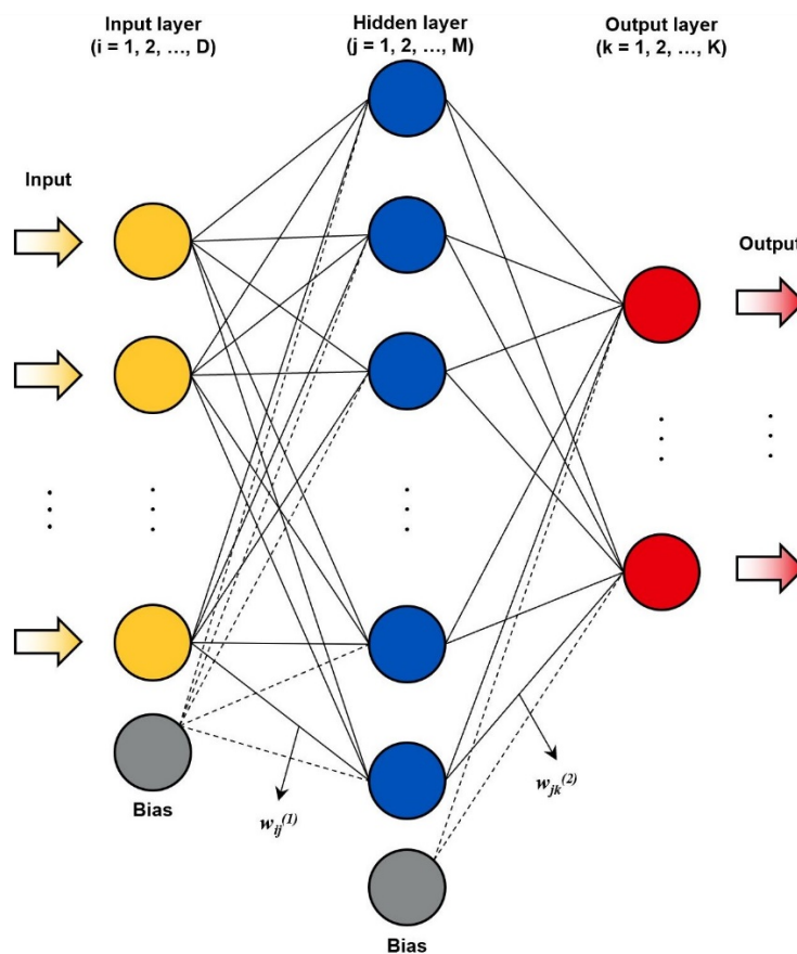
Figure 1. Schematic example of an ANN structure with a single hidden layer ( w_{ij}^{(1)} = weighted connection between i -th node in the input layer and j -th node in the hidden layer and w_{jk}^{(2)} = weighted connection between j -th node in the hidden layer and k -th node in the output layer; i = 1, 2, \dots, D ; j = 1, 2, \dots, M ; k = 1, 2, \dots, K )
