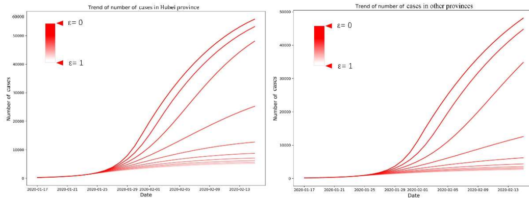
FIGURE 2. Confirmed cases under different \epsilon , the x-axis is date, the y-axis is number of confirmed cases.
