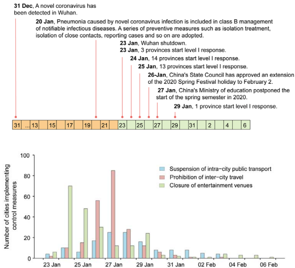
362 Figure 1 Timeline of implementation of transmission control measures against COVID-19 in 363 China.
