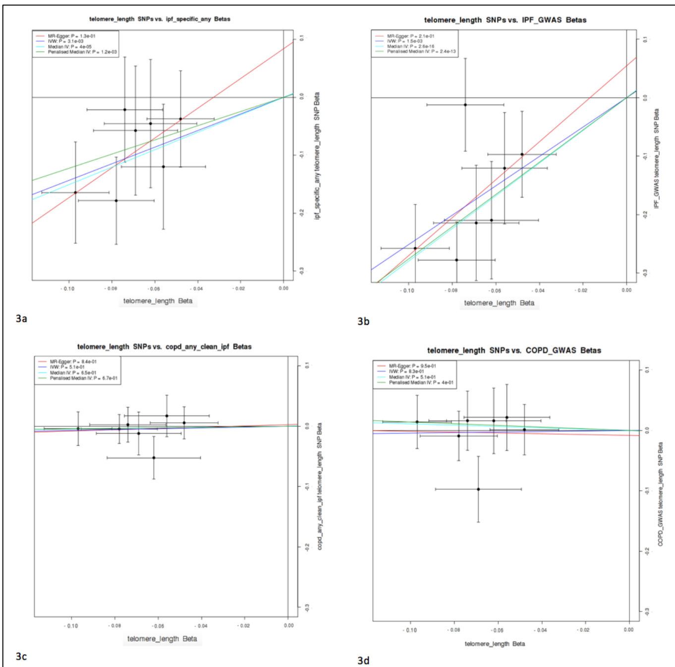
Figure 3. Two-sample MR results for IPF and COPD showing evidence of telomere length causality in IPF but not in COPD. Graphs show the strength of the relationship between disease incidence and telomere length SNPs on the y axis against the telomere length association from previous GWAS for each SNP on the x axis. A non-zero gradient to the lines, with significant p values shown in the top left-hand box for the different MR models used, is evidence of causality of telomere length for disease. Results shown are for all seven telomere variants for (a) IPF ('narrow') in UK Biobank, (b) IPF Replication Cohort, (c) COPD in UK Biobank, (d) COPD Replication Cohort
