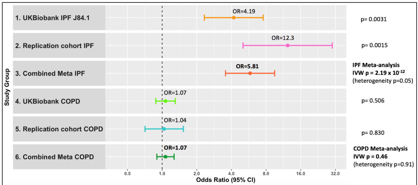
Figure 4. Meta-analysis results for IPF and COPD in UK Biobank and replication cohorts showing significant evidence of telomere length causality in IPF and not COPD across cohorts. Odds ratios and 95% confidence intervals for IPF ('narrow') in UKB, IPF Replication Cohort, IPF meta-analysis, COPD in UK Biobank, COPD Replication Cohort and COPD meta-analysis using IVW Method.
