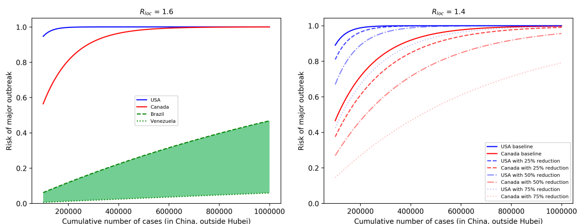
Figure 2. In the left: Risk of major outbreaks as a function of cumulative number of cases in selected countries, assuming R_{loc} = 1.6 and baseline connectivity to China. Other countries in South America, and Mexico are inside the green shaded area. In the right: the effect of the reduction of imported case numbers (either by travel restriction or entry screening) in the USA and Canada, assuming R_{loc} = 1.4 .
