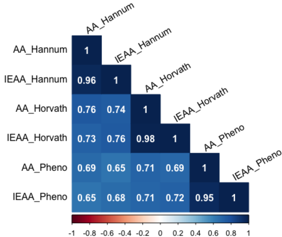
Figure 2: Correlation matrix of age acceleration metrics estimated by three epigenetic clocks. Legends: Spearman's rank correlations between each pair of epigenetic age acceleration (AA) or intrinsic epigenetic age acceleration (IEAA) metrics estimated by Hannum clock, Horvath clock, and PhenoAge are shown in the boxes of the matrix.
