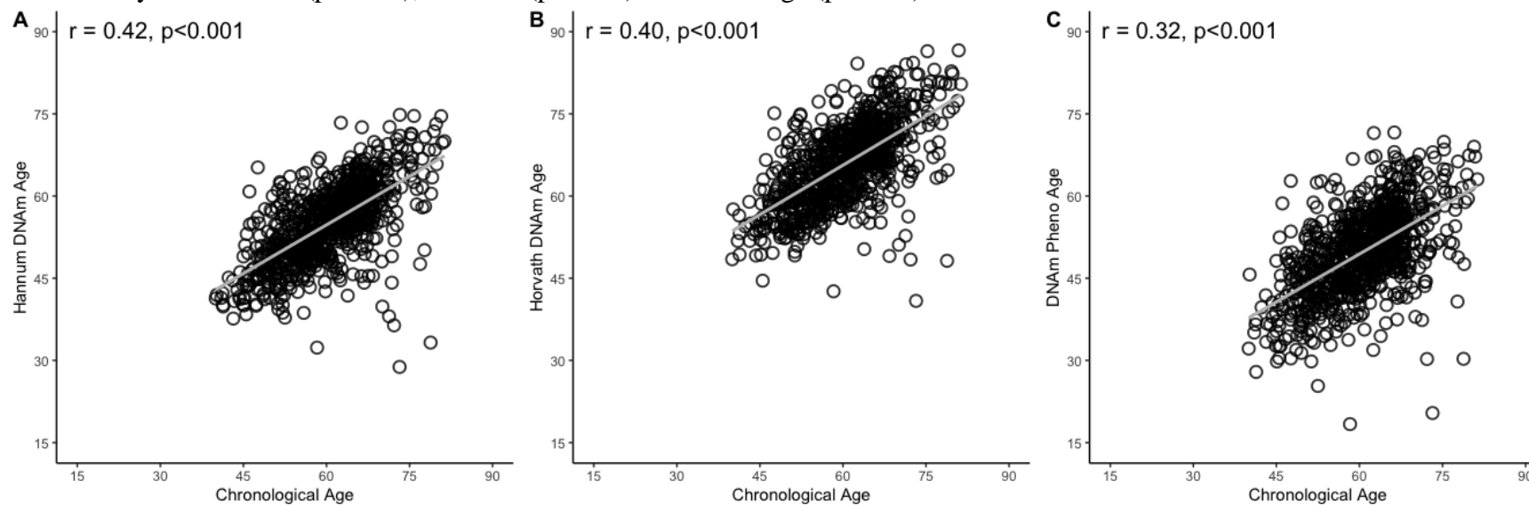
Figure 1: Correlations between chronological age and DNAm age estimated by three epigenetic clocks. Legends: Scatterplots with Pearson correlation coefficients ( r ) and p-values for the relationship between chronological age and DNA methylation age estimated by the Hannum (panel A), Horvath (panel B) and PhenoAge (panel C) clocks.
