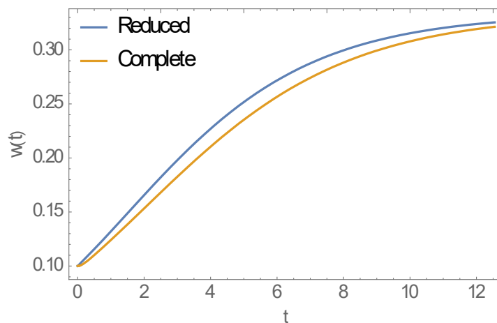
Figure A: Relaxation patterns of stationary MacDonald systems (reduced model, full model). Both systems relax to the same equilibrium w^* = 1 - 1/R_0 , but reduced model predicts faster relaxation rate.
