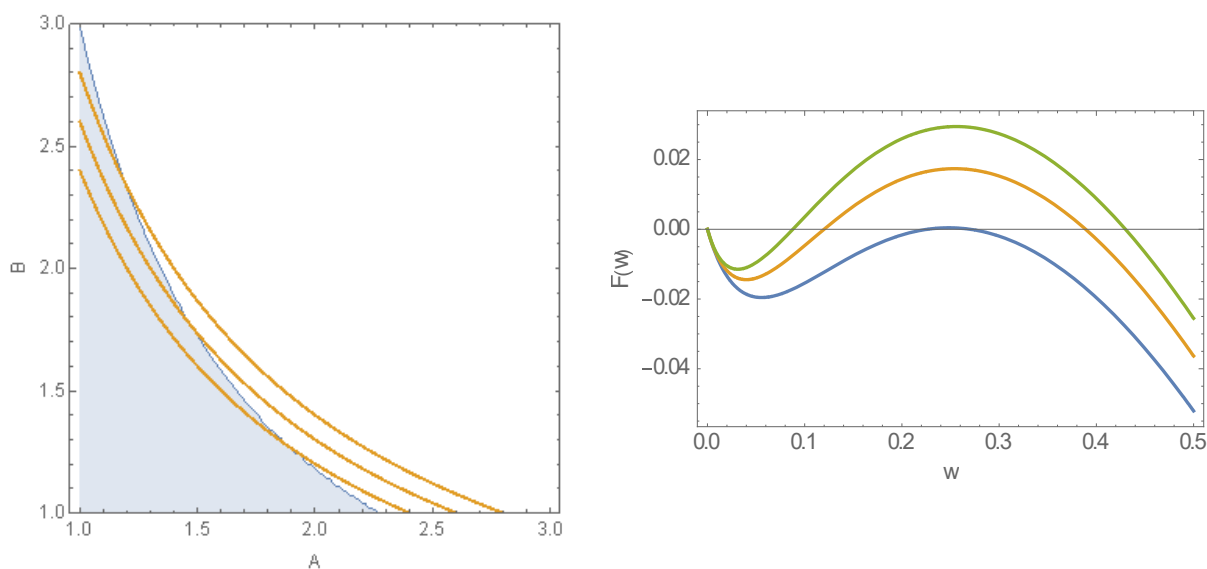
Figure F: (a) (A, B) parameter space of MacDonald system with mating for rescaled parameters A \rightarrow A / (\gamma + \mu) , B \rightarrow B / \nu . Shaded region is ‘stable zero’ (elimination case); open region has triple (bistable) equilibria. Orange lines are isocontours of R_0 = AB = \{2.4, 2.6, 2.8\} . (b) Functions F(w | A, B) of reduced MacDonald system, for fixed R_0 = 2.6 , and 3 values A = \{1.5, 2, 2.5\} . Case R_0 = 2.6 ; A = 1.5 is close to bifurcation (zero \rightarrow triple equilibria).
