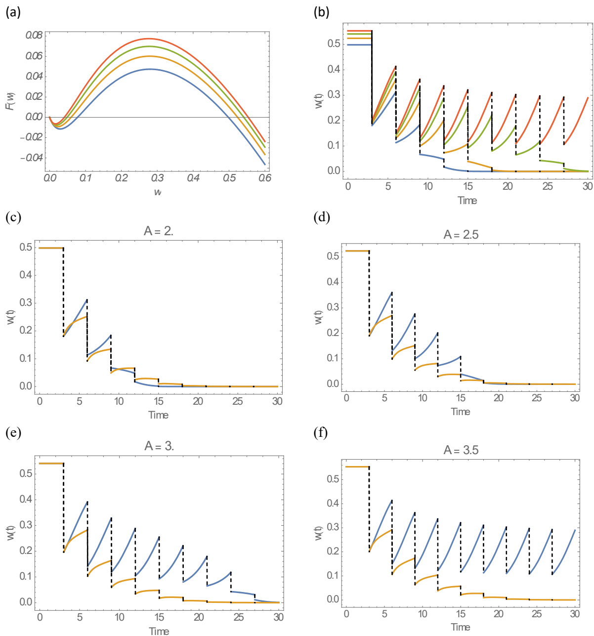
Figure G: MDA control of MacDonal system with mating, fixed R_0 = 3 , and 4 vales of transmission coefficient A = 2 - 3.5 . Panel (a) shows the corresponding reduced MacDonal functions Error! Reference source not found. and equilibria. Panel (b) MDA histories of 4 communities. Panels (c-f) compare MDA histories of the reduced model (blue) and the complete MacDonal (yellow), for 4 choices of A .
