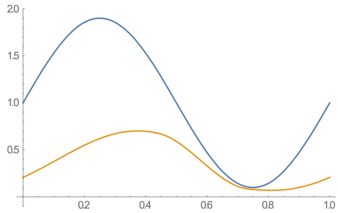
Figure 1: Sustained seasonal patterns of the reduced MacDonald system and complete host-vector systems for R_0 = 2 . Total snail N(t) (blue), infected y(t) (yellow). Rapid decline of N(t) , brings y(t) close to N .
