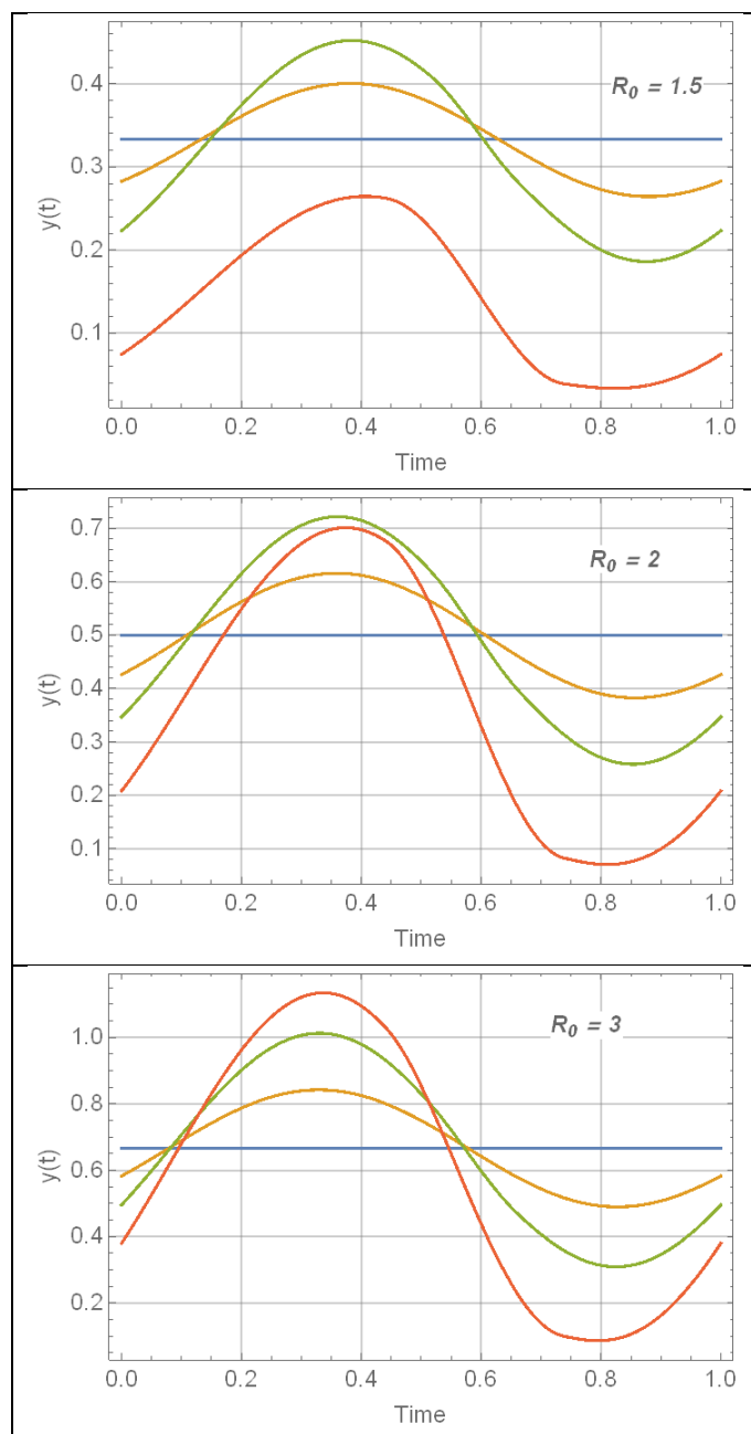
Figure H: Periodic snail solutions y(t) for 3 R_0 values of Table 1, and amplitude range 0 \leq \alpha \leq .9 (blue to red).
