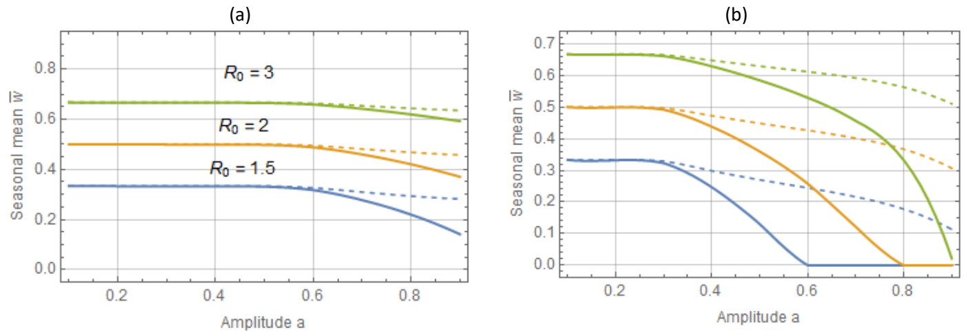
Figure 3: Seasonal mean \bar{w}(a) = \langle w^*(t, a) \rangle as functions of amplitude a : type I trigonometric N(t, a) panel (a), and type II peak – panel (b). The full human-snail MacDonald (solid) vs. reduced system (dashed) for 3 values R_0 = 1.5; 2; 3 . Reduced model departs significantly from the full system at large seasonal amplitude ( a > .6 ). It can thus over-predict seasonal mean burden by wide margin.
