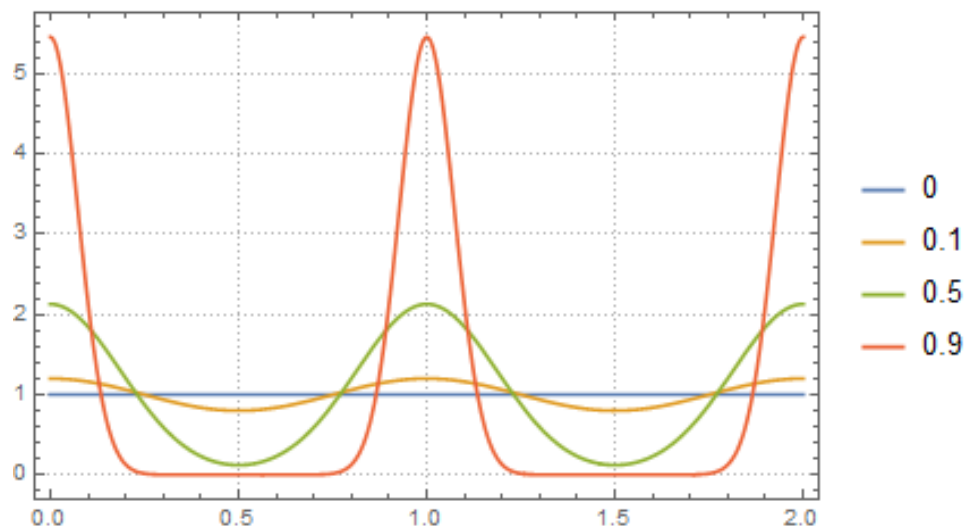
Figure 1: Examples of type II 'peak seasonality', modeled by elliptic theta function,
