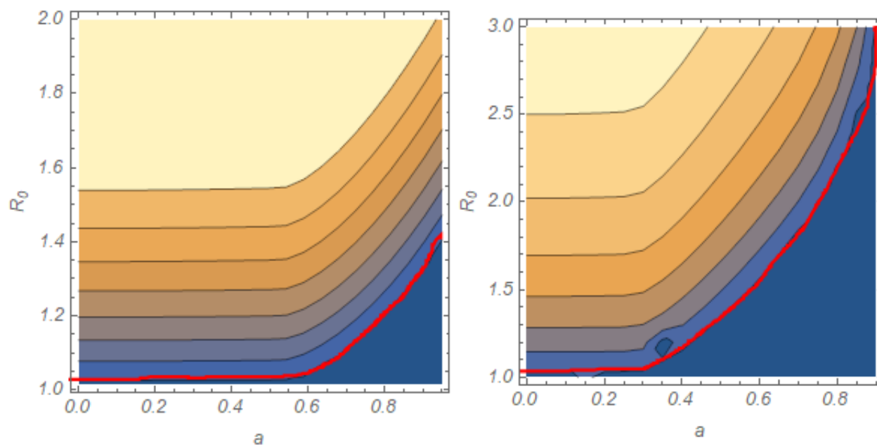
Figure 4: Iso-contours of seasonal mean MWB function \bar{w}(a, R_0) = C : left panel is trigonometric N(t, a) , right panel – peak-type N(t, a) . The range of contour values: 0 < C < 0.35 (left), and 0 < C < 0.6 (right). Thick red curve marks the boundary between endemic region (above), and zero-infection (below).
