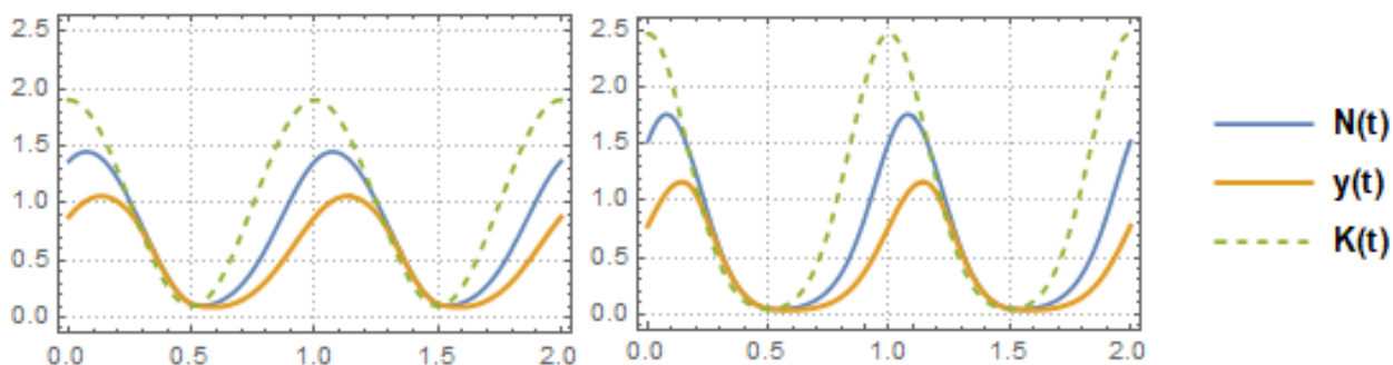
Figure B: Typical seasonal patterns for logistic snail model with CC-function K(t, a) , relative growth rate \beta/\nu = 5 , and snail mortality \nu = 4 /year. Left panel show shows MacDonald solution \{N(t), y(t)\} for trigonometric K(t, a) of
