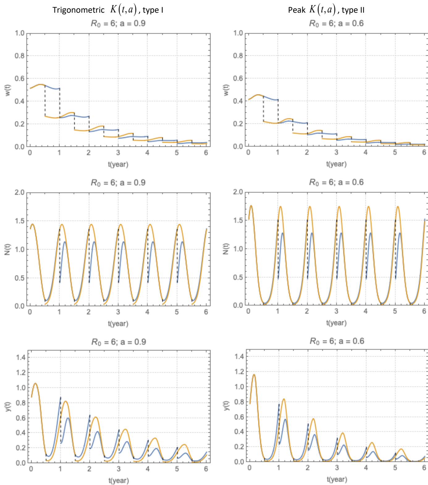
Figure 7: Combined MDA + molluscicide strategies for type I-II seasonality (left-right panels). Two curves correspond to start of season (suboptimal timing \tau = 0 ), and mid-season ( \tau = 0.5 , close to optimal).
