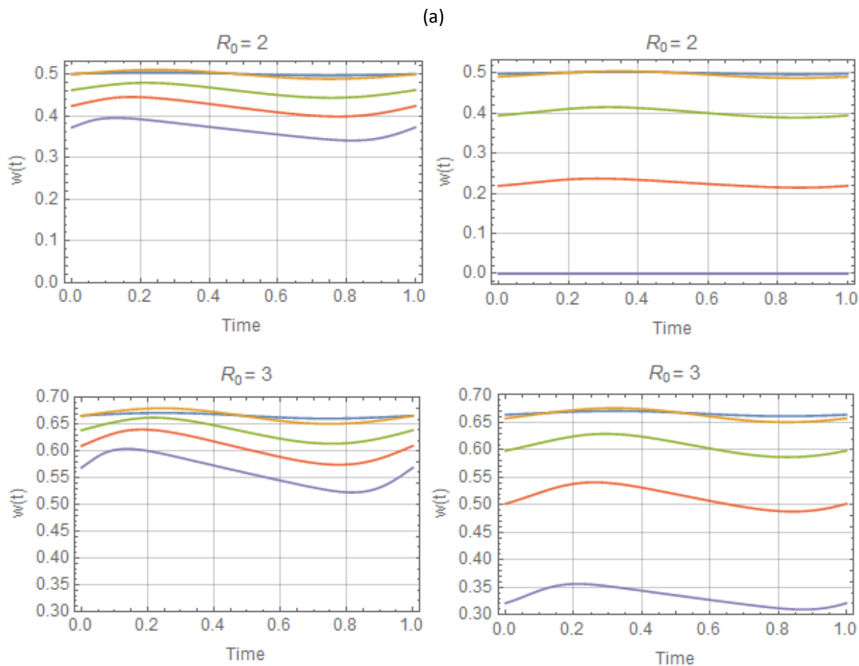
Figure D: Periodic solutions w^*(t, a) for - peak-type N(t|a) , with R_0 = 2, 3 , and a range of amplitude values 0 \leq a \leq .8 (top to bottom). As in Figure C, left column shows reduced system, right column - complete system.
