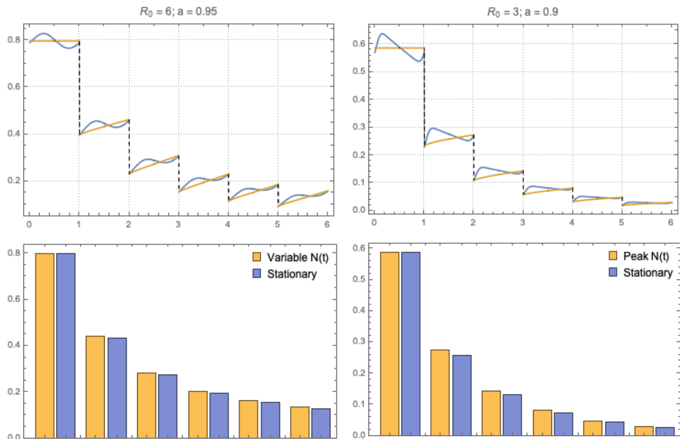
Figure 5: Annual MDA regimen for MacDonal system (1.7) with 2 types of seasonality and its adjusted stationary system: type I (left column) and type II (right column). Top plots compare MDA histories of seasonal MacDonal (blue) vs. the corresponding stationary (seasonal mean) MacDonal (yellow). Bottom panels show their seasonal-mean burden on tears 1-6.
