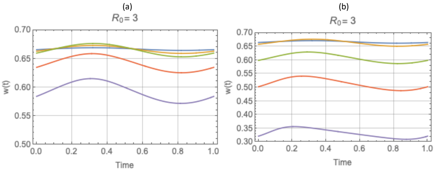
Figure 2: Periodic solutions w^*(t) of complete system: type I trigonometric N(t) (left panel) and type II peak N(t) (right panel), for values of R_0 = 3 and amplitude range 0 \leq a \leq 1 , descending from stationary equilibrium a = 0 (blue) to a = .95 (purple).
