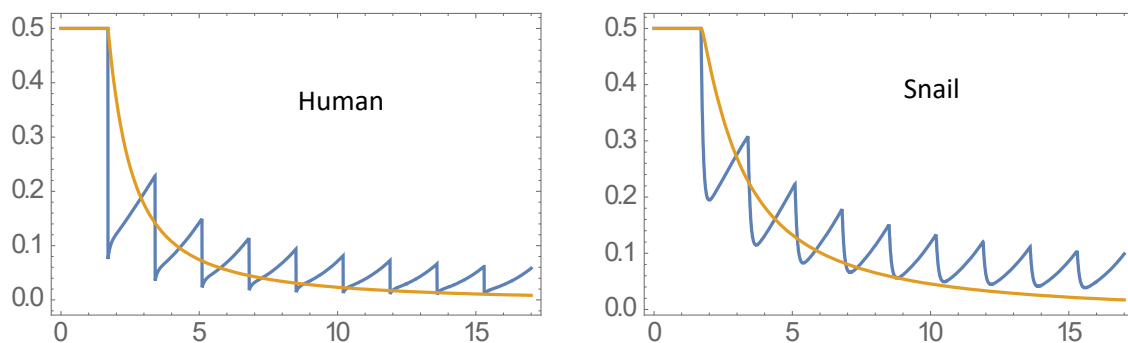
Figure E: Averaging effect on MDA: two panels compare repeated periodic MDA history (blue), and the corresponding ‘mean drug clearing’ model (yellow). The former approaches limit cycle regime, the latter goes to elimination (effective BRN R_{ef} < 1 ). Here we have chosen treatment period T = 1.7 < T_c = 1.89 .
