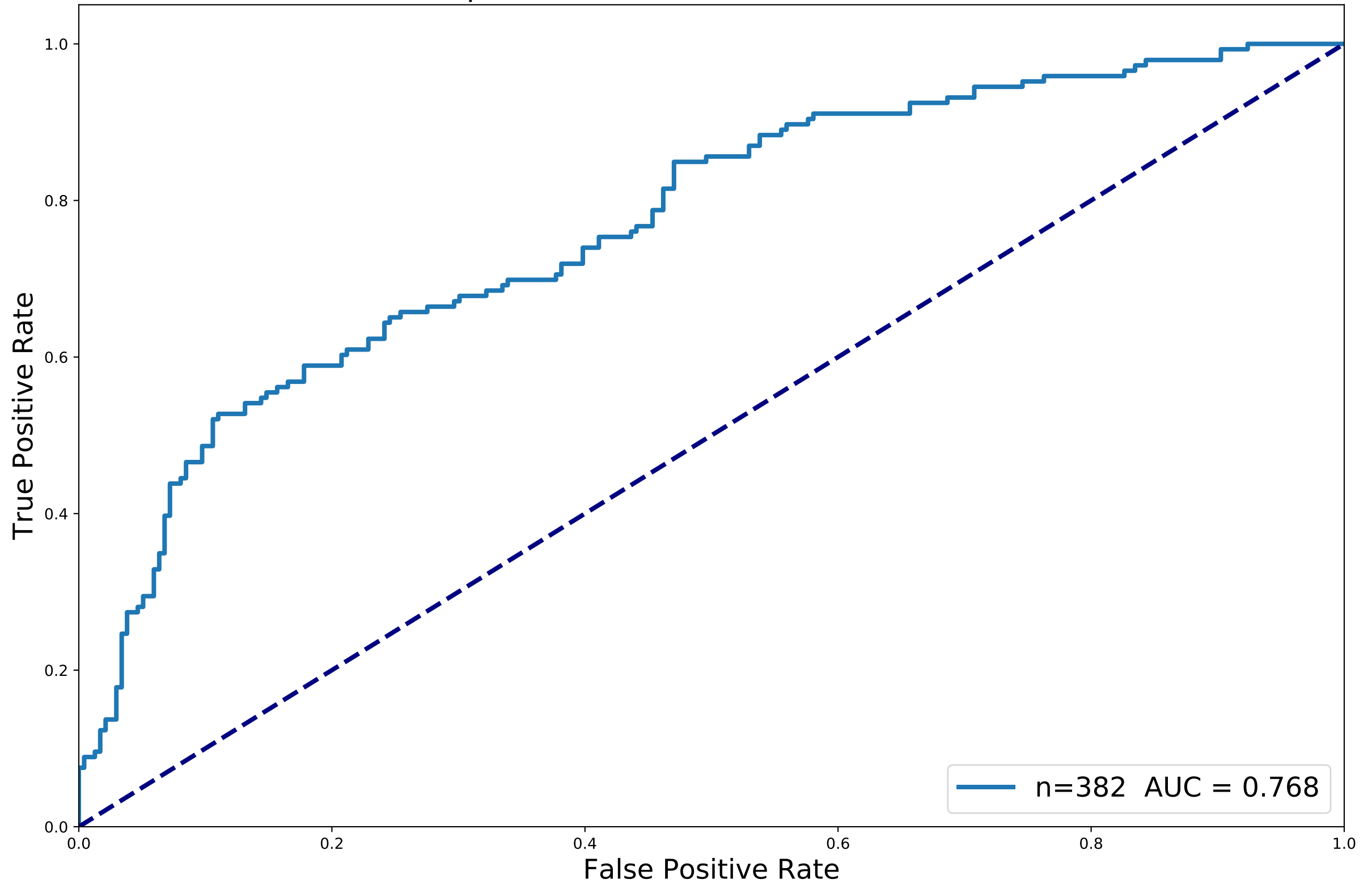
Alcohol Dependence Classifier ROC Curve on Test Set
