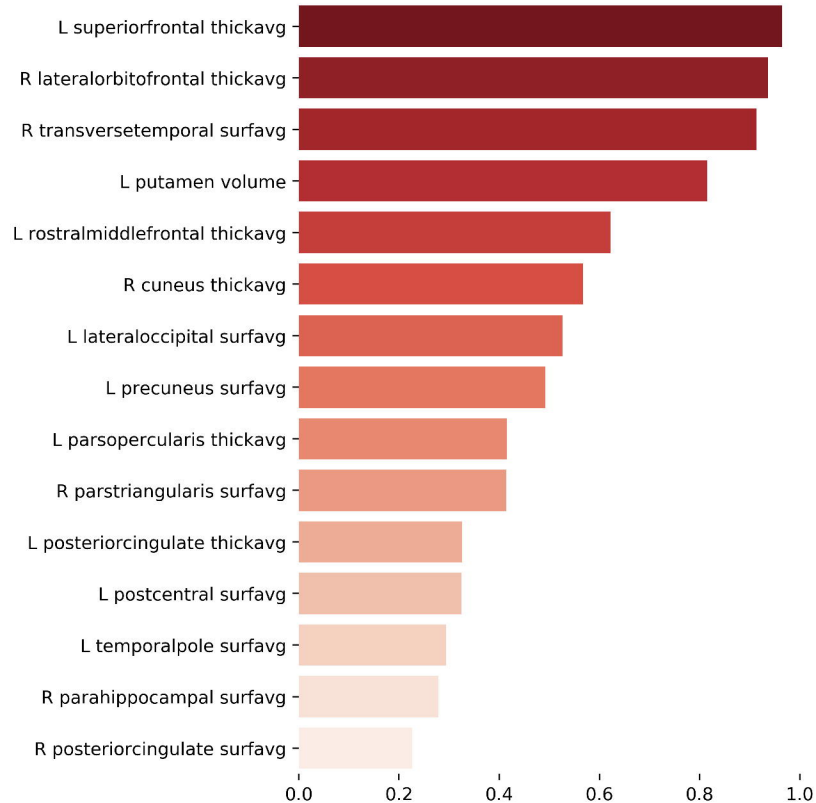
Top 15 Features
