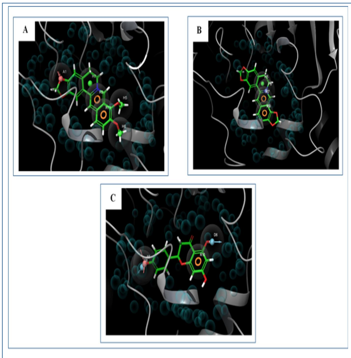
Figure 10. 3D representation of the pharmacophore modelling of the three best ligand molecules.
