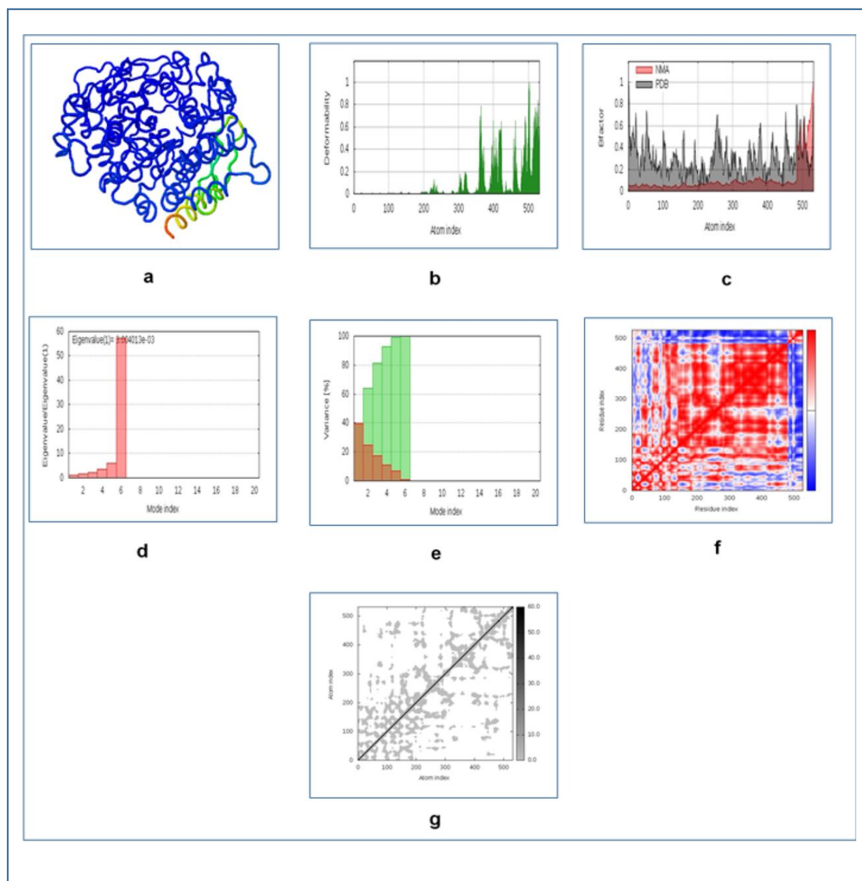
Figure 12. Results of molecular dynamics simulation of coptisine-acetylcholinesterase docked complex. (a) NMA mobility, (b) deformability, (c) B-factor, (d) eigenvalues, (e) variance (red color indicates individual variances and green color indicates cumulative variances), (f) covariance map (correlated (red), uncorrelated (white) or anti-correlated (blue) motions) and (g) elastic network (darker gray regions indicate more stiffer regions) of the complex.
