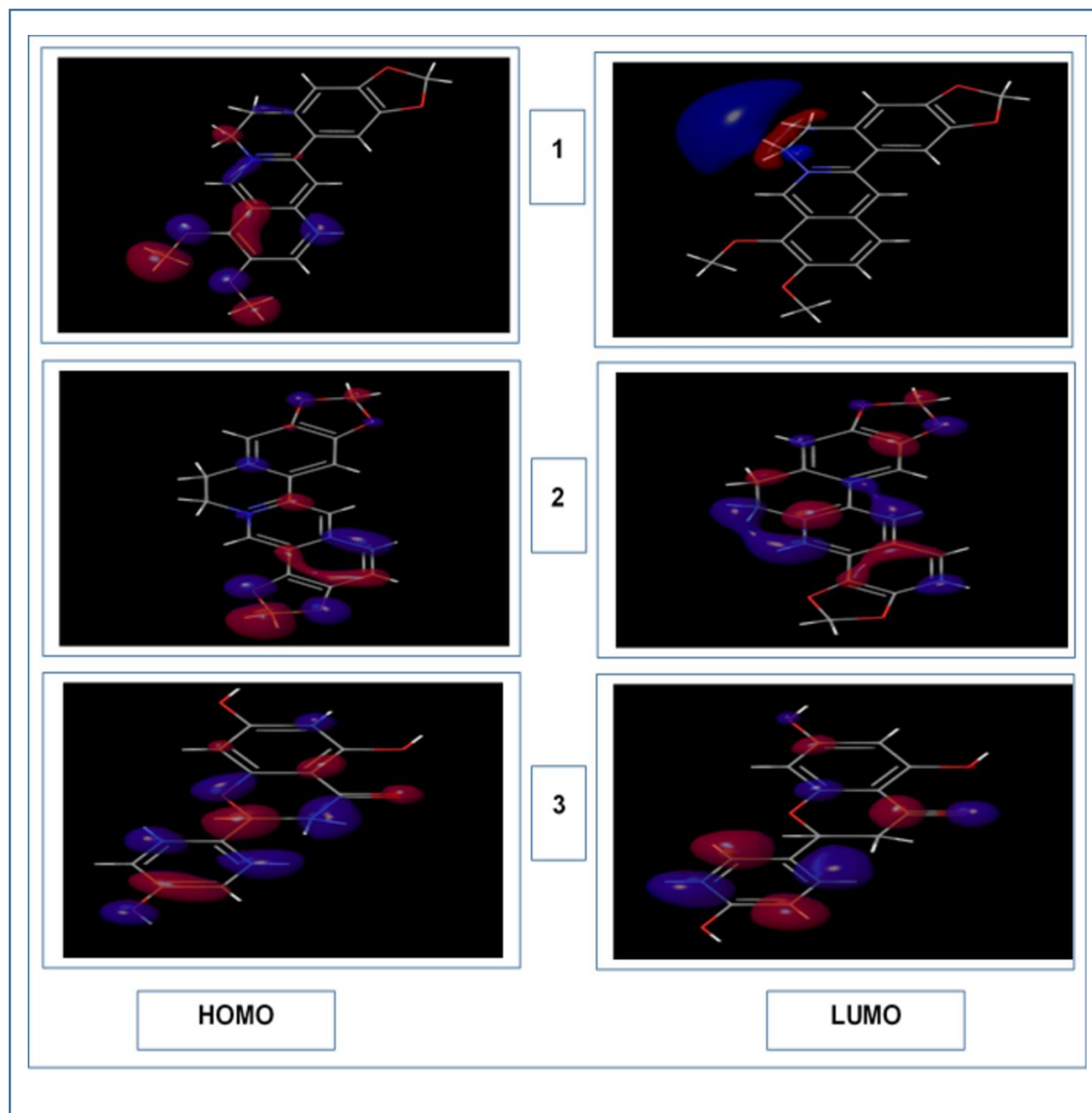
Figure 11. The results of DFT calculations (HOMO-LUMO structures) of, 1. Berberine, 2. Coptisine, 3. Naringenin. The HOMO structures are illustrated in the left column and the LUMO structures are illustrated in the right column.
