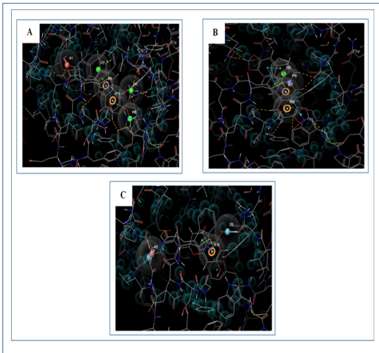
Figure 09. 2D representation of the pharmacophore modelling of the three best ligand molecules.
