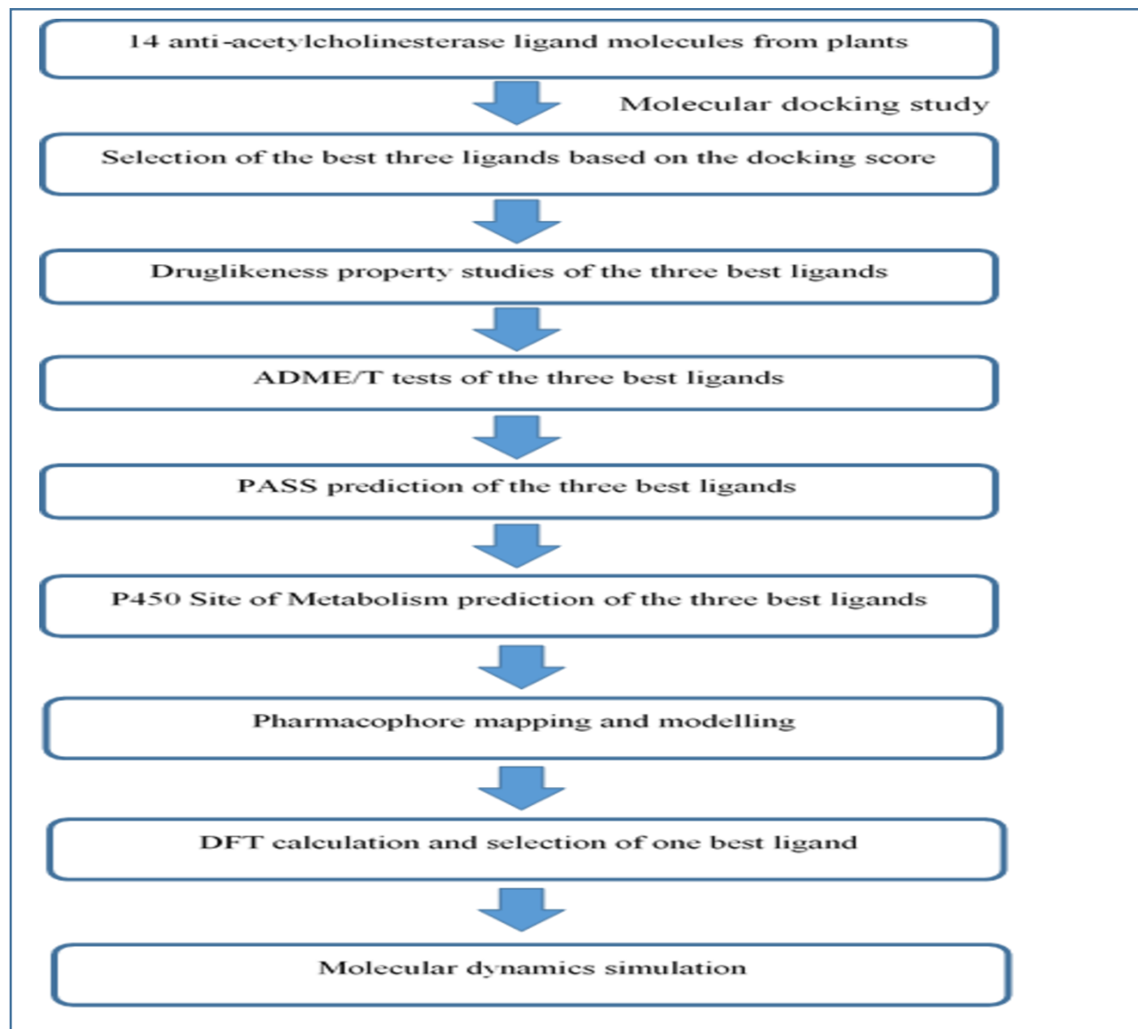
Figure 02. The flowchart of the work-plan of the experiment.
