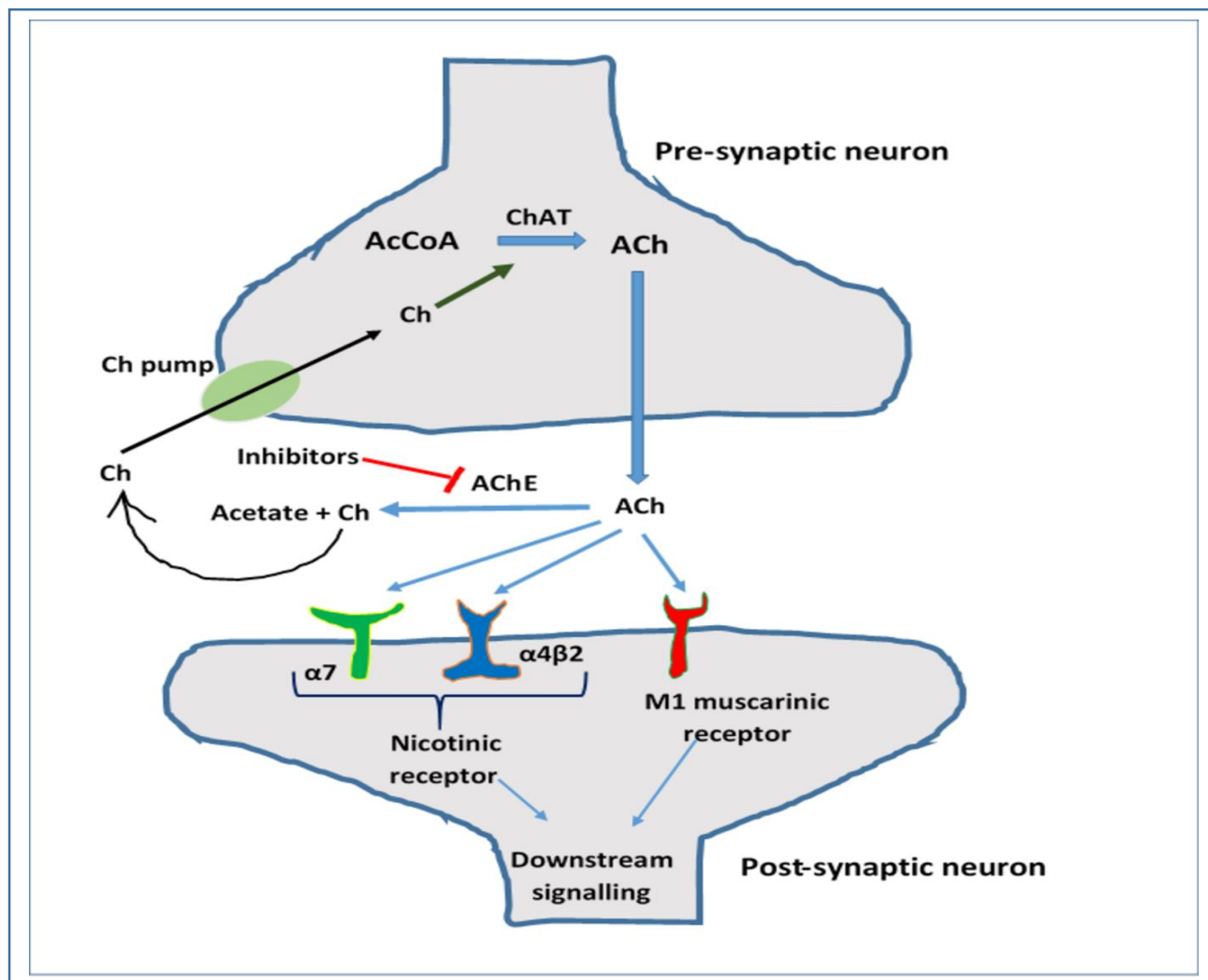
Figure 01. Cholinergic hypothesis and role of acetylcholinesterase in AD development. Acetylcholine (ACh) is synthesized (synthesizing reaction is catalysed by choline acetyltransferase, ChAT) and released by the pre-synaptic neuron. The acetylcholine mediates its effects on the post-synaptic neuron through nicotinic and/or muscarinic receptors. The ACh later performs the downstream signalling in the post-synaptic neuron. Acetylcholinesterase (AChE) enzyme breaks down the ACh and overexpression of AChE lowers the amount of acetylcholine in the brain which leads to the AD onset. AChE inhibitors repress the AChE activity, thus aid in the AD treatment.
