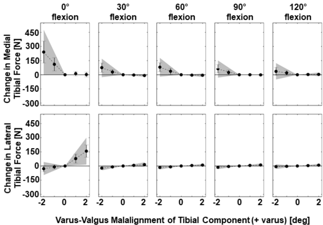
Figure 2. Plots show means (points) and standard deviations (error bars) of the changes in the medial and lateral tibial forces caused by V-V malalignment of the tibial component. Dotted lines show the significant relationships ( p < 0.05 ) between the changes in tibial force variables and V-V malalignments (Table 1). The shaded grey regions show the 95% tolerance intervals for the sensitivities.
