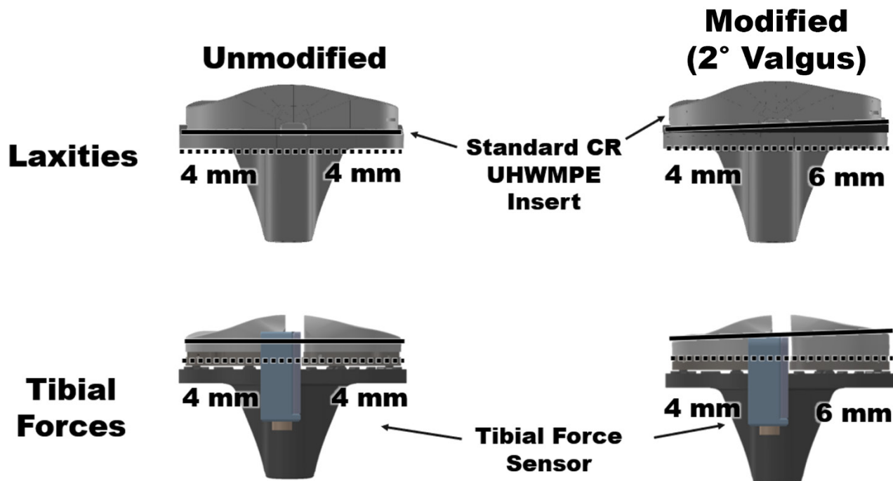
Figure 1. Renderings show the design of the modified tibial baseplates used when measuring the laxities (top row) and the design of the modified articular surface inserts used when measuring the tibial forces (bottom row). For the tibial baseplate, the modifications consisted of rotating the proximal features of the baseplate that secured the insert in place (solid black line) relative to the distal surface of the baseplate that interfaced with the cement mantle (dotted black line). Because the geometry of the distal surface was not changed, all baseplates could be implanted using the same cement mantle in each knee. The geometry of the proximal locking features of the tibial baseplate was also unchanged so the same standard UHMWPE (ultra-high molecular weight polyethylene) liner could be used in all knees. For the articular surface inserts, the modifications consisted of rotating the proximal articular surface (solid black line) relative to the distal surface that secured the inserts to the tibial force sensor (dotted black line) 21 . The modified tibial baseplate and articular surface inserts (left column) are an example of one of the four modified tibial baseplate and articular surface inserts created for each size tibial component. In the example case of a 2° valgus malalignment, the medial side of the tibial component is approximately 2 mm thicker than the lateral side.
