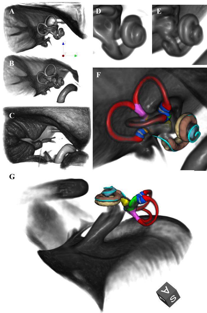
Figure 4: Volume renderings of inner ear templates and atlas (ROI size: 4 \times 4 \times 3 cm; resolution: 0.2 mm isotropic; viewpoint: right-lateral view onto right inner ear). Panels: A. T2 template; B. CISS template; C. T1 template; D. Closeup cochlea in T2 template; E. Closeup cochlea in CISS template, with a clear separation of scala tympani and vestibuli; F. Atlas surface meshes on CISS template volume rendering. G. Same as F, with a different perspective focussing on the vestibule. Colors and regions: red: semicircular canals; blue: ampullae; pink: common crus; grey: cupula walls; green: utricle; yellow: saccule; brown: scala vestibuli; beige: scala tympani; light blue: cochlear cupula; cyan: cochlear duct. ( Print in color. )
