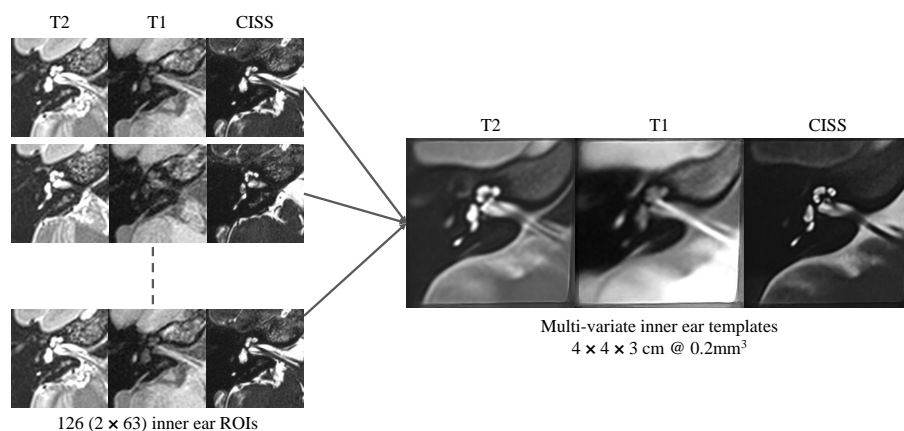
Figure 2: Inner ear template building input: three of 126 example multi-variate inputs (T2, T1, CISS) of the inner ear region are shown, centered, Reid’s plane aligned and cropped with a 4 \times 4 \times 3 cm ROI. The geodesic mean template is reconstructed and shown on the right side.
