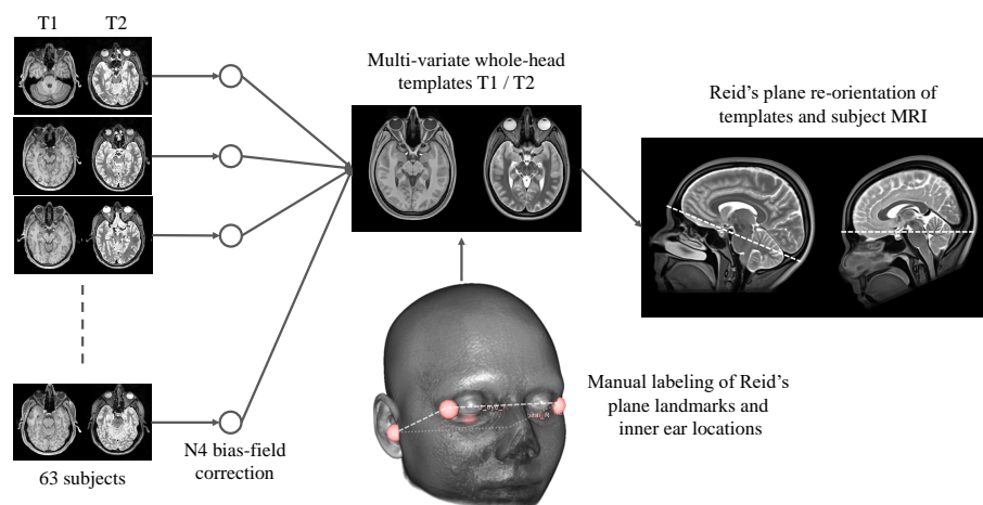
Figure 1: Full-brain template building and annotation, for re-orientation of the axial plane to Reid's standard plane, and for localization of left/right inner ear region-of-interests (ROI). (Print in color.)
