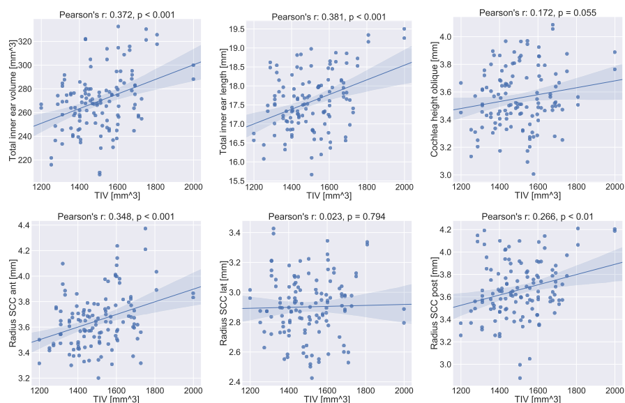
Figure 5: Correlation plots for inner ear measurements with total intracranial volume (TIV). Linear correlation values (Pearson’s r ) and corresponding p -values are indicated in the subplot titles. The 95% confidence interval for the regression estimate is drawn as a translucent band around the regression line. Total inner ear volume and length, as well as the radii of the anterior and posterior semicircular canals (SCC) are linearly correlated with head size. The oblique cochlea height might well be while the radius of the lateral SCC appears to not be correlated at all with TIV. The results indicate the importance of TIV for future quantitative assessments between cohorts.
