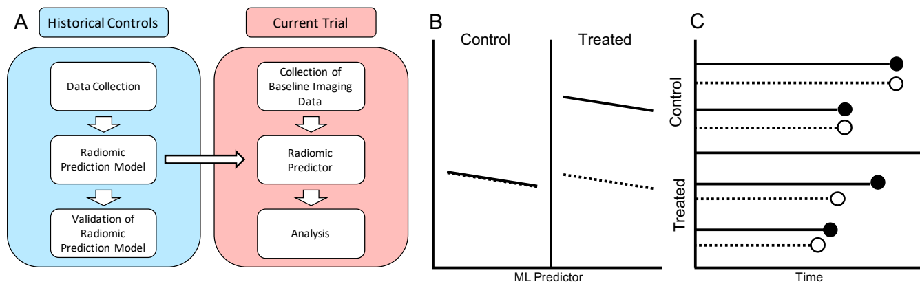
Fig. 1. A: Workflow for implementing the proposed method in a new clinical trial. B (continuous) and C (survival outcome): Schematic diagram for individualized predictions that are generated for each person in the current trial, where the solid lines indicate observed outcome for the participants of the current trial and the dashed lines indicate predicted outcome for those participants had they not been treated.
