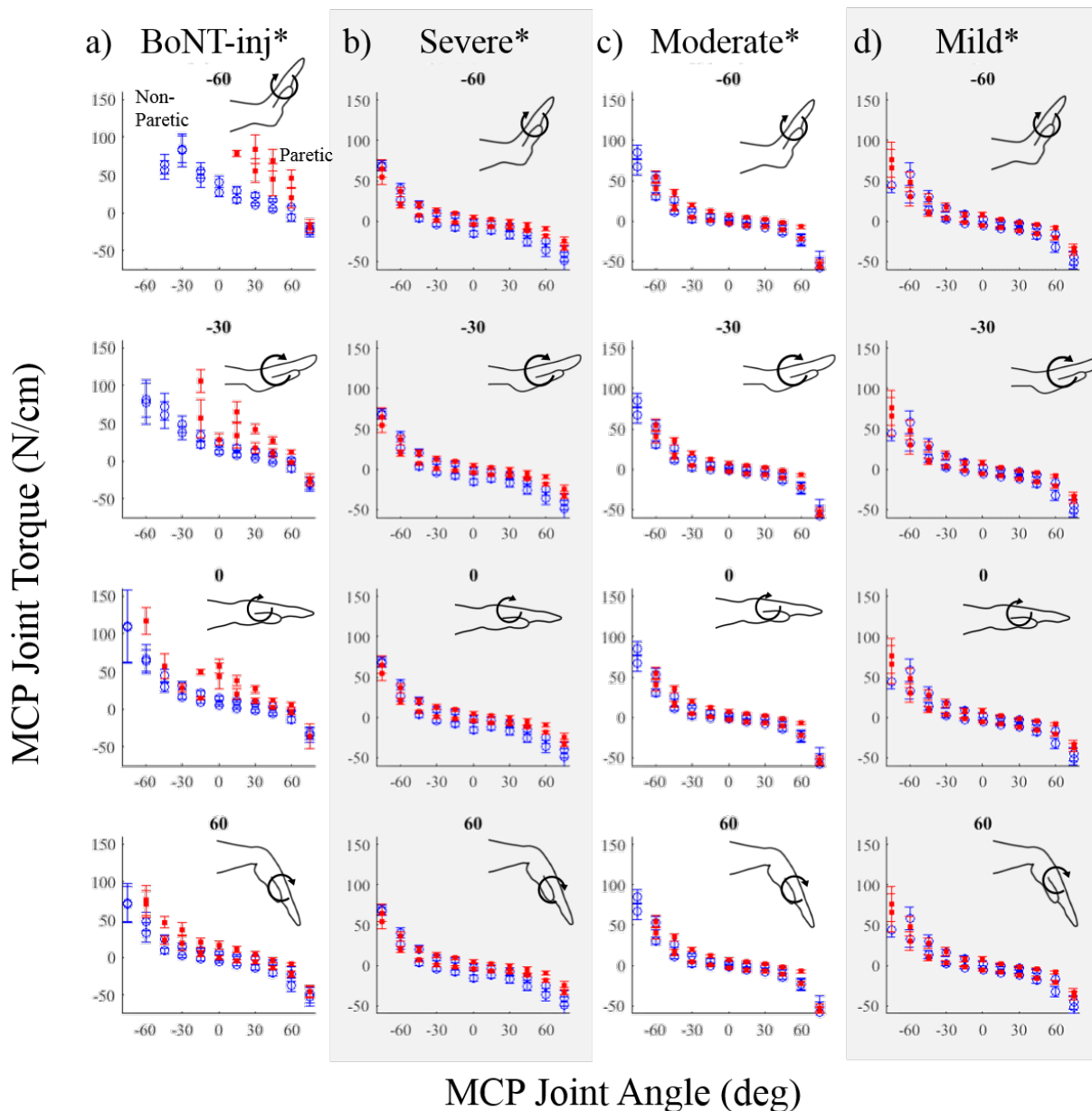
Figure 2: Metacarpophalangeal (MCP) torque data measured in the paretic (red) and non-paretic (blue) limb over the MCP joints' range of motion for the (a) BoNT-injected, and no-BoNT (b) severely, (c) moderately, and (d) mildly impaired groups. The wrist joint was locked in -60 (top row), -30, 0, and 60 degrees flexion (bottom row). Error bars indicate standard error. Negative MCP angles indicate extension, positive indicate flexion. While significant differences ( * denotes p < 0.05 ) in torques measured in paretic vs non-paretic limbs were observed in every group, the only group where finger flexion torque was greater in the paretic hand was the BoNT-injected group, with the effect increasing as the fingers were positioned in an extended posture. Data points are only displayed when there is individual data for 3 or more participants at that specific posture.
