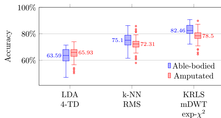
Figure 6: Classification accuracies for able-bodied and amputated subjects when predicting the grasp type with three different types of classifiers.
