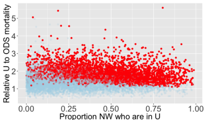
Figure 5: Age-weighting and relative mortality among Model 3 runs. The proportion of normal weight individuals who are unhealthy at the beginning of the simulation is displayed on the x-axis. The relative mortality of unhealthy individuals to obese diabetic ever-smokers ( ODS ) is displayed on the y-axis i.e., if equal to 2, the U mortality rate would be twice of the ODS mortality rate. Parameter sets that resulted in the obesity paradox are in red and sets that did not result in the obesity are in blue. As U mortality becomes substantially higher than ODS mortality, having fewer individuals starting in U is sufficient to counterbalance the higher mortality due to obesity.
