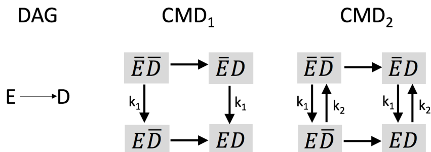
Figure 1: From left to right: A simple DAG showing causality wherein exposure E causes outcome D . Next, in CMD_1 , We will assume that E and D are both dichotomous, so the corresponding CM will have 2^n states (where n = 2 since there are 2 random variables on the DAG). Additionally, D status does not affect E status. The \bar{X} notation denotes not X , so \bar{E} is unexposed. Thus the rates at which individuals become exposed (i.e. go from \bar{E} to E ) are the same whether or not they have D —equal rates are denoted by the same parameter value and if the parameter symbol is not indicated, distinct rates are assumed. This CM is further asserting that once an individual becomes diseased or exposed, they cannot return to the non-diseased or non-exposed state. In CMD_2 , we see that individuals can move from E to \bar{E} , but their D status does not affect the rate at which they transition as indicated by the equal rates between \bar{E}D to \bar{E}\bar{D} and ED to E\bar{D} . Both CMD_1 and CMD_2 would be considered corresponding with the given DAG.
