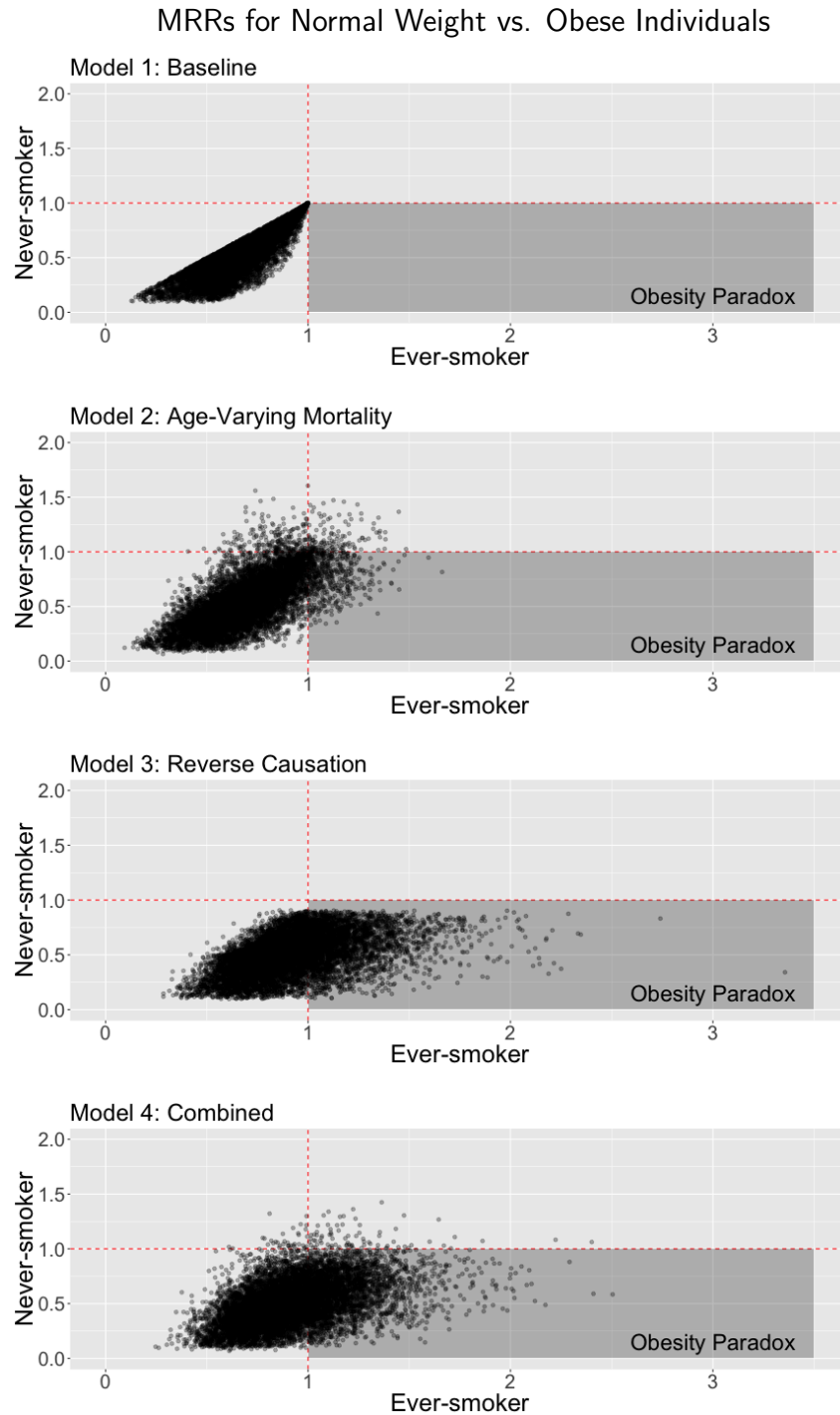
Figure 3: Results from all model runs and parameter sets. Each plot represents the MRR (mortality rate ratio) comparing normal weight individuals to obese individuals for never-smokers against the corresponding MRR for ever-smokers for each of the 10,000 LH-sampled parameter sets with each point representing a single simulated study. The obesity paradox occurs when obese never-smoking diabetics have higher rates of mortality than normal weight never-smoking diabetics and obese ever-smoking diabetics have lower rates of mortality than normal weight ever-smoking diabetics. By row: 1. Preston et al. [6] 2. adding in age-varying mortality rates; 3. reverse causation and 4. combined model.
