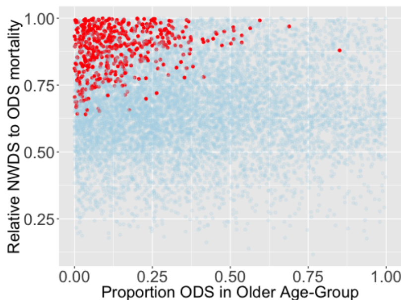
Figure 4: Age-weighting and relative mortality among Model 2 runs. The proportion of obese diabetic ever-smokers ( ODS ) who are old at the beginning of the simulation is displayed on the x-axis e.g., if equal to 0.5, half of the individuals in ODS are in the older age group and half are in the younger age group. The relative mortality of normal diabetic ever-smokers ( NWDS ) to ODS is displayed on the y-axis e.g., if equal to 0.5, the NWDS mortality rate would be half of the ODS mortality rate. Parameter sets that resulted in the obesity paradox are in red and sets that did not result in the obesity are in blue. When NWDS mortality is close to ODS mortality, having ODS be primarily younger can counterbalance the higher mortality due to obesity.
