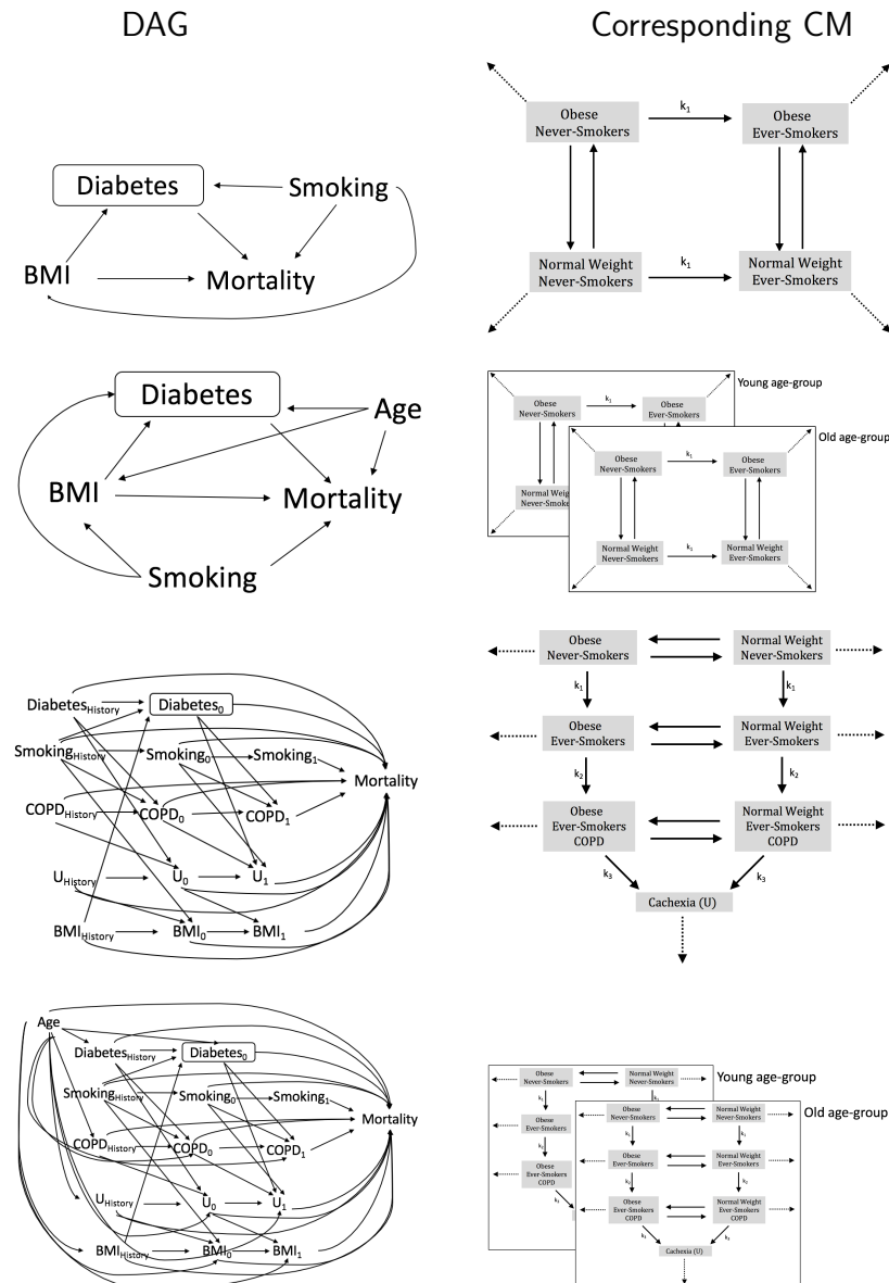
Figure 2: All DAGs and corresponding CMs used in our obesity paradox simulation study. DAGs (left column) and corresponding CMs (right column) for each model. By row: 1. Preston et al. [6] DAG; 2. adding in age-varying mortality rates; 3. reverse causation, and 4. combined model. In the DAGs, ‘BMI’ is the exposure and ‘Mortality’ is the outcome. ‘Age’ and ‘Smoking’ confound the relation between ‘BMI’ and ‘Mortality’. The box around ‘Diabetes’ indicates that the study population is conditioned on individuals with diabetes. Cachexia is represented by ‘U’, and ‘COPD’ is chronic obstructive pulmonary disease. With respect to the longitudinal DAGs, ‘History’ denotes status before the study, ‘0’ denotes baseline, and ‘1’ represents the end of the study i.e., one year follow up. In the CMs, mortality rates are denoted by dotted lines. Rates with no labels (including mortality rates) may all be distinct.
