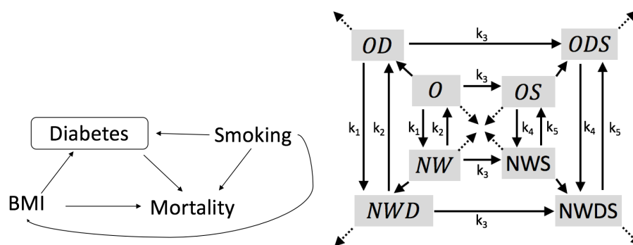
Figure S2: (left) DAG representing the obesity paradox from Preston et al. [6] (right) CM: Schematic of the single age group compartmental model diagram corresponding to the DAG. NW represents normal weight individuals; O represents obesity; D represents diabetes, and S represents smoking. Individuals in any given compartment can die. Each arrow represents flows between states and rates that are equal to each other have the parameter. For instance, diabetes status does not affect the rate at which an individual transitions from obese to normal weight, therefore OD to NWD and O to NW have the same rate. We specify where transition rates are the same between compartments by labeling the model schematic accordingly and using the same parameter to represent equal rates in the equations. Mortality rates are denoted by dotted lines. Rates with no labels (including mortality rates) may all be distinct.
