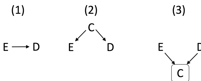
Figure S1: The sources of association between variables become evident on a DAG. E is the exposure, D is the outcome or disease, and C is the covariate (1) cause and effect, (2) common causes or confounding, and (3) common effect or collider bias e.g. selection bias.
