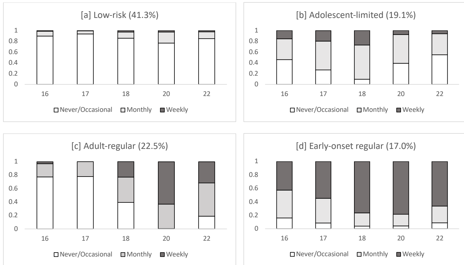
Figure 1. Distribution of binge drinking response across latent classes at each timepoint ( n=6,888 ). Class proportions based on estimated posterior probability 1
