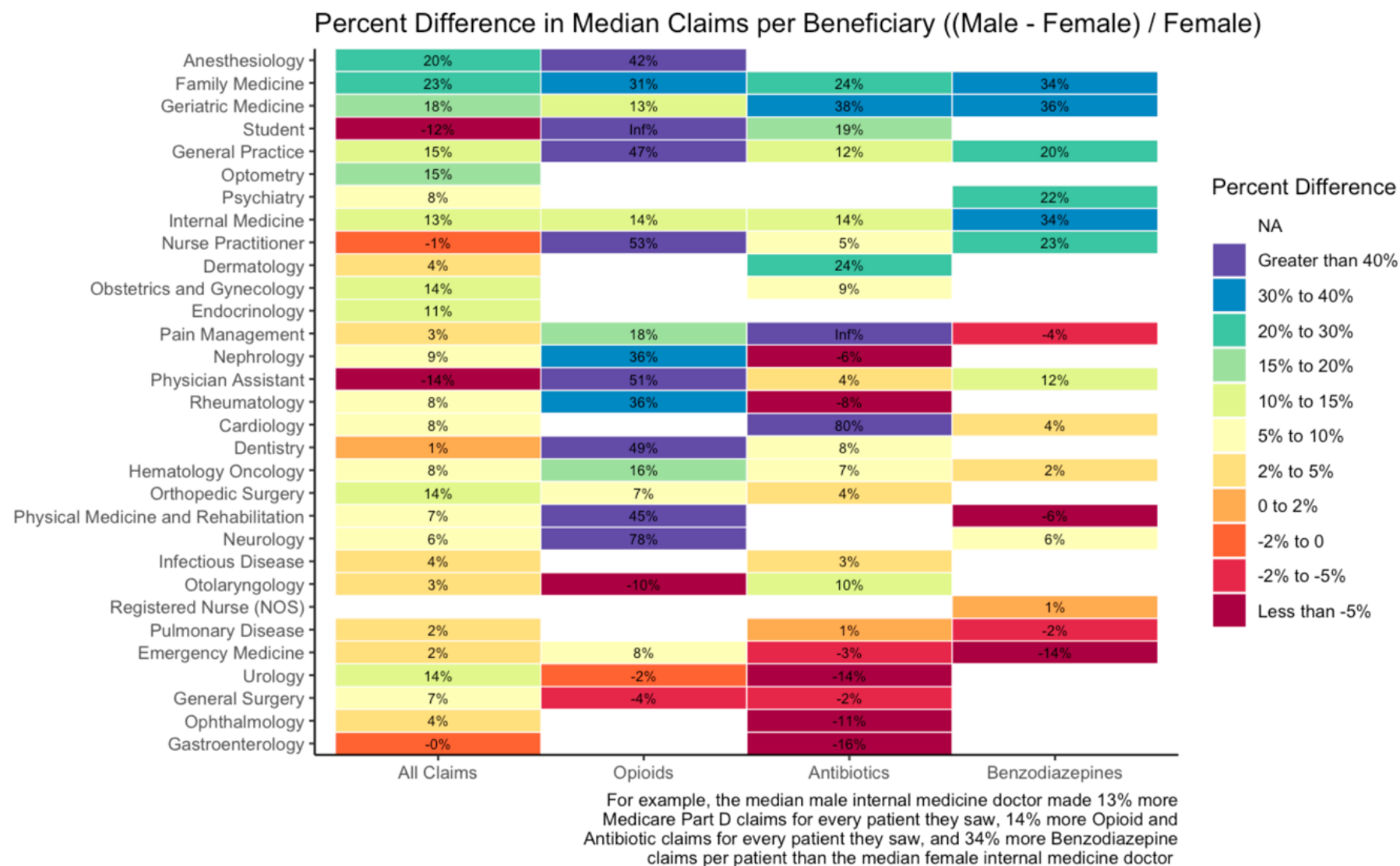
Figure 2: Percent difference of male and female providers' median drug cost, and Medicare Part D beneficiaries.
