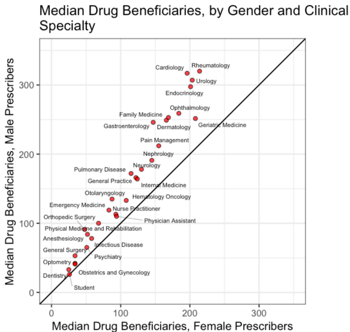
Figure 7: Provider median drug beneficiaries, by gender and specialty.
