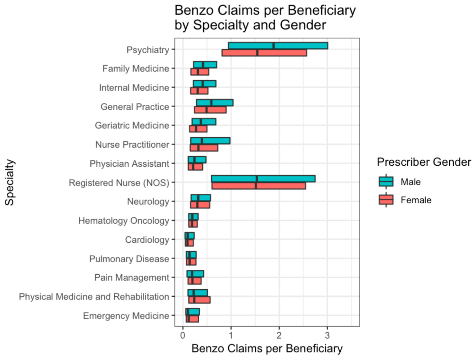
Figure 5: Distribution of provider benzodiazepine prescribing per beneficiary by specialty and gender.
