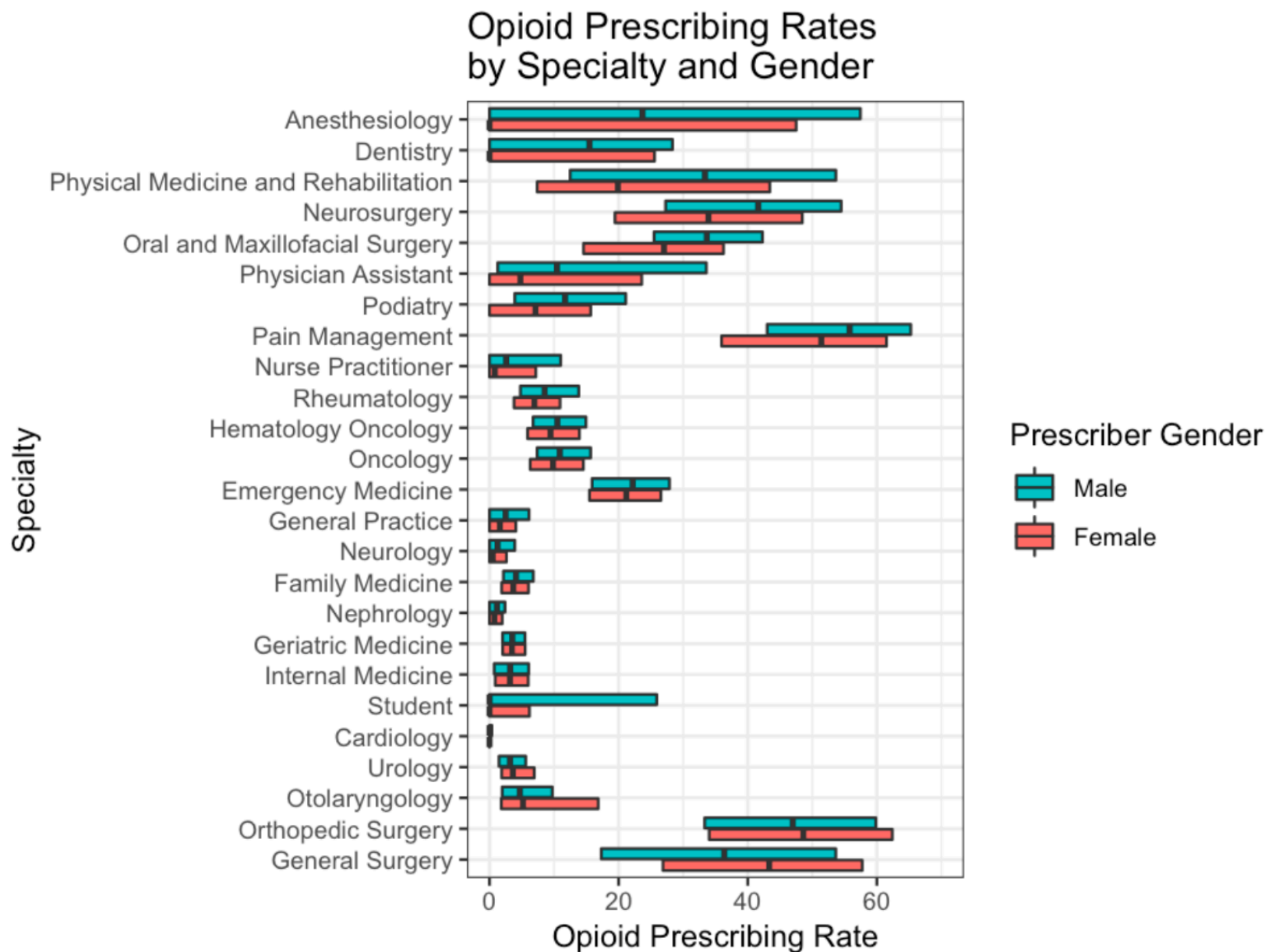
Figure 4: Distribution of provider opioid prescribing rates by specialty and gender.
