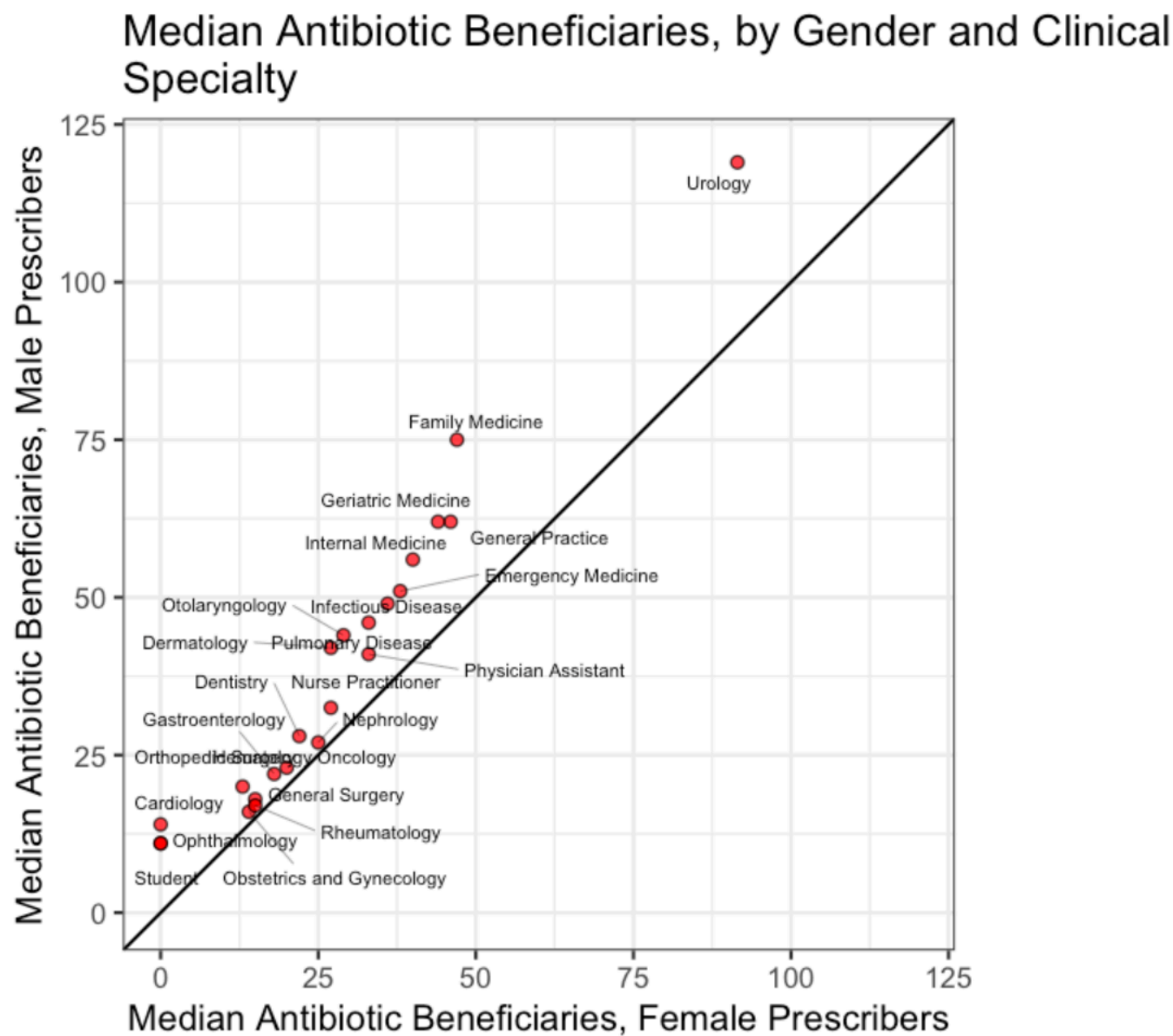
Figure 9: Provider median antibiotic beneficiaries, by gender and specialty.
