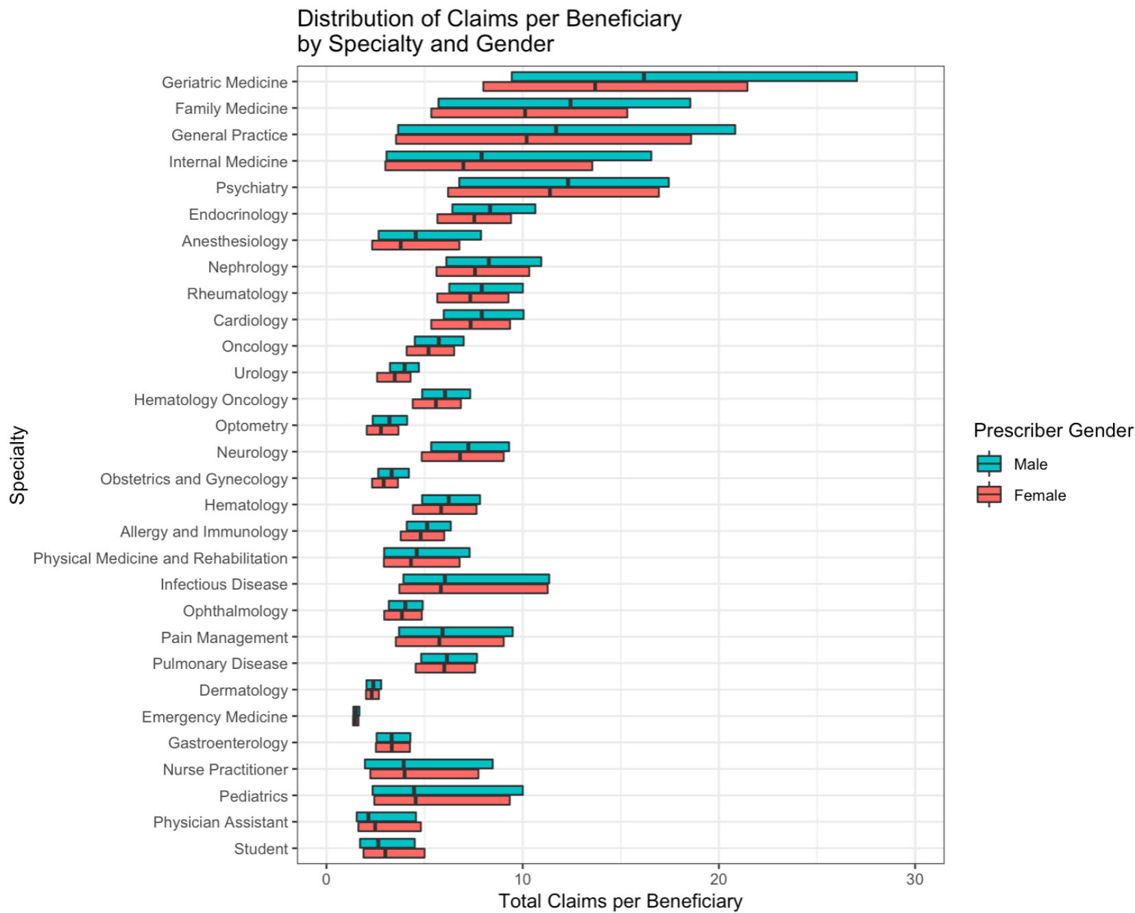
Figure 3: Distribution of provider prescribing of drugs per beneficiary by specialty and gender.
