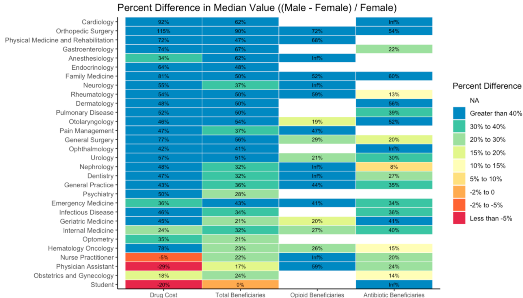
Figure 1: Percent difference of male and female providers' median drug cost, and Medicare Part D beneficiaries.
