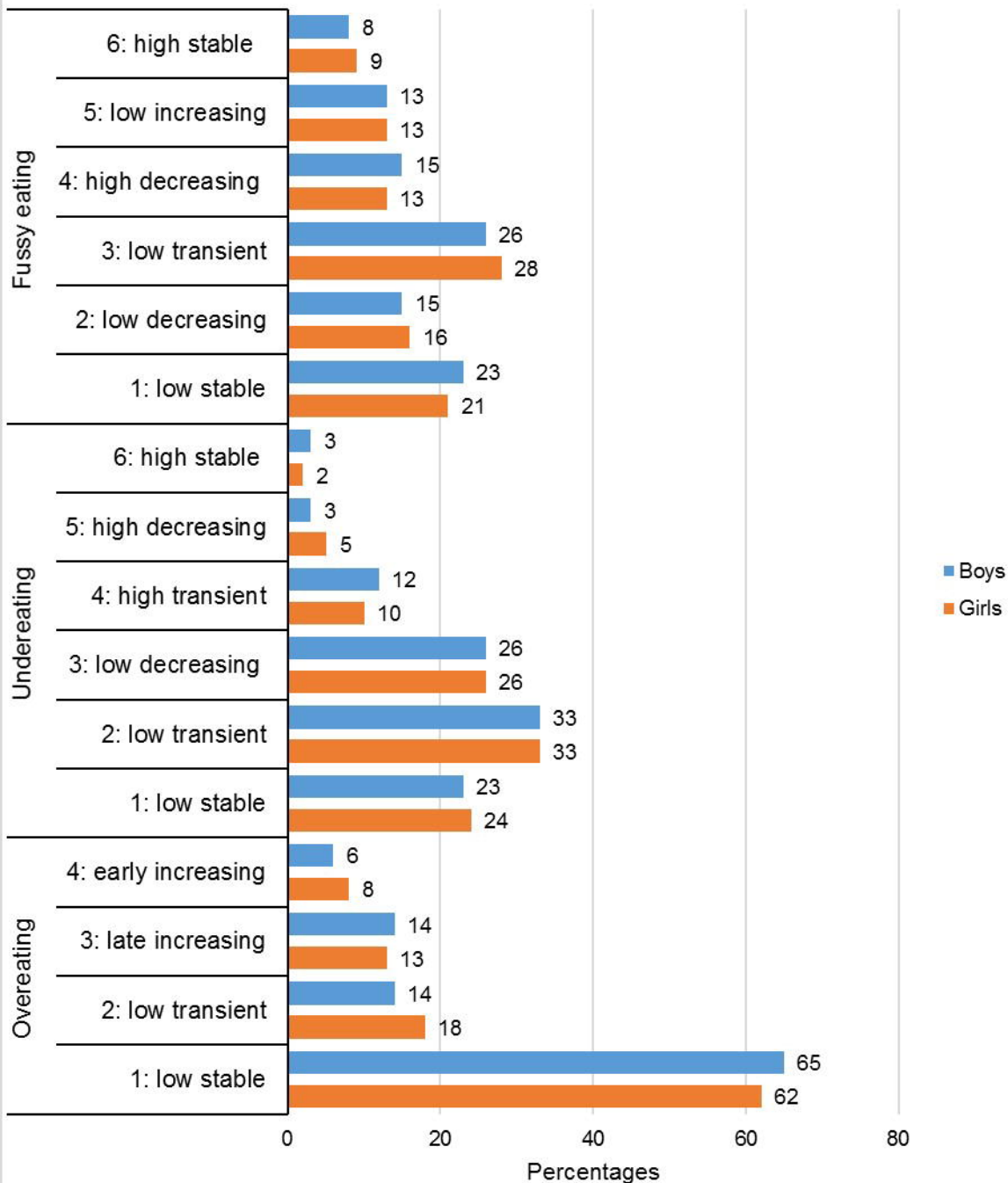
Figure 2: Assigned classes of overeating, undereating and fussy eating using posterior probabilities
