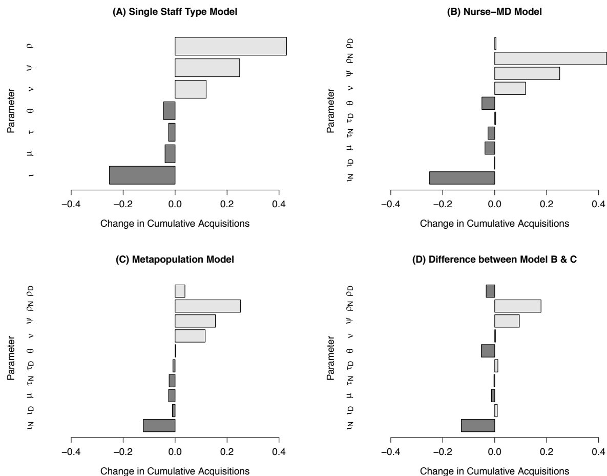
498 499 Figure 5. Global parameter sensitivity of three modeled ICU population structures. 500 Panel A depicts the change in proportional change in cumulative MRSA acquisitions per 501 one-percent change in the value of a specific parameter, with light bars indicating 502 increased acquisitions, and dark bars indicating decreased acquisitions for a model 503 assuming random mixing and with a single staff type for both nurses and physicians. 504 Panel B depicts the same for a model that separates nurses and physicians in to 505 different staff types, while Panel C depicts the same for a metapopulation model where 506 nurses were assigned to a strict subpopulation of patients. Panel D depicts the 507 difference in proportional changes between the Metapopulation and Nurse-MD models. 508
