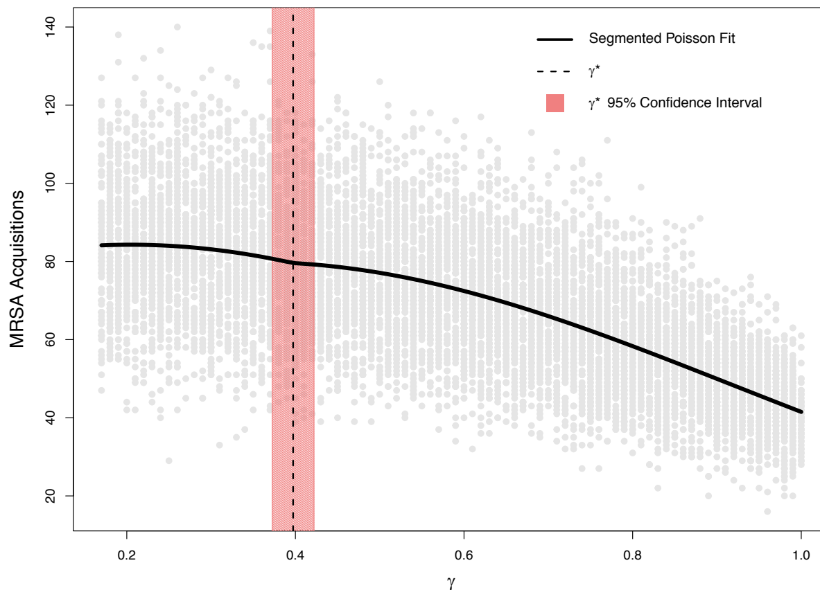
509 510 Figure 6. Relationship between the proportion of time nurses spend treating patients 511 outside their assigned group ( \gamma ) and cumulative MRSA acquisitions over 10,000 512 simulations, randomly sampling \gamma from a uniform distribution between 1/6 and 1. Grey 513 dots show an individual simulation, while the black line shows a segmented Poisson 514 regression fit with linear and quadratic terms for \gamma . The vertical dashed line depicts the 515 single segmentation point, \gamma^* , to the left of which these more complicated models are 516 adequately approximated by the Nurse-MD model where random mixing occurs. The 517 shaded area shows the corresponding confidence interval. 518
