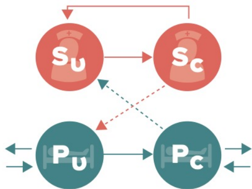
470 471 Figure 1. Schematic representation of the compartmental flow of a mathematical model 472 of methicillin-resistant Staphylococcus aureus (MRSA) acquisition with a single type of 473 staff. Solid arrows indicate possible transition states, while dashed arrows indicate 474 potential routes of MRSA contamination or colonization. Healthcare staff are classified 475 as uncontaminated ( S_U ) or contaminated ( S_C ), while patients are classified as 476 uncolonized ( P_U ) or colonized ( P_C ). 477
