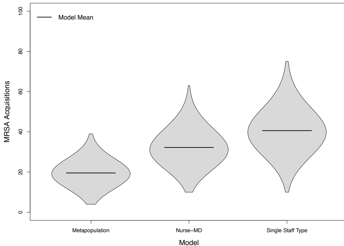
494 495 Figure 4. Distribution of cumulative MRSA acquisitions in 3,000 simulated 18-bed 496 intensive care units under three theoretical population structures. 497
