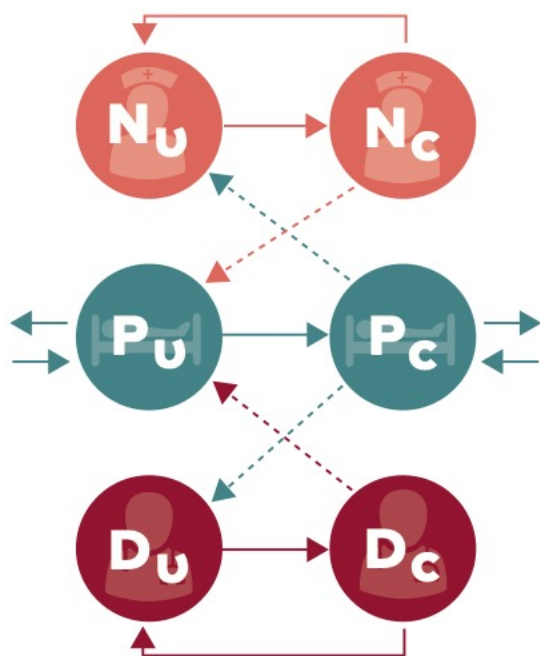
478 479 Figure 2. Schematic representation of the compartmental flow of a mathematical model 480 of methicillin-resistant Staphylococcus aureus (MRSA) acquisition with nurses and 481 intensivists separated into different staff types. Solid arrows indicate possible transition 482 states, while dashed arrows indicate potential routes of MRSA contamination or 483 colonization. Nurses and doctors are classified as uncontaminated ( N_U or D_U ) and 484 contaminated ( N_C and D_C ), while patients are classified as uncolonized ( P_U ) or 485 colonized ( P_C ). 486 487 488
