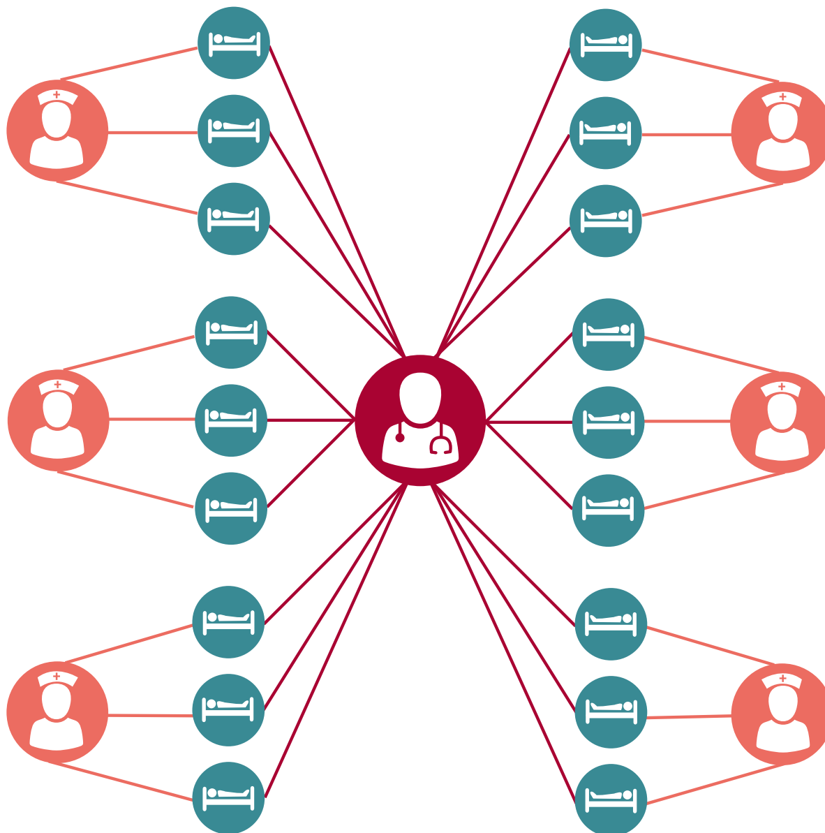
489 490 Figure 3. Schematic representation of a Metapopulation model of methicillin-resistant 491 Staphylococcus aureus (MRSA) acquisition. Patients (blue) are treated by a single 492 assigned nurse (orange). A single intensivist (red) randomly treats all patients. 493
