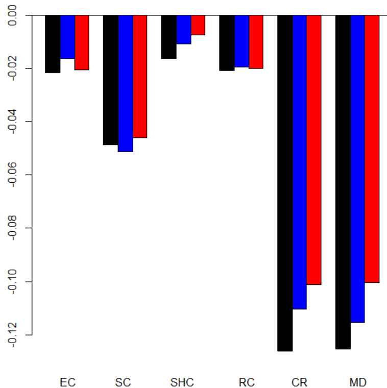
Figure 6: Smoothing effects on response coefficients
