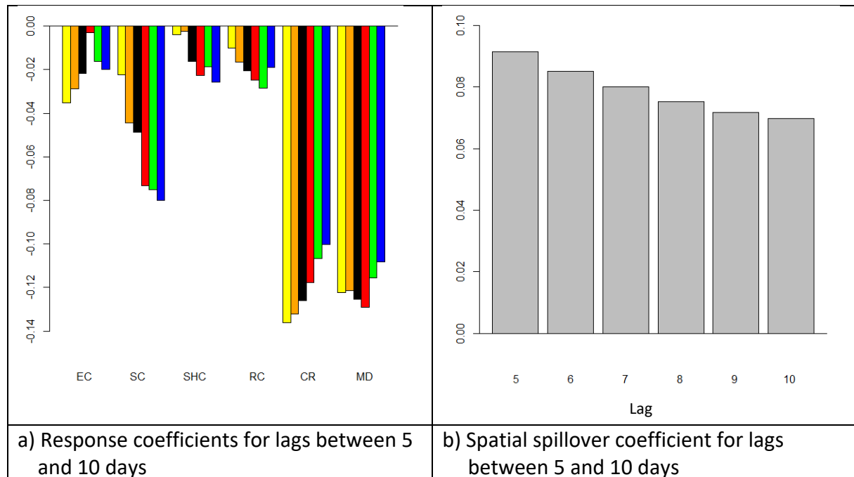
Figure 5: Comparison of response and spillover coefficients for varying lags
