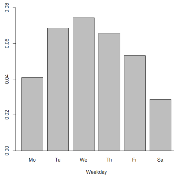
Figure 8: Day of the week effect
