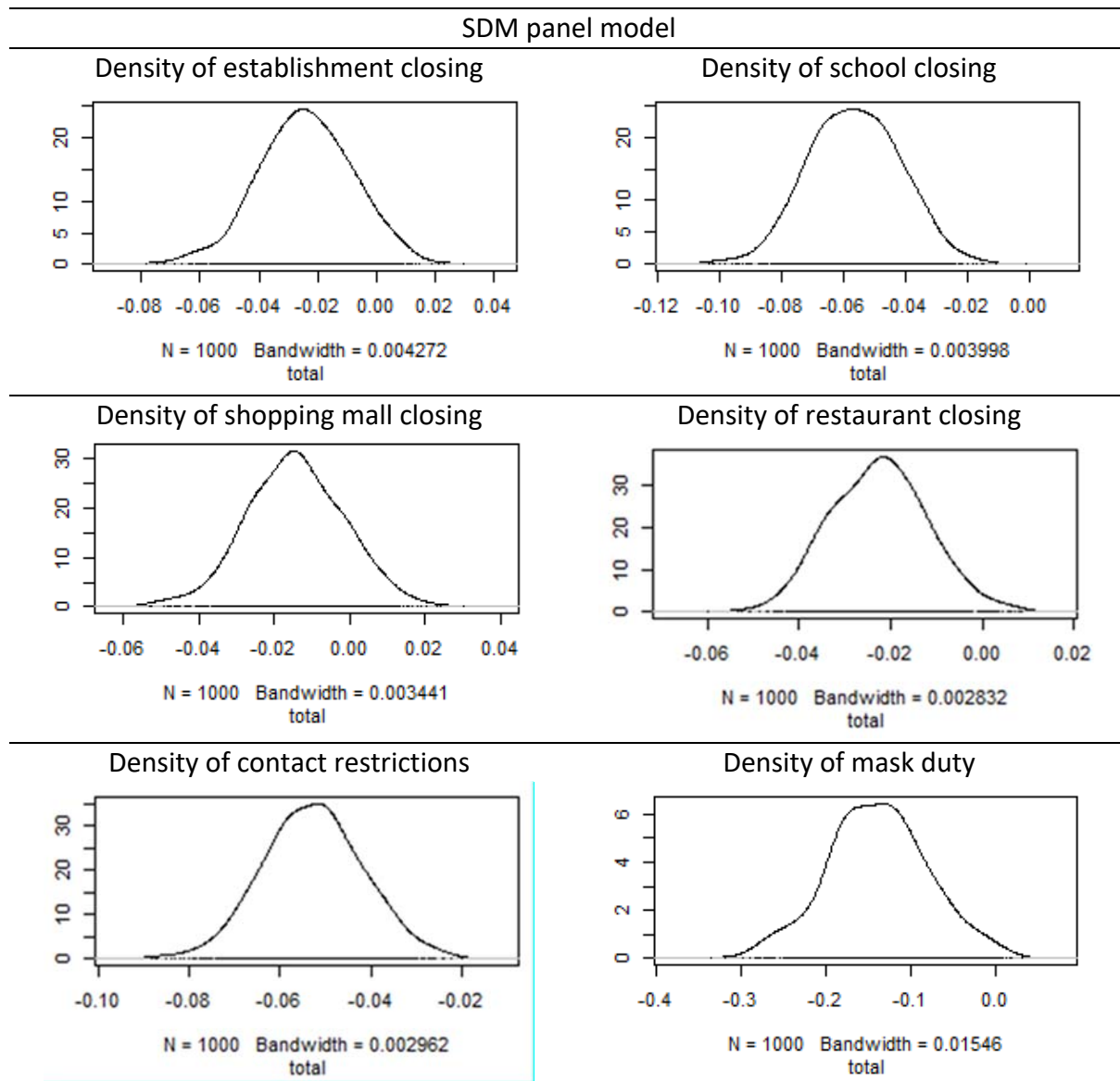
Figure 2: Density plots for total impacts of public health measures
