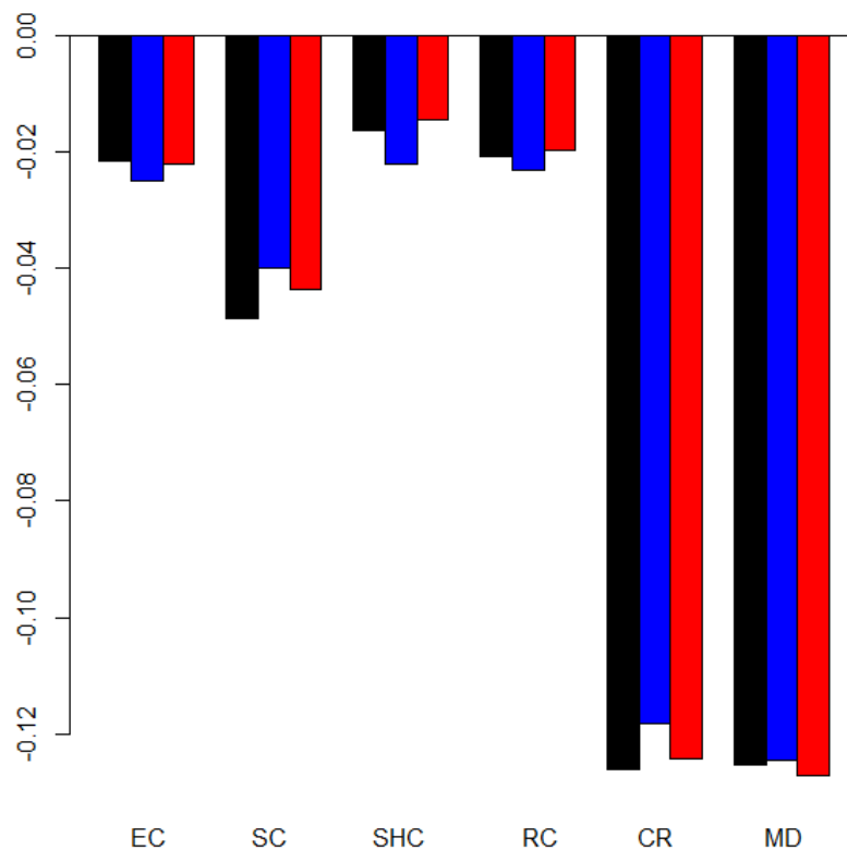
Figure 4: Comparison of response coefficients of SDM, SAR and GNS models
