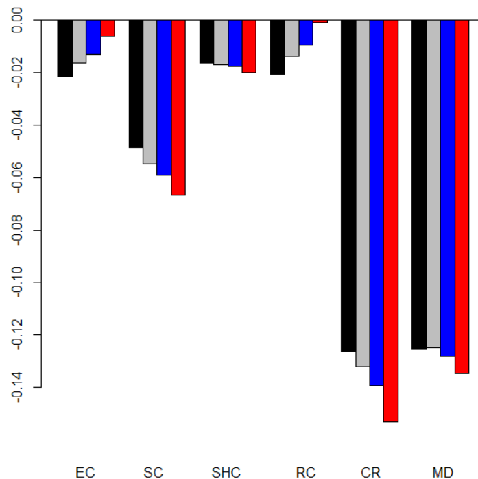
Figure 7: Comparison of response coefficients for different spatial weights matrices
