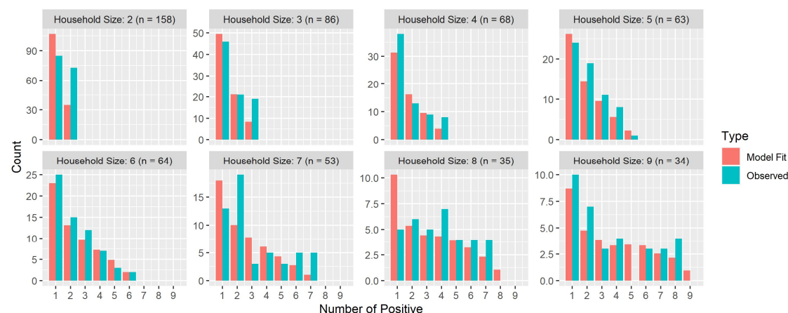
Figure 7: Best model fit to the observed data in the Bnei Brak data set, aggregated according to the household size (fit to households of size greater than or equal to 10 are not shown).
