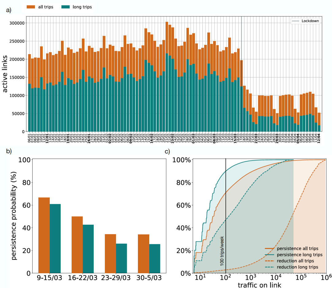
Figure 5. Network analysis. a) Number of mobility connections between French locations over time. b) Link persistence probability: probability that a connection present during week February 3-9 is still present in one of the four selected weeks: before lockdown (March 9-15), during enforcement (March 16-22), during lockdown (March 23-29, March 30 – April 5). c) Persistence probability and traffic reduction in relation with traffic. For a given x-axis value (traffic on link), solid lines measure the fraction of broken links which used to have at most that weight in the baseline week. Dashed lines report the fraction of missing traffic that was
