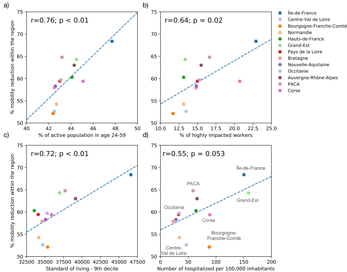
Figure S1. Reduction in internal mobility for the week April 6-12, 2020 vs. epidemic, socio-economic, and demographic indicators. The following plot is the equivalent of Figure 4 for internal mobility. Correlation is evaluated between outgoing traffic and the four considered indicators: a) the population in active age (24-59 years old), b) the fraction of employees in the sectors mostly affected by lockdown, c) the 90 th percentile of the regional standard of living. Pearson correlation coefficients and their p-values are reported, d) the cumulated number of COVID-19 hospitalizations per 100,000 inhabitants on April 05, 2020.
