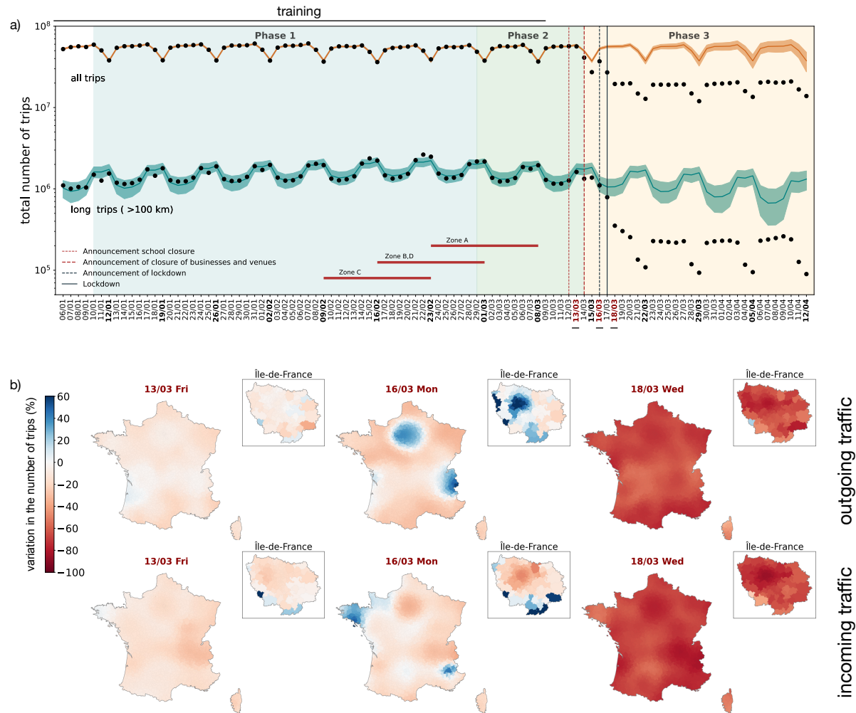
Figure 1. The phases of the COVID-19 epidemic in France, and its impact on mobility patterns.
