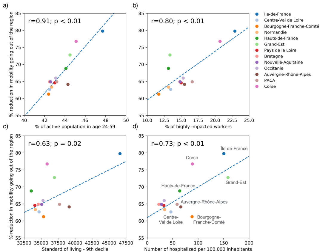
Figure 4. Reduction in outgoing mobility for the week April 6-12, 2020 vs. epidemic, socio-economic, and demographic indicators. Correlation is evaluated between outgoing traffic and the four considered indicators: a) the population in active age (24-59 years old), b) the fraction of employees in the sectors mostly affected by lockdown. c) the 90 th percentile of the regional standard of living 23 , d) the cumulated number of COVID-19 hospitalizations per 100,000 inhabitants on April 05, 2020. Pearson correlation coefficients and their p-values are reported.
