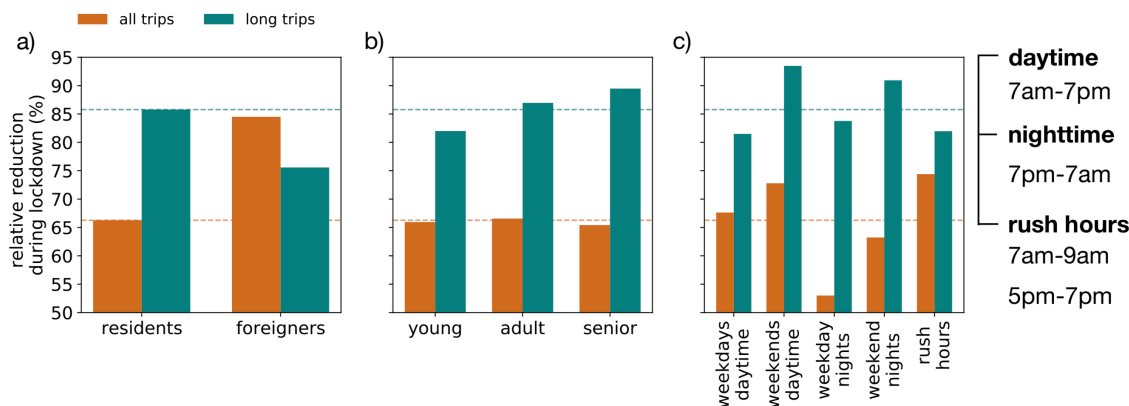
Figure 2. Mobility reduction during lockdown across user type, age and time of day. Reduction is computed as the average over the week starting Monday April 6, with respect to the average over the first week of February (starting Monday February 3). a), b) and c) show the relative reduction broken down by residents/foreigners, age classes, and times of the day. They also show statistics for all trips (orange) and long trips (green), defined as trips with geodesic distance longer than 100 km. Horizontal orange and green lines indicate relative reduction on all residents (all, long, respectively).
