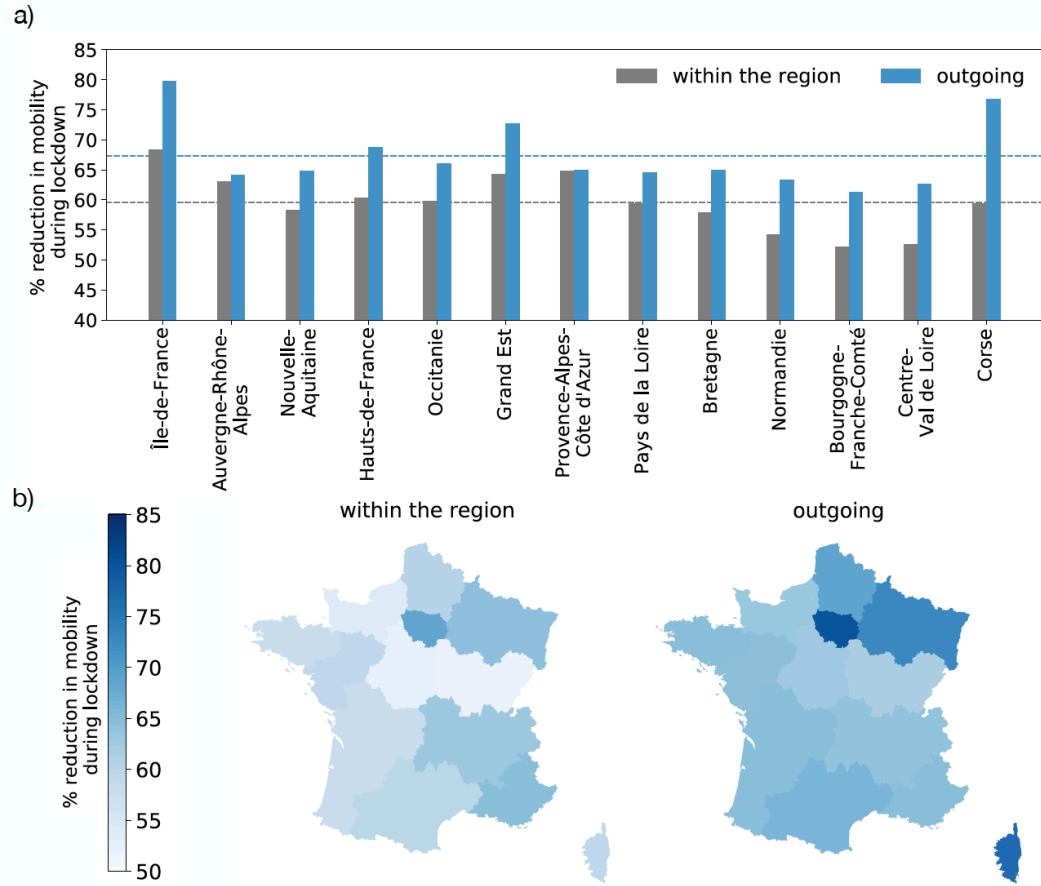
Figure 3. Lockdown-induced mobility reduction across regions. a) Breakdown of mobility reduction by region in mainland France. Reductions for trips within region are in gray, for trips leaving the region are in blue. The horizontal gray and blue lines indicate the corresponding averages across regions. b) Map visualization of a).
