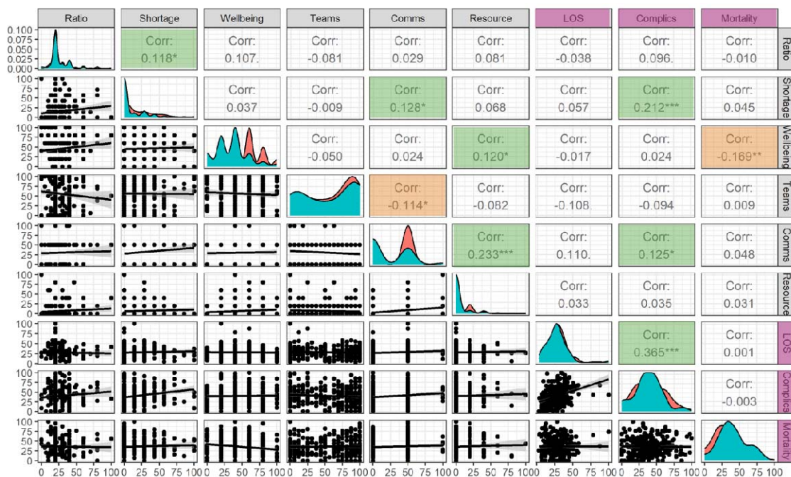
168 Figure 3 Correlation of outcomes with main strain categories. Correlation matrices show the relation between parameters, 169 with the variables displayed across the top and sides of the diagram. The diagonal shows the distribution of the variable in 170 question (2020 in red, 2021 in teal), the upper triangle shows the correlation coefficient by Pearson coefficient, *p<0.05, 171 **p<0.01, ***p<0.001 by Pearson coefficient, significant positive correlations highlighted in green, significant negative 172 correlations highlighted in orange. The lower triangle shows the scatter plot of the two variables to allow visual inspection. 173 NonICU – non-ICU nursing staff recruited into the ICU, Ratio – nursing ratio change in surge times (increased ratio indicating
