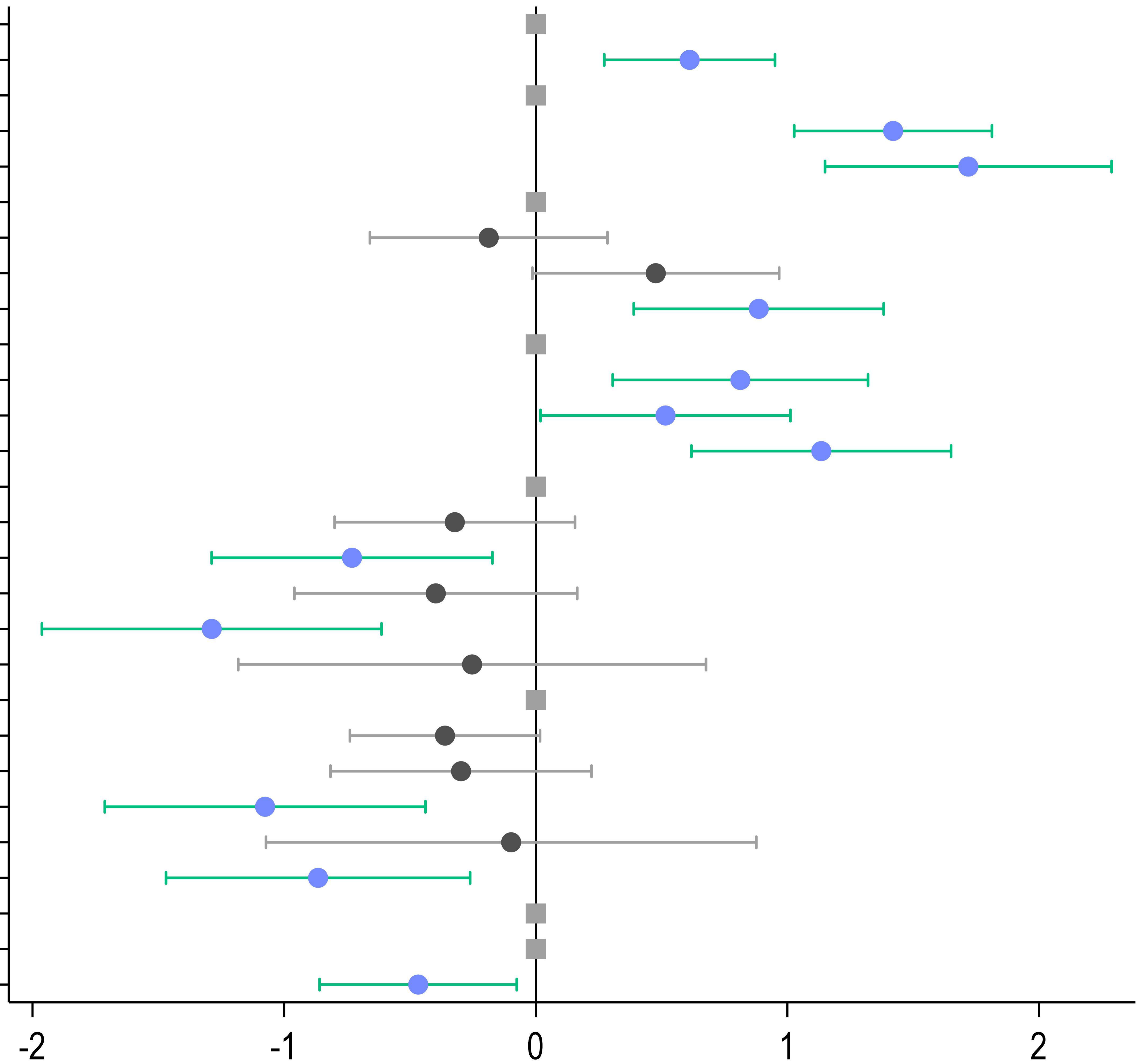
Coefficient estimates and 95% confidence intervals
