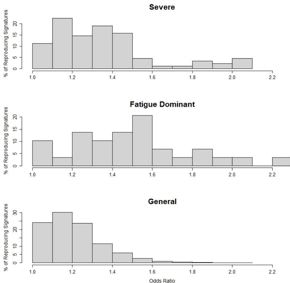
Figure 1. Distribution of observed odds ratios in AoU for reproducing signatures with high case frequencies (>5%)
