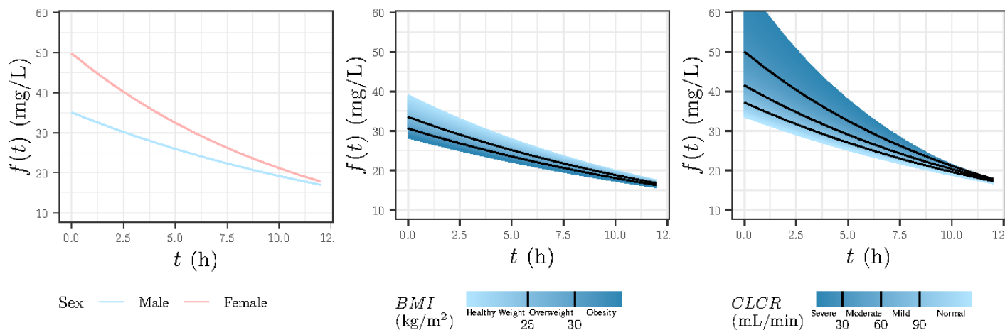
Figure 1: Evolution of the concentration f(t) according to the fixed effects in the three univariate scenarios: the first panel corresponds to an effect of SEX on V , the second panel to an effect of BMI on V and the third panel to an effect of CLCR on Cl . For the second and third panels, the black lines correspond to the limits of the intervals of the continuous covariates.
