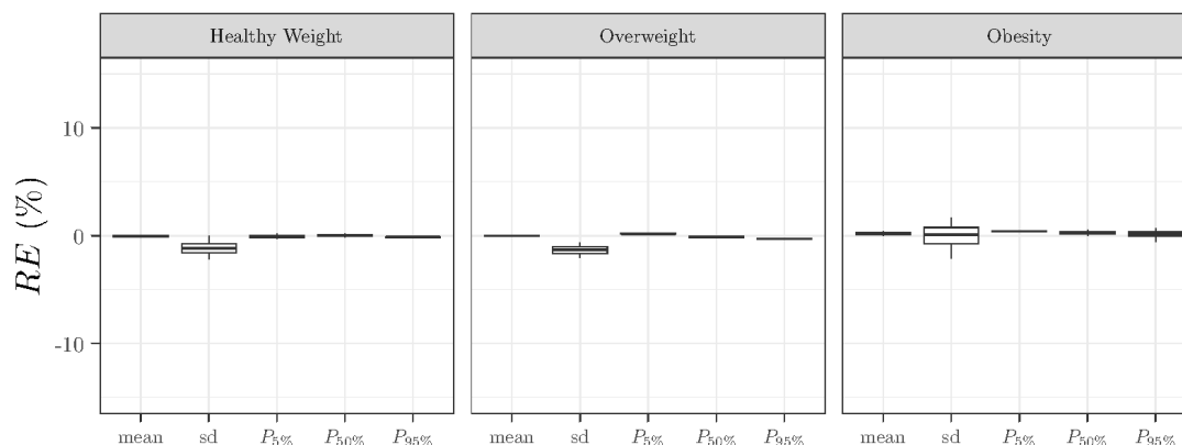
Figure A.1.1: BMI only - Relative error ( RE ) of distribution metrics (mean, standard deviation and percentiles) of BMI for the three intervals, as compared to the statistics of the NHANES database. For each BMI interval, the virtual population was simulated 100 times from the copula.
