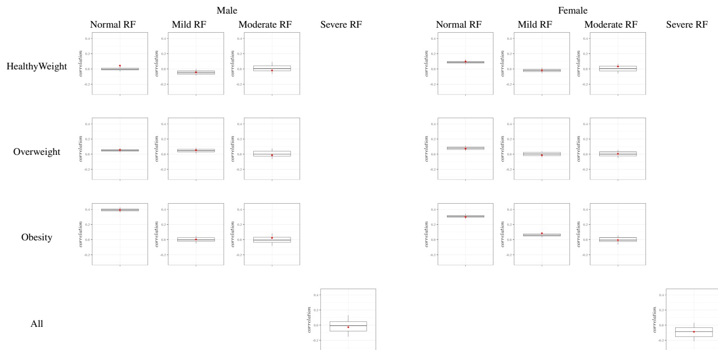
Figure A.1.7: Three Covariates - Correlations of \log BMI and \log CLCR pair in the NHANES database (red diamond) and in virtual population relative simulated 100 times from the copula (boxplot).
