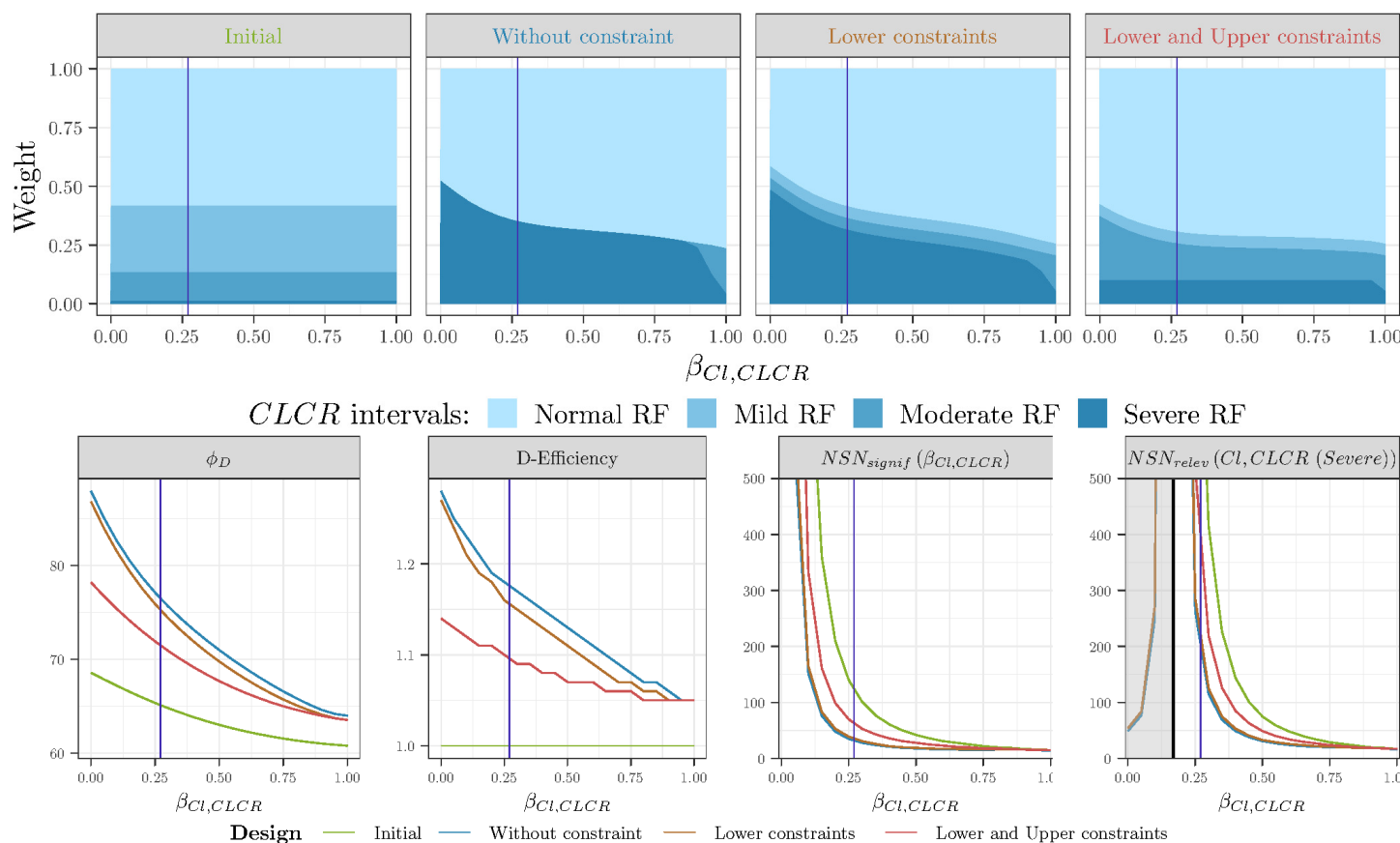
Figure 6: CLCR only - Optimal proportions for the covariate distributions for the D-criterion (top), \phi_D , D-Efficiency and NSN to reach 80% power (bottom), as a function of \beta_{CI,CLCR}
