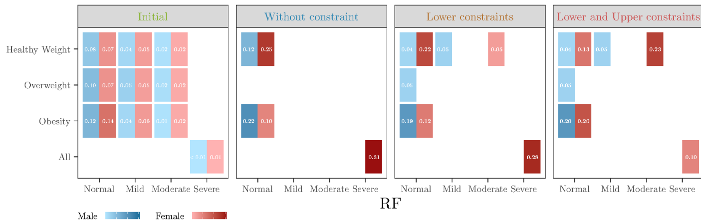
Figure 7: Three Covariates - Optimal proportions for the covariate distributions for the D-criterion for the different sets of constraints
