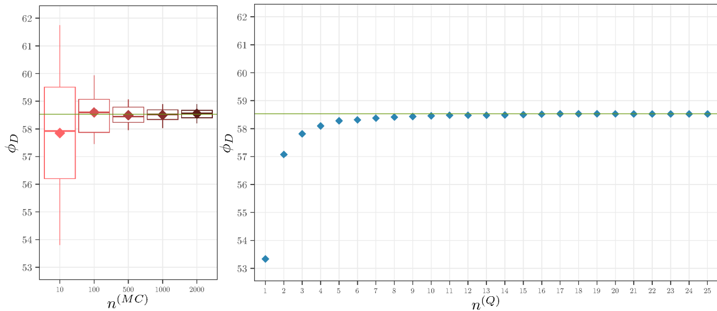
Figure A.2.1: BMI only - \phi_D computation with FIM integration using copula and MC (left) and copula and GLQ (right).
