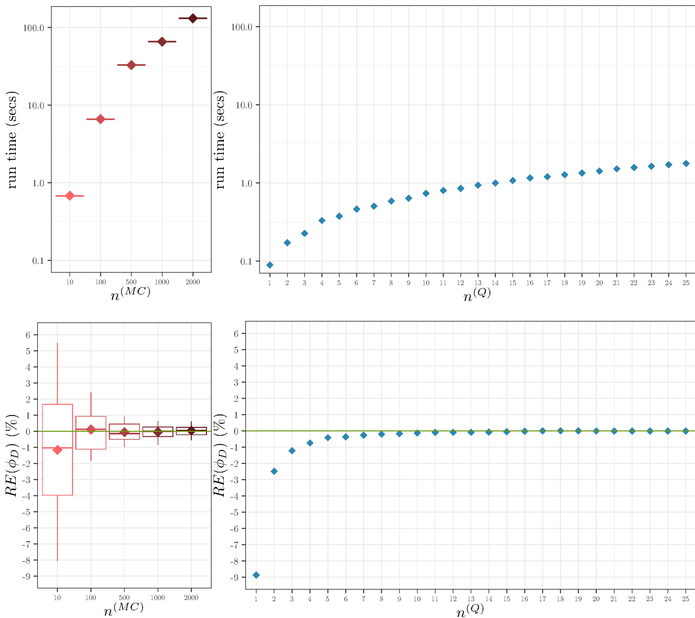
Figure 3: BMI only - Run time for \phi_D computation (top) and relative error ( RE ) in \phi_D computation (bottom), with FIM integration using on the left copula and MC and on the right copula and GLQ. The target value was the average \phi_D obtained with n^{(MC)} = 1000 and n^{(MC)} = 2000 .
