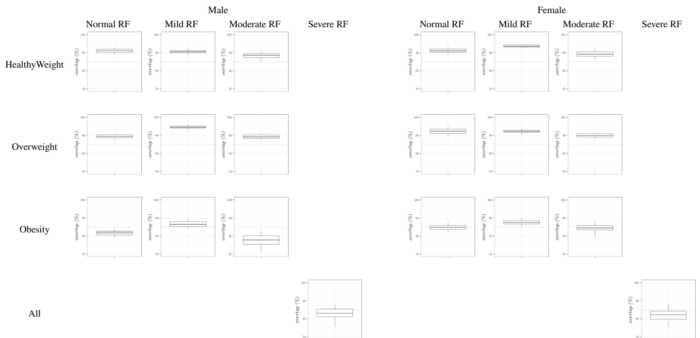
Figure A.1.6: Three Covariates - Overlap metric of 95 th density contours of virtual population relative simulated 100 times from the copula to the NHANES database.
