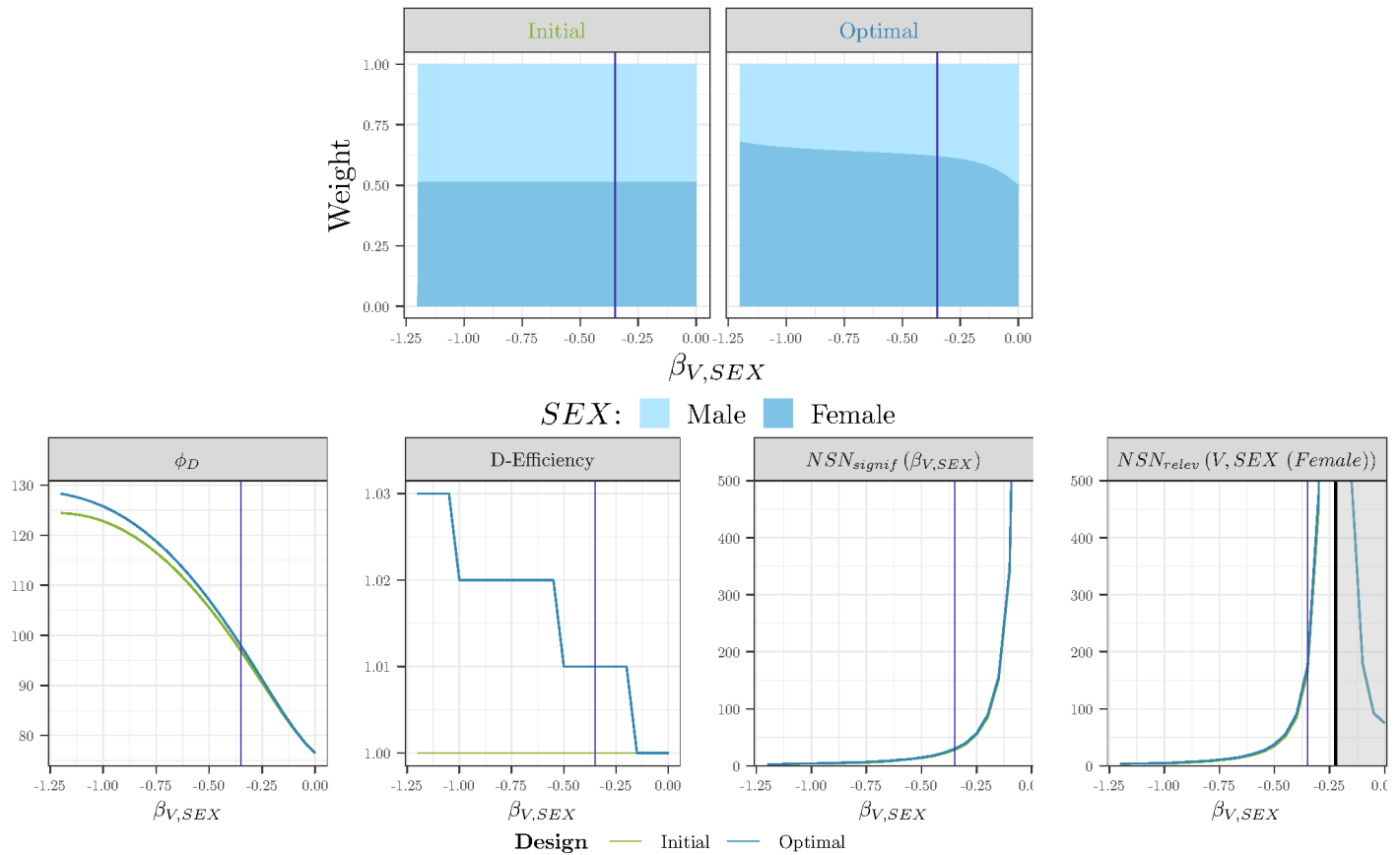
Figure 4: SEX only - Optimal proportions for the covariate distributions for the D-criterion (top), \phi_D , D-Efficiency and NSN to reach 80% power (bottom), as a function of \beta_{V,SEX}
