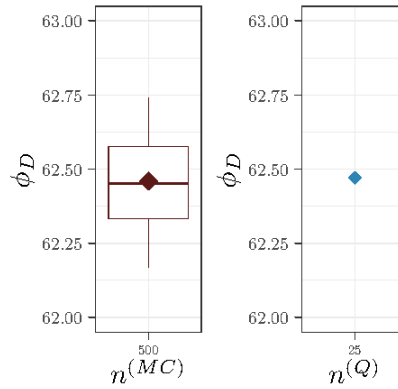
Figure A.2.4: Three covariates - \phi_D with FIM integration using copula and MC (left) and copula and GLQ (right).
