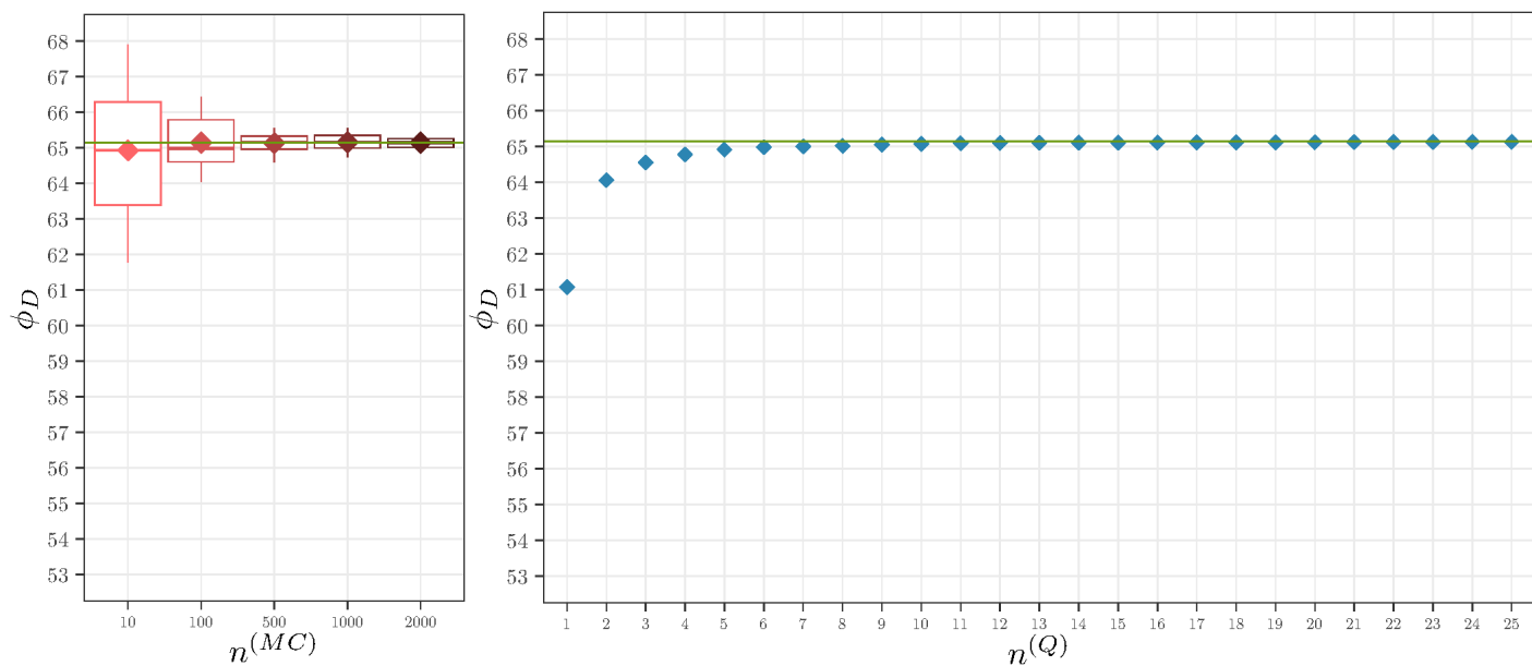
Figure A.2.2: CLCR only - \phi_D computation with FIM integration using copula and MC (left) and copula and GLQ (right).
