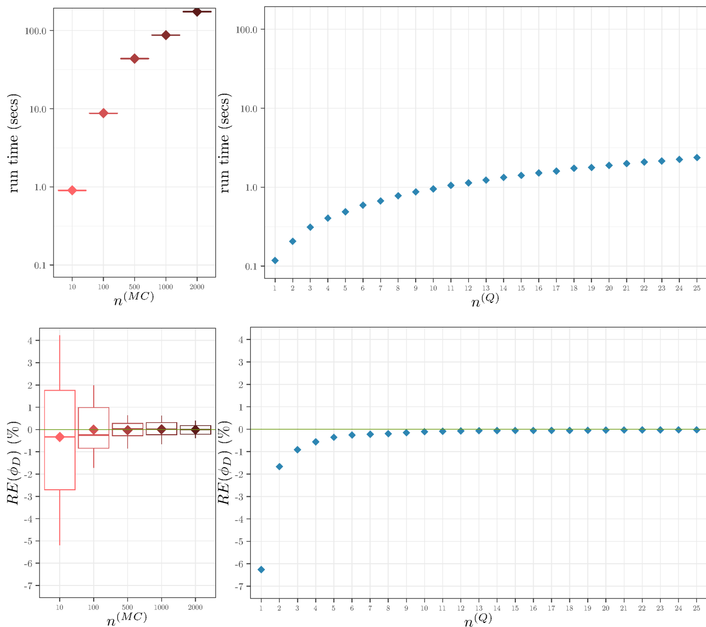
Figure A.2.3: CLCR only - Run time for \phi_D computation (top) and relative error ( RE ) in \phi_D computation (bottom), with FIM integration using on the left copula and MC and on the right copula and GLQ. The target value was the average \phi_D obtained with n^{(MC)} = 1000 and n^{(MC)} = 2000 .
