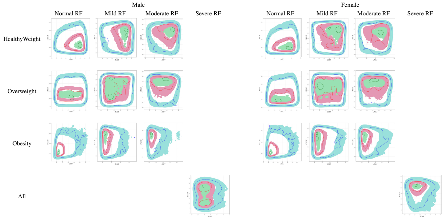
Figure 2: Three Covariates - Visual predictive checks based on the contours of the bivariate density between BMI and CLCR . For each of the 20 covariate combination, the virtual population was simulated 100 times from the copula and the 99% prediction intervals of percentile contours of the joint distribution was derived and compared to the contours observed in the NHANES database.
