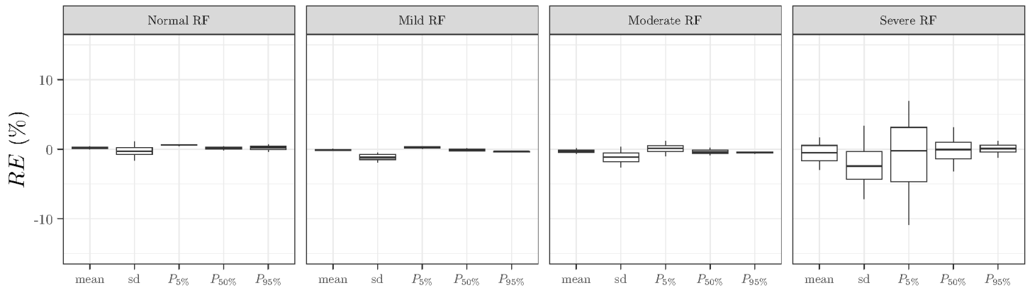
Figure A.1.3: CLCR only - Relative error ( RE ) of distribution metrics (mean, standard deviation and percentiles) of CLCR for the four intervals, as compared to the statistics of the NHANES database. For each CLCR interval, the virtual population was simulated 100 times from the copula.
