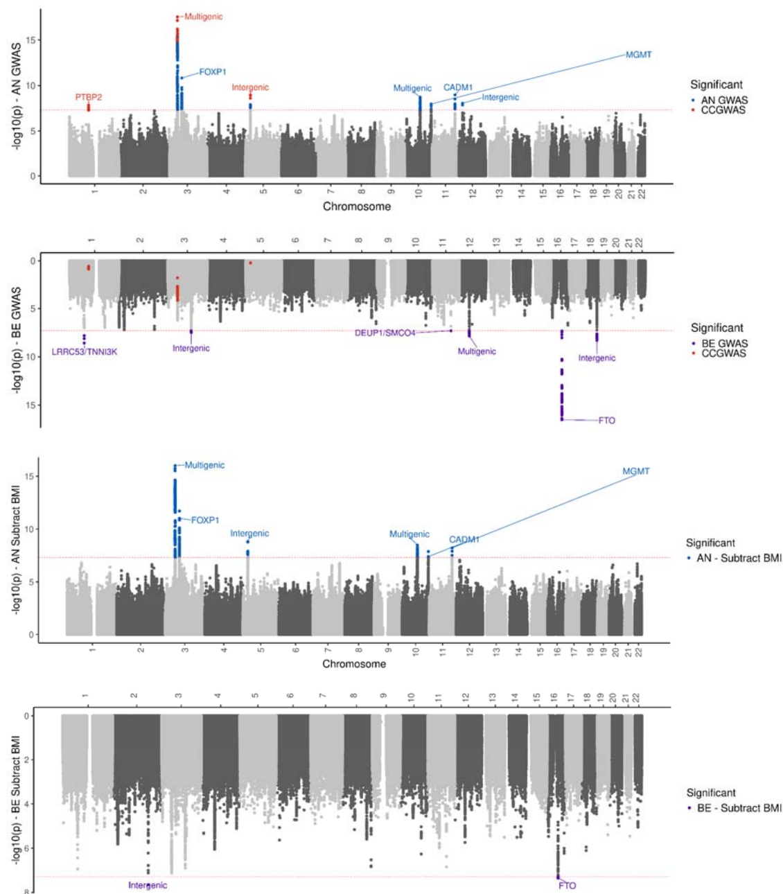
Figure 1: Miami plots showing results from the AN (top) and BE-BROAD (bottom) meta-analyses. The dotted red line is the genome-wide significance threshold ( P \leq 5 \times 10^{-8} ).
