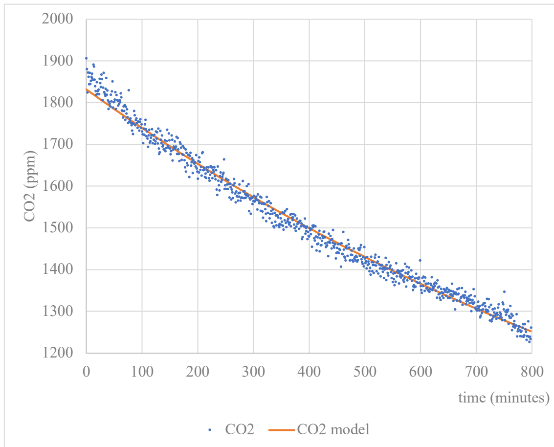
347 348 Figure 4. Model of CO 2 removal in room Ne, a room of 1,040 m 3 with a gauge of 240 (room 349 emptied after use, all doors and windows closed) during one night (800 minutes). r = 0.994 . 350 Renewal rate = 0.04 volume/h. Clean air flow per occupant at 100% occupancy = 0.2 351 m 3 /h/occupant (< 1% of the regulatory floor).
