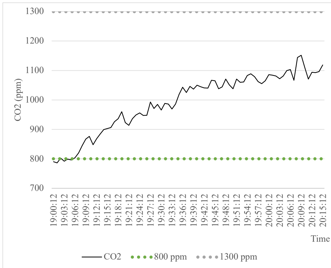
Figure 3. Typical CO 2 profile in room Ta, a room of 1,360 m 3 occupied by 95 people for a gauge of 300 (32% occupancy). 3 rd quartile of CO 2 = 1071 ppm. Clean air flow during session = 35 m 3 /h/occupant. Clean air flow at 100% occupancy = 11 m 3 /h/occupant. Percentage of gauge reduction required to meet legal airflow of 25 m 3 / hour / occupant at 100% occupancy = 55% (78% to reach the 50 m 3 /h/occupant target of HCSP).
