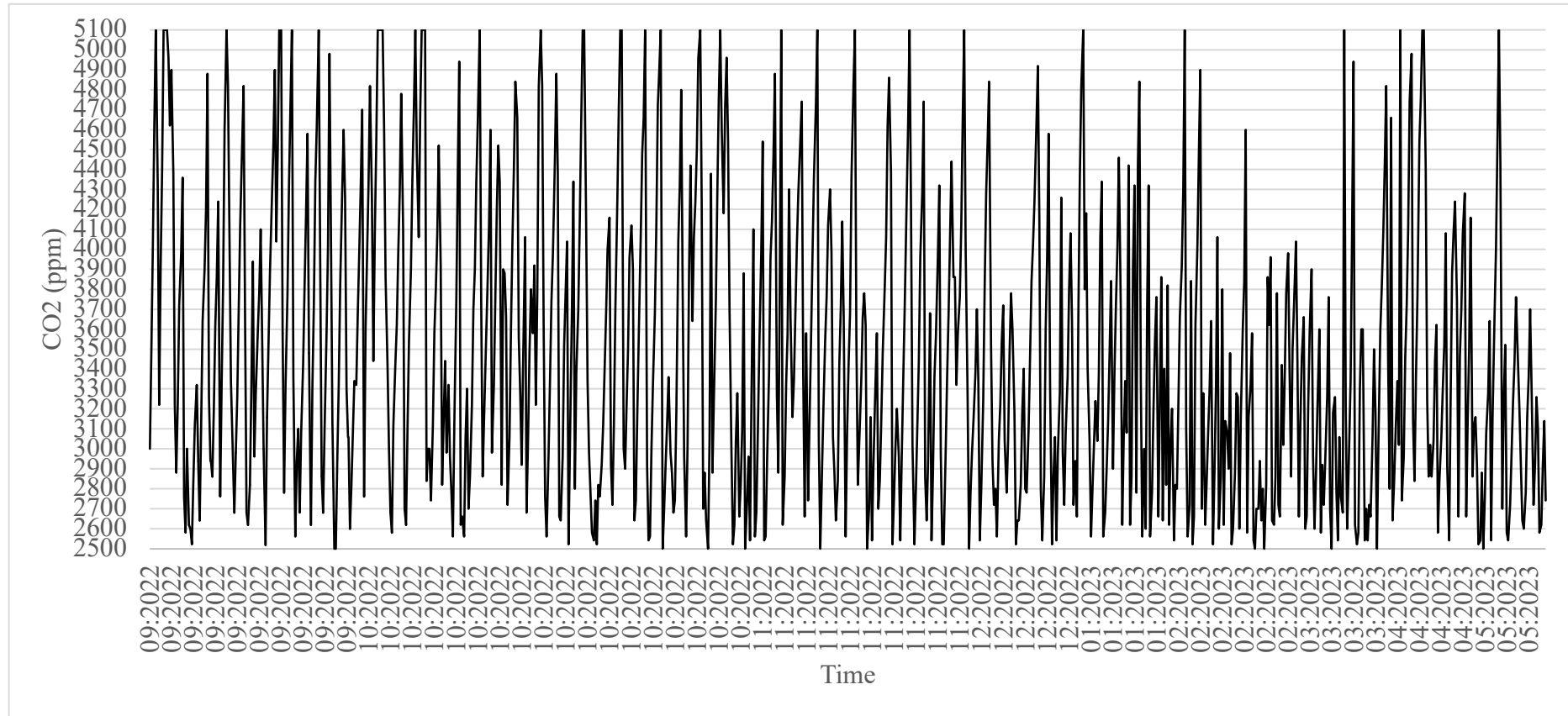
366 Figure 6. 94 CO 2 peaks above 2,500 ppm (28 of which above 5,000 ppm) were observed between September 2022 and June 2023, in one of the 367 23 UGA classroom (out of 101 monitored) where peaks above 5,000 ppm were measured (only values above 2,500 ppm were plotted in this graph). 368 This room has a gauge of 44 occupants, an area of 51.8 m 2 , and a volume of 140 m 3 (3.2 m 3 /occupant).
