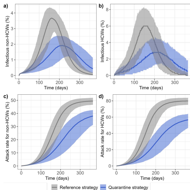
Figure 2: Epidemic curves comparing the reference (grey) and quarantine (blue) strategies. Predicted changes over 365 days in the median and 95% prediction band of the percentage of infectious individuals (I and A compartments) amongst a) non-healthcare workers and b) healthcare workers. Attack rate in c) non-healthcare workers and d) healthcare workers.
