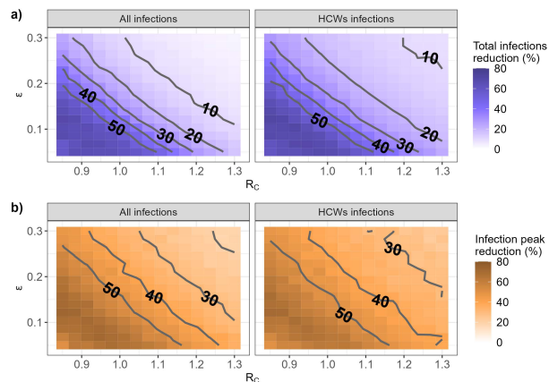
Figure 4: Predicted reduction achieved by the quarantine hospital strategy (as compared with the reference strategy) in (a) the cumulative number of infections over 365 days and (b) the peak incidence, as a function of R_C , the basic reproduction number in the community, and \epsilon , the level of self-isolation non-compliance in symptomatic HCWs.
