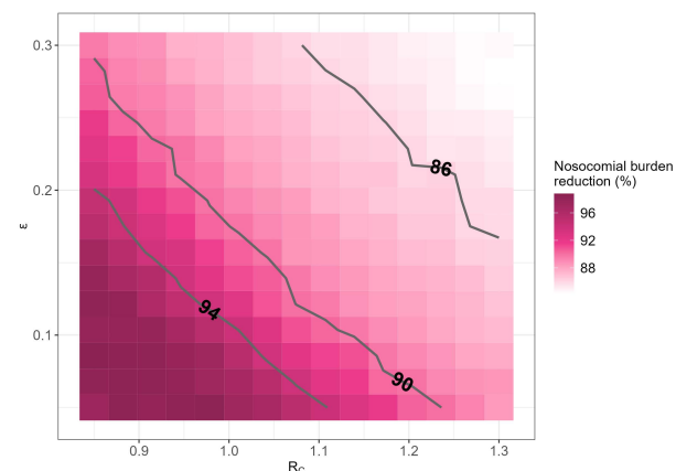
Figure 5: Reduction in the cumulative number of nosocomial acquisitions over 365 days, as a function of assumed values for R_C , the basic reproduction number in the community, and \epsilon , the level of self-isolation non-compliance in symptomatic HCWs.
