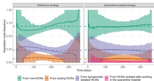
Figure 3: Distribution of acquisition routes over time for non-HCW infections in the community, comparing the reference (left) and the quarantine hospital (right) strategies. Time changes in the median proportion of new infections is depicted over 365 days (solid lines), along with the 95% prediction band (shaded areas), for each route: acquisitions from non-HCWs, from HCWs resting between work shifts, from symptomatic HCWs strictly isolating in the community and, in the quarantine hospital strategy case, from HCWs isolating after a shift in the quarantine hospital. The dashed lines show the median acquisition frequency over the entire 365 days.
