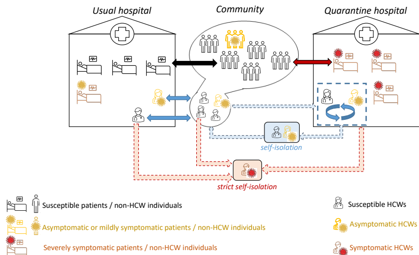
Figure 1: Global model structure: movements of individuals (non-HCWs and HCWs) between the community, quarantine and usual hospitals.
