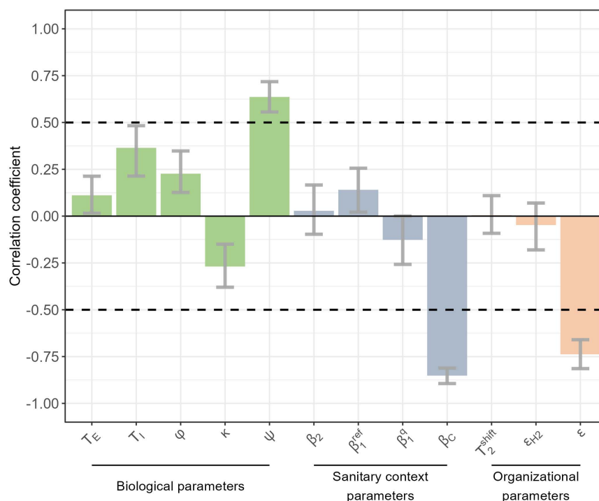
Figure 6: Sensitivity analysis: partial rank correlation coefficients (PRCC) between the predicted reduction in the cumulative number of cases over 365 days and model parameters. Three categories of parameters are explored: biological characteristics of the virus, parameters resulting from the population structure and implemented control measures within the usual hospitals and community ("sanitary context parameters") and parameters describing the implementation of the quarantine hospital strategy ("organizational parameters"). The full list of model parameters is provided in Table 2, along with their baseline values and explored ranges.
