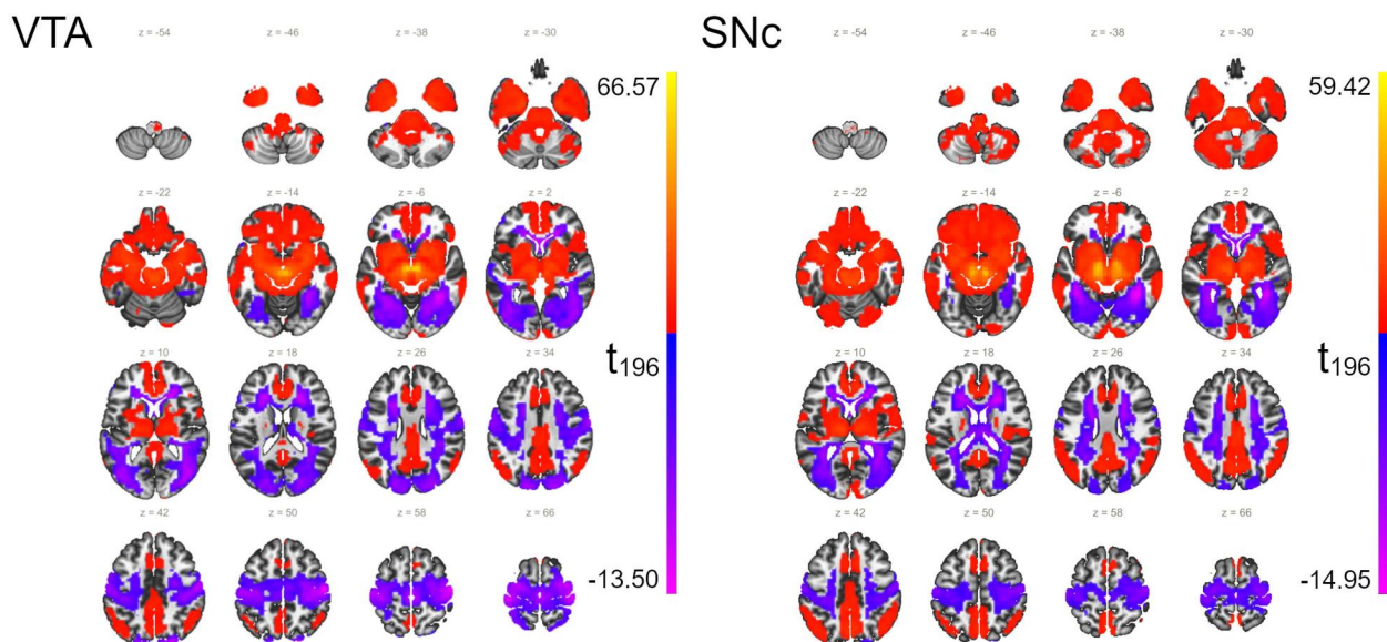
FIGURE 2: Voxel-wise description of VTA (left) and SNc (right) functional networks in CONN. All voxels with significant functional connectivity to the seed ROI over all patients in the sample in a one-sample t-test are highlighted. Please note that the maps describe VTA and SNc networks in the whole cohort rather than between group differences. See supplement for details.
