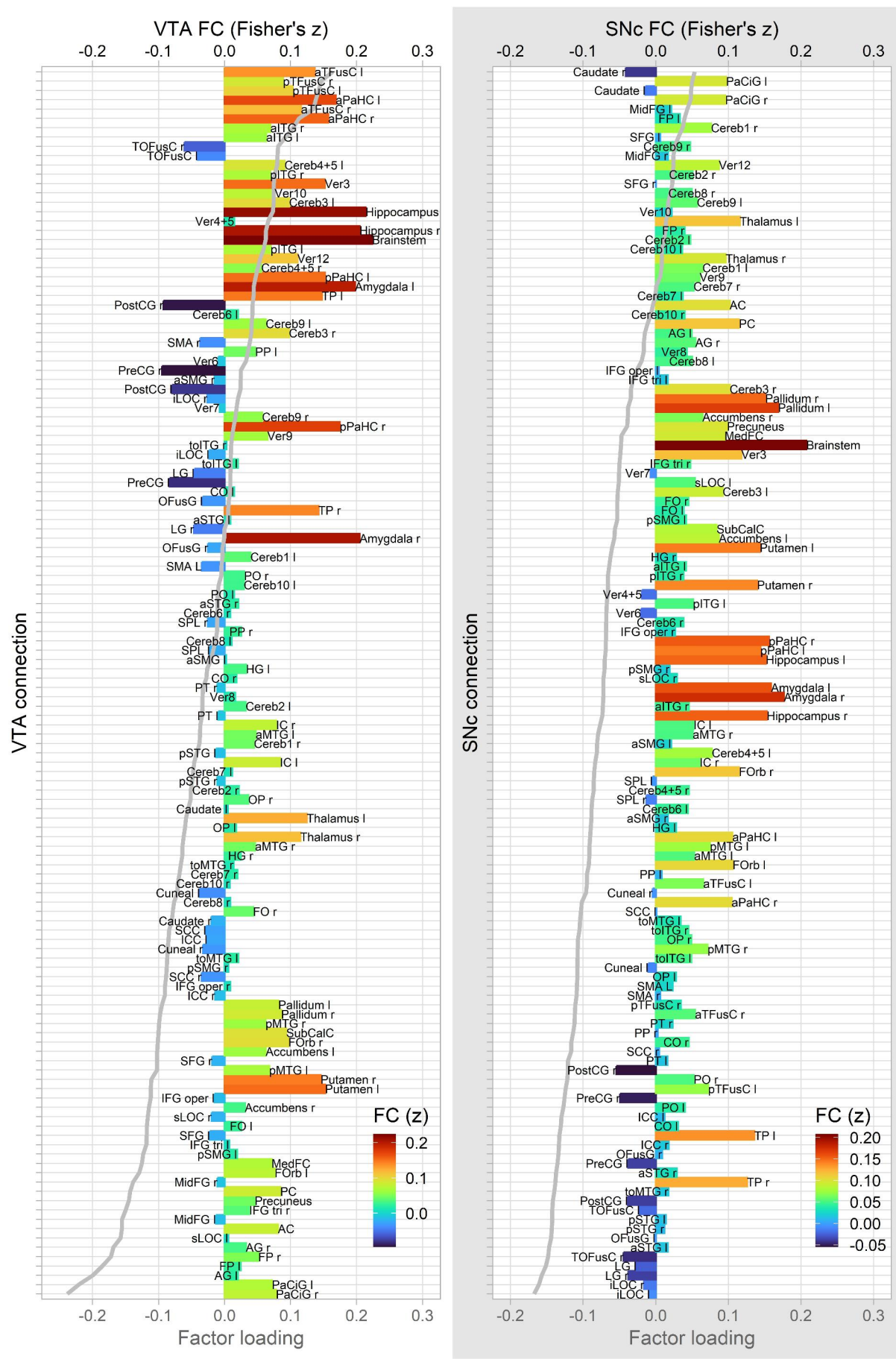
FIGURE 3: Construction of principal components. PC4 for VTA (cognition and spatial processing, left) and PC1 for SNc (sensory perception and processing, right, grey shading) were found to be significantly associated with POCD risk
