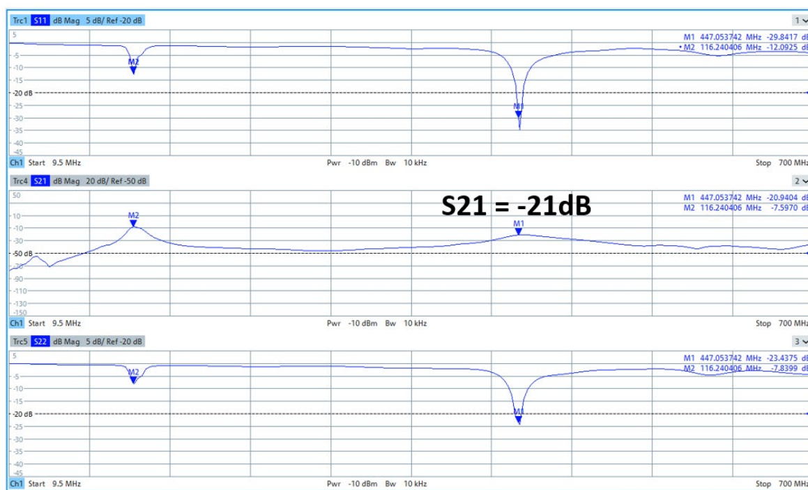
Figure 3. S-parameter measurement of the proposed high impedance microstrip array at 447MHz. The results demonstrate the excellent decoupling performance of the high frequency mode (at 447MHz) while the low frequency mode is weakly coupled. The gap between the coil element is 10mm.
