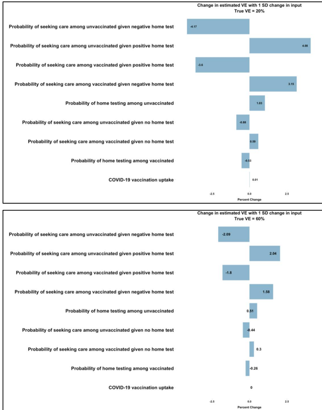
Figure 3: Tornado plot showing the effects of varying parameters on \widehat{VE} . Plots show in rank order the most to least (top-down y-axis) influential parameters that affect estimated \widehat{VE} . Figure 3a (top plot) shows the effect of one standard deviation increase in each parameter on change in \widehat{VE} when true VE is 20%. Figure 3b (bottom plot) shows effects of one standard deviation increase in each parameter on change in \widehat{VE} when true VE is 60%. These values can be interpreted as the percentage point change for each one standard deviation increase in the respective model input.
