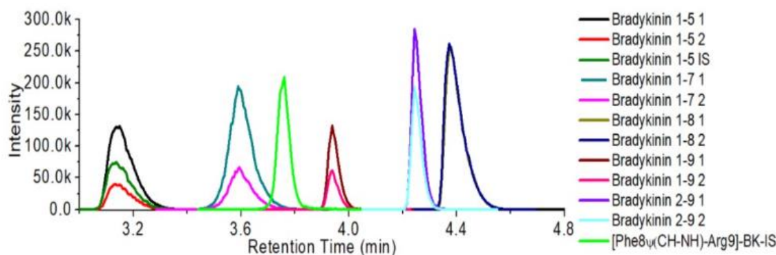
Figure E1. A representative LC-MS/MS chromatogram of Calibrator 3 (0.5 ng/mL for each analyte), illustrating clear separation among all analytes. The signal intensities for all analytes are notably robust, ensuring the reliability and accuracy of our analytical method.
