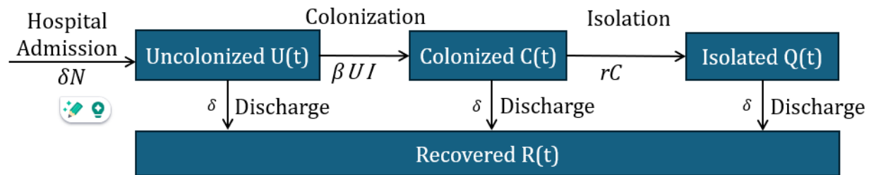
Figure 1: Schematic representation of the Uncolonized-Colonized-Quarantined-Recovered (UCQR) Model. From any compartment, a patient can be discharged, including those MRSA colonized but unidentified.
