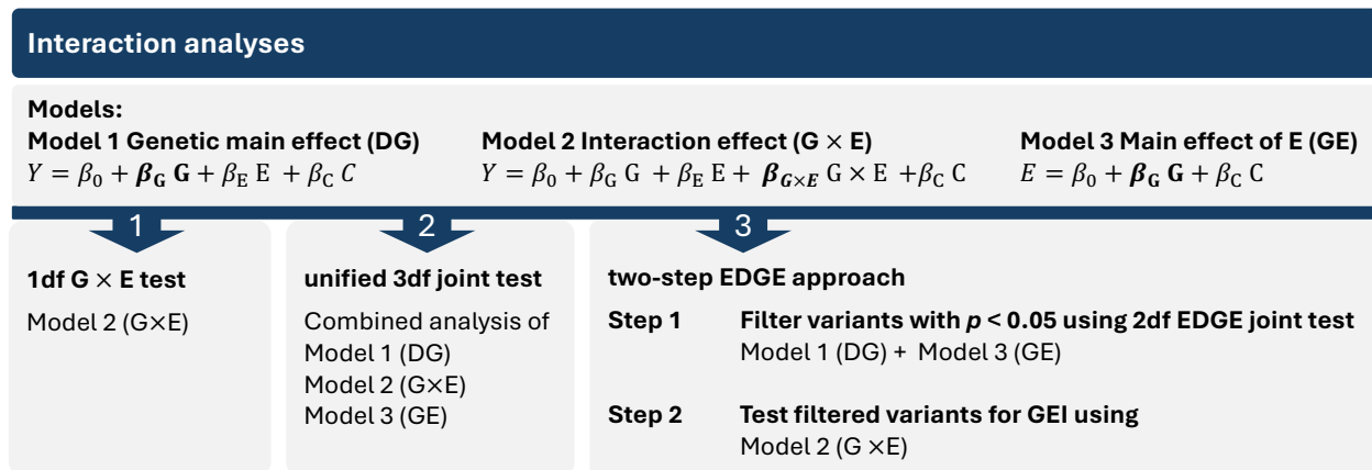
Figure 1 The three GEI analysis approaches used in this study.
