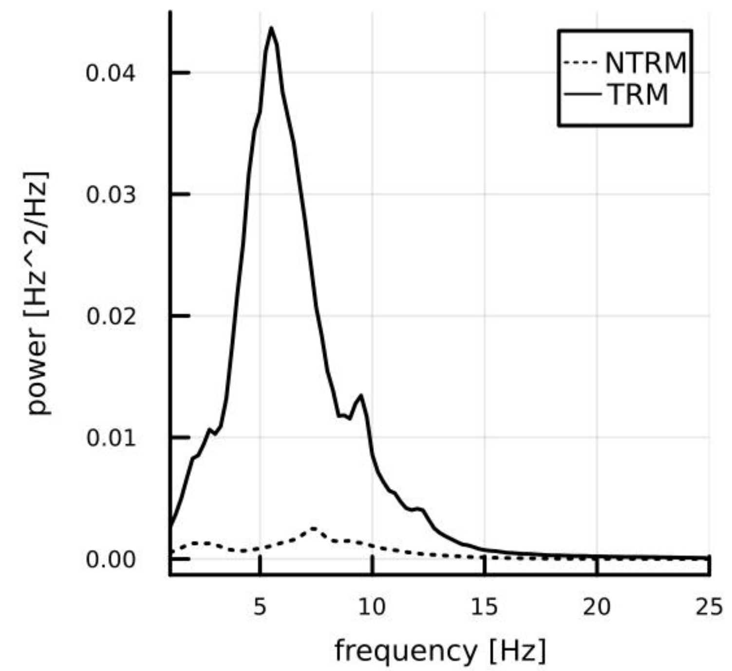
Angular velocity (Z)
