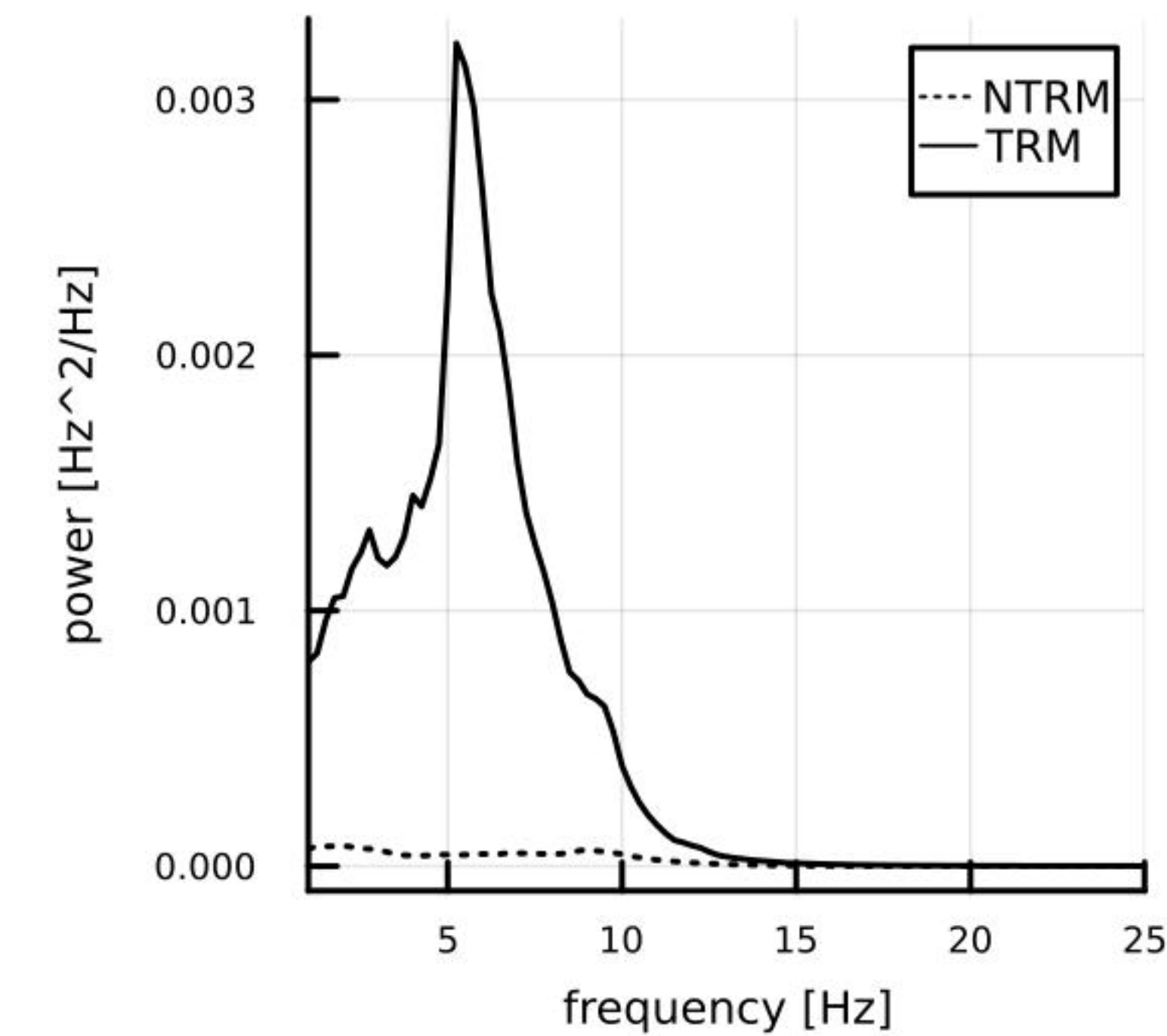
Angular velocity (X)
