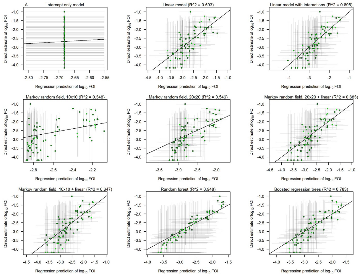
Figure S3. Scatterplots showing the relationship between the statistical regression predictions of FOI on the x-axis vs. the FOI estimates projected from LF case data and reporting probabilities for each of the eight statistical models (plus a null intercept-only model) included in our analysis. Plots are restricted to FOI estimates that were used in model fitting and do not include data held out for model validation. Results are for the 2 nd administrative level and a 6% seroreversion rate.
