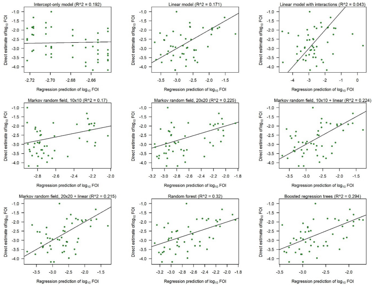
Figure S5. Scatterplots showing the cross-validation performance of each statistical regression model.
