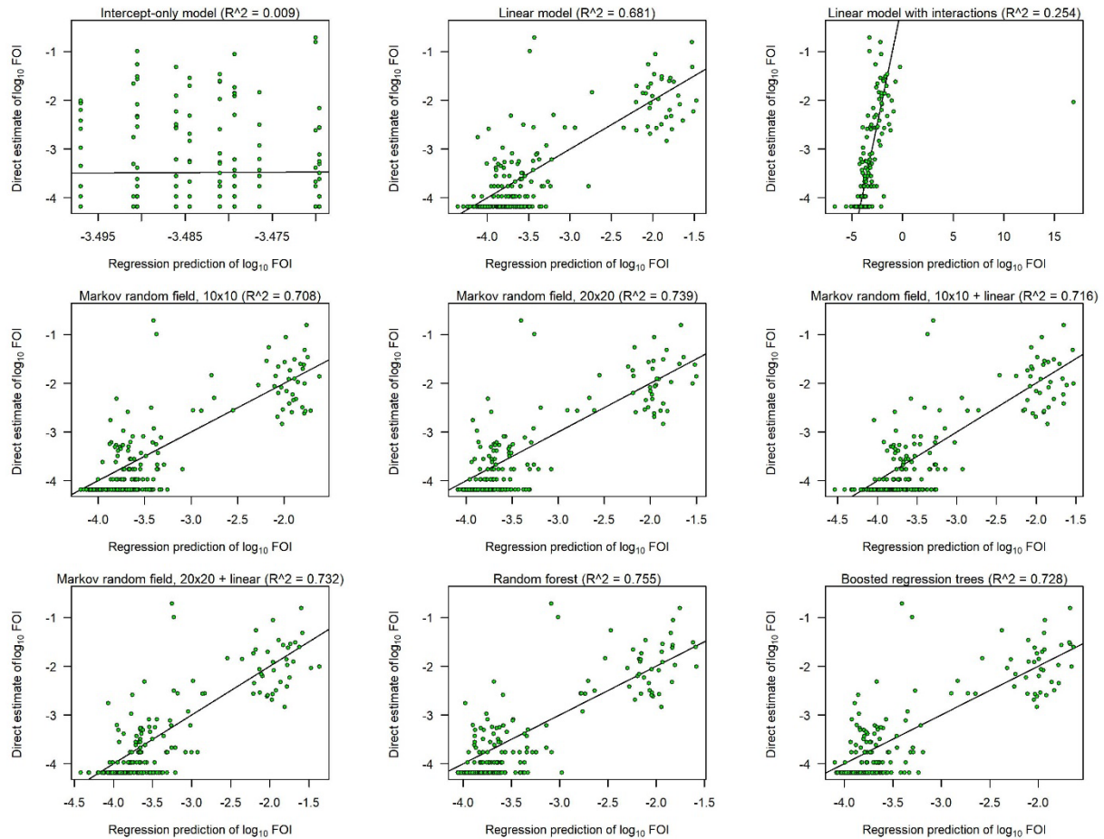
Figure S6. Scatterplots showing the cross-validation performance of each statistical regression model.
