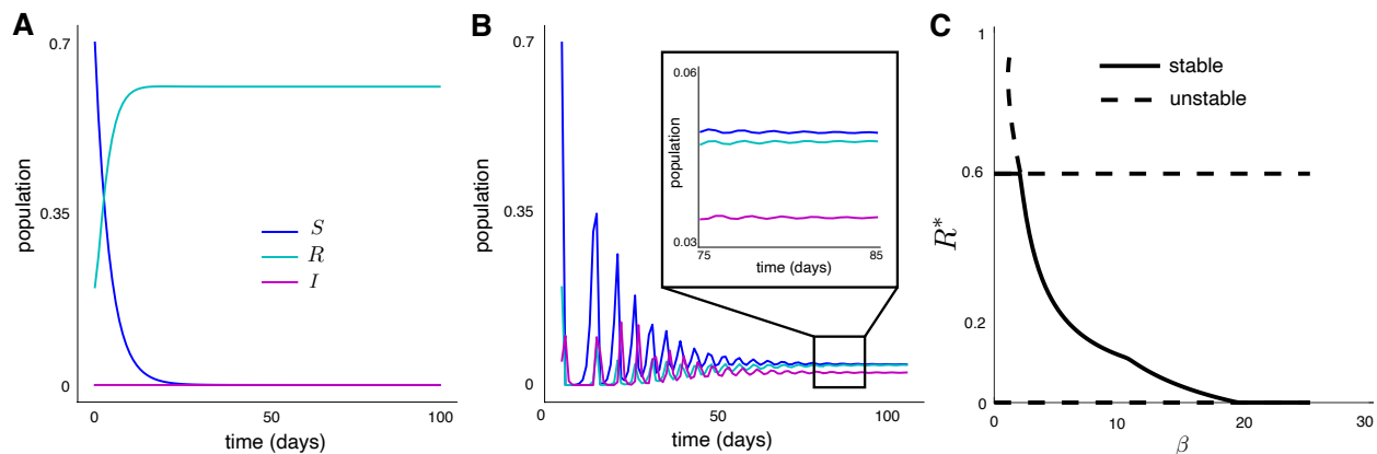
Figure 2: Simulation results of Eq. (1): (A) bacteria population in the absence of virus-infected bacteria \alpha = 0 , \beta = 0 and I(0) = 0 , (B) bacteria population in the presence of virus-infected bacteria \alpha = 0 , \beta = 15 and I(0) > 0 , and (C) a bifurcation diagram showing the impact of virus infectivity on equilibrium mutant population.
