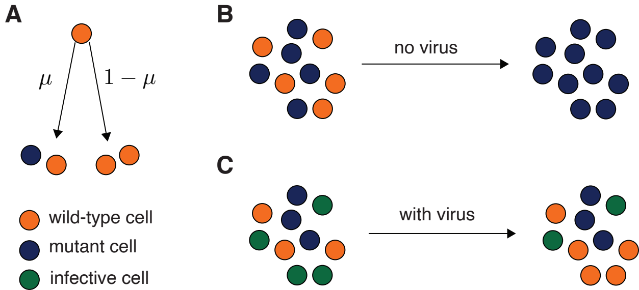
Figure 1: Schematic of our model. (A) Wild-type cells undergo fission and with a probability \mu produce mutants that are antibiotic-resistant. (B) If mutants arise, then they will eventually dominate the population. This is undesirable. (C) We hypothesize that adding viral infection promotes the ability for coexistence between the wild-type and mutant strains.
