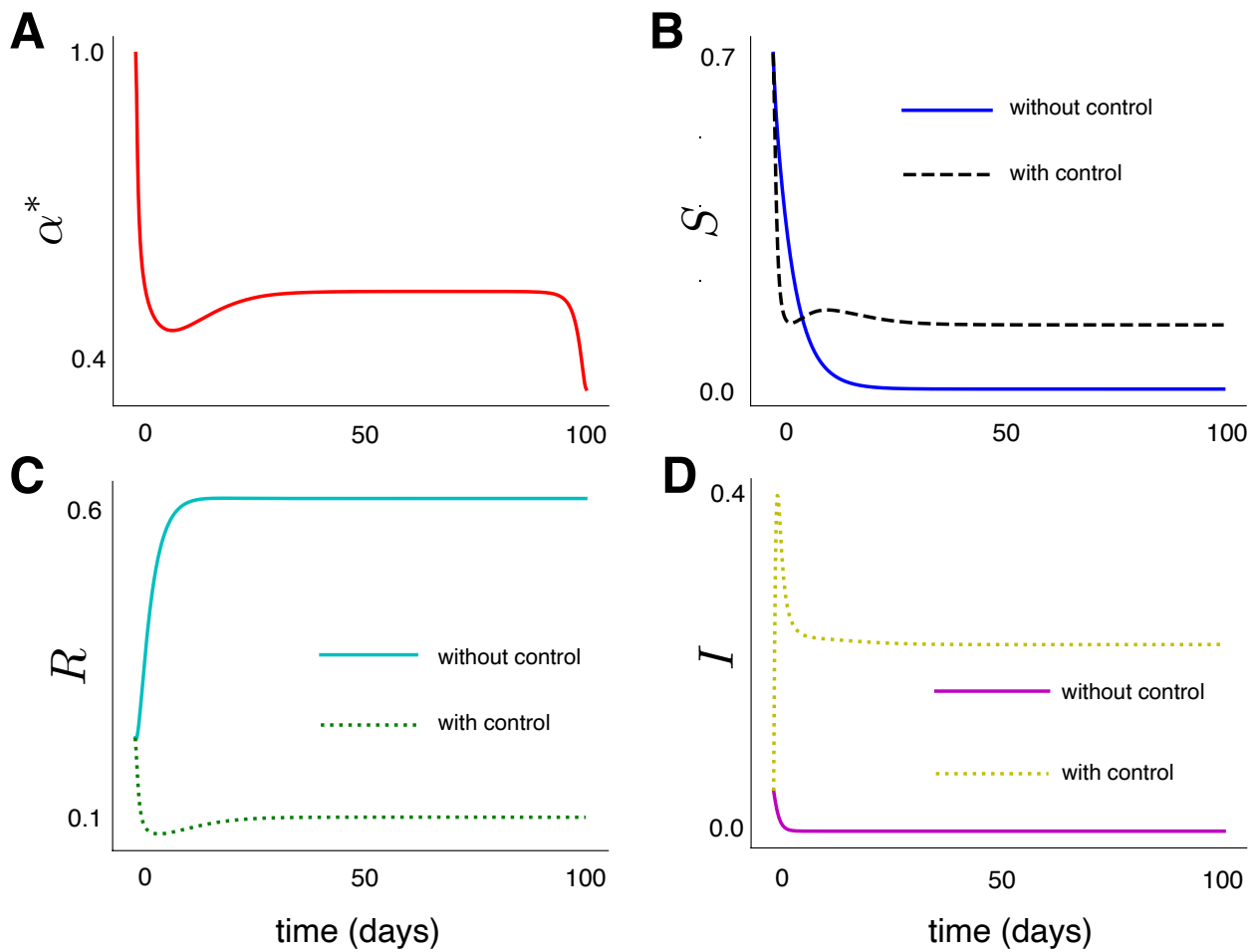
Figure 3: Simulation results of Eq. (1) with optimal control obtained from solving Eq. (4). (A) the optimal profile for the control variable \alpha , (B) the corresponding wild type bacteria population S , (C) the corresponding antibiotic-resistant bacteria population R , and (D) the corresponding virus infected bacteria population I .
