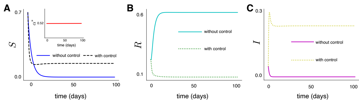
Figure 4: Simulation results from Eq. (1) with a constant virus infusion rate \hat{\alpha} as obtained from Eq. (6) (A) Wild type population in response to the constant control profile. Inset: the constant control profile. (B) Antibiotic-resistant bacteria population R and (C) Virus infected bacteria population I .
