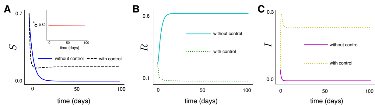
Figure 4: Simulation results from Eq. (1) with a constant virus infusion rate \hat{\alpha} as obtained from Eq. (6) (A) Wild type population in response to the constant control profile. Inset: the constant control profile. (B) Antibiotic-resistant bacteria population R and (C) Virus infected bacteria population I .
